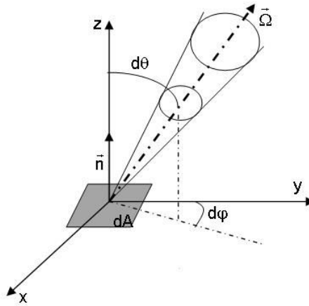
FIGURE 1.1 – Luminance monochromatique
