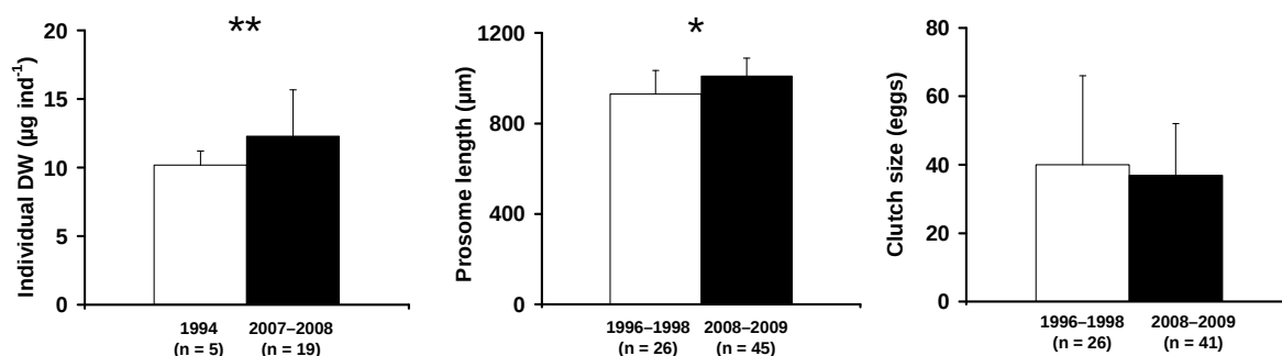
Fig. 1. Comparison of Eurytemora affinis ’ female individual dry weight (DW), prosome length and clutch size between two periods in the brackish water reach of the Scheldt estuary (Antwerpen). Mean values are given with their standard deviations. n for DW correspond to the number of treated samples, n for prosome length and clutch size correspond to the number of copepods analysed. Mann–Whitney tests significance levels are indicated (*: p < 0.05 ; **: p < 0.01 ).
