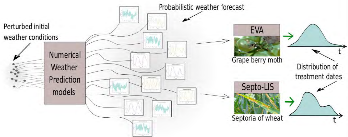
Figure 3: Ensemble prediction and propagation of weather forecast uncertainties through the both cases wheat septoria and grape berry moth.
