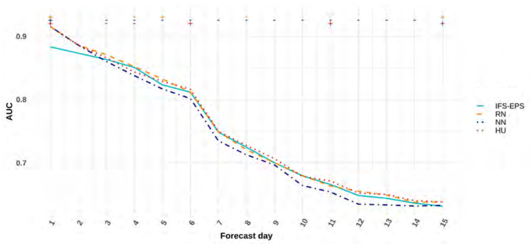
FIG. 8. AUC of 2-meter temperature forecasts above 15°C, computed for the 11 sites over the period 01/06/2018-31/05/2019, as a function of forecast day. Results for the random 12-member IFS-EPS and the three seamless ensembles are overlaid. Top + (resp. -) signs indicate that the performance of a seamless ensemble is statistically better (resp. worse) than the IFS-EPS performance, according to the Wilcoxon test.
