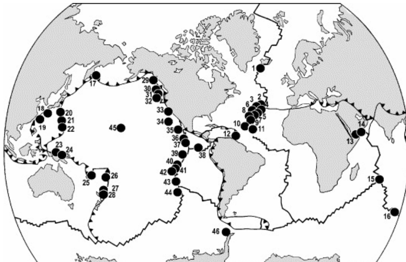
Figure I.10 : Positions géographiques des zones hydrothermales connues (à des profondeurs >200 m) présentant une faune associée : 1 — Steinhall, 2 — Menez Gwen, 3 — Lucky Strike, 4 — Mount Saldanha, 5 — Rainbow, 6 — Lost City, 7 — Broken Spur, 8 — TAG, 9 — Snake Pit, 10 — Logatchev, 11 — Ashadze, 12 — Kick'em Jenny Volcano, Grenada, 13 — Gulf of Aden, 14 — Tadjoura Rift, 15 — Rodryges Triple Junction (Kairei and Edmond Fields), 16 — Amsterdam — St. Paul Plateau, 17 — Piip's Volcano, 18 — Okinawa trough (Fields Minami-Ensei Knoll, Iheya Ridge, Izena Caldron, Hatoma Knoll), 19 — Daiyon Knoll, 20 — Ogasawara North (Fields Myojin Knoll, Sumisi Caldera, Seamounts Suiyo, Moknyo and Kaikata), 21 — Ogasawara South (Nikko Seamount), 22 — Mariana Trough, North and South (Fields Daini Kasuga Seamount, Central Mariana Trough, South Mariana Ridge), 23 — Manus Basin, 24 — Edison Seamount, 25 — North Fiji Basin, 26 — Lau Basin, 27–28 — Kermadec Ridge (Fields Rumble III and Rumble V, Brothers Caldera and Macauley Cone), 29 — Explorer Ridge, 30 — Juan de Fuca, 31–32 — Gorda Ridge, 33 — Guaymas Basin, 34 — EPR 21°N, 35 — EPR 13°N, 36 — EPR 11°N, 37 — EPR 9°N, 38 — Galapagos Rift, 39 — EPR 7°S, 40 — EPR 17°, 40 — 21°S, 42 — EPR 23°S (and Pito Seamount, Easter Microplate), 43 — EPR 27–32°S, 44 — Pacific-Antarctic Ridge 37°S, 45 — Loihi Seamount, 46 — Hook Ridge, Bransfield Strait. (Tarasov et al. , 2005).
