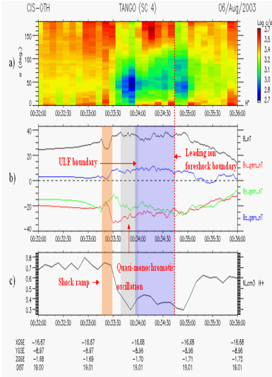
Fig.4.11 A snapshot of magnetic field measurements with 1s time resolution and proton density in the cavity from C4, where the ion measurements are from CODIF sensor. The red, gray and blue shadows denote respectively the time intervals of the shock ramp, ULF waves, and the backstreaming field-aligned beam.
