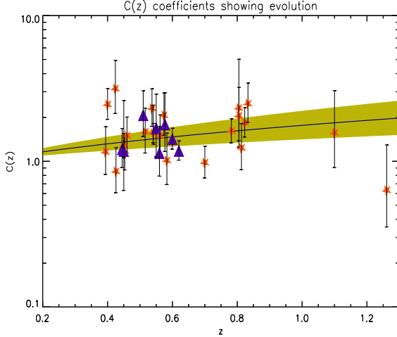
Fig. 1. XMM and Chandra measurements of the evolution of clusters L – T relation expressed by the C(z) coefficient (Eq. 3). Stars are Chandra data while triangles are our XMM data and error bars are derived from the 1\sigma error on the temperature measurement. Grey area represents the 1\sigma error on the C(z) fit.
