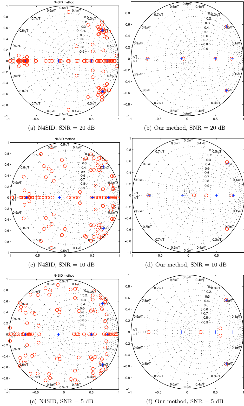
Figure 3.4: The effect of SNR.
