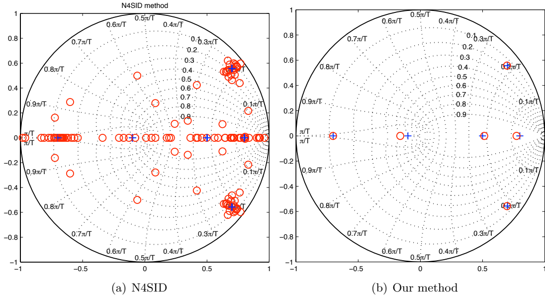
Figure 3.3: The inputs are sum of sinusoidal signals.
