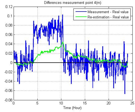
Figure 15: Scenario 2. State estimation error at sensor location
