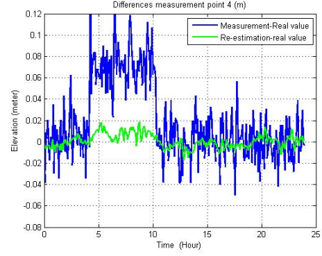
Figure 7: Scenario 2. State estimation error at sensor location
