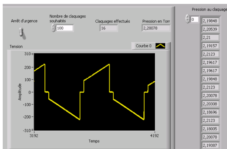
Figure.III. 6. Interface graphique (Labview 7.1).
