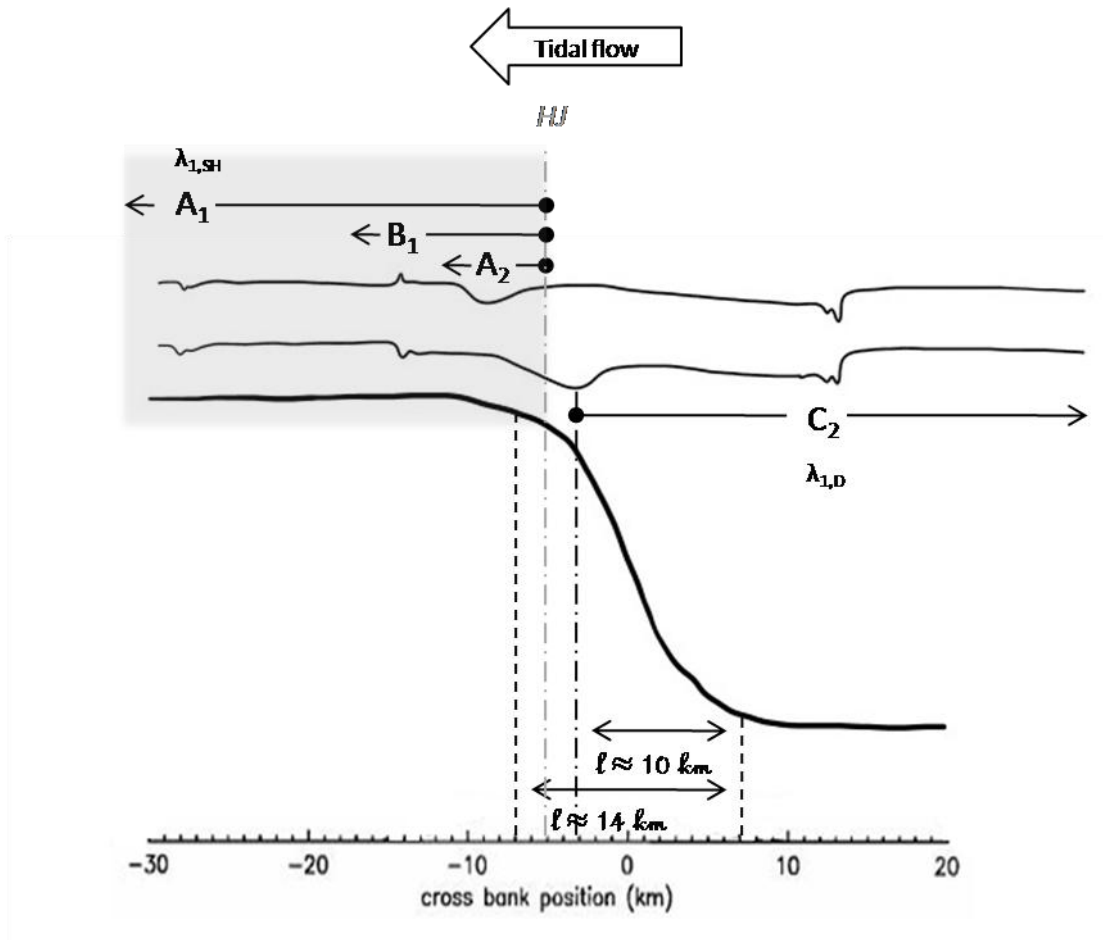
FIGURE 3 - Schematic of internal wave dynamic above Georges Bank
