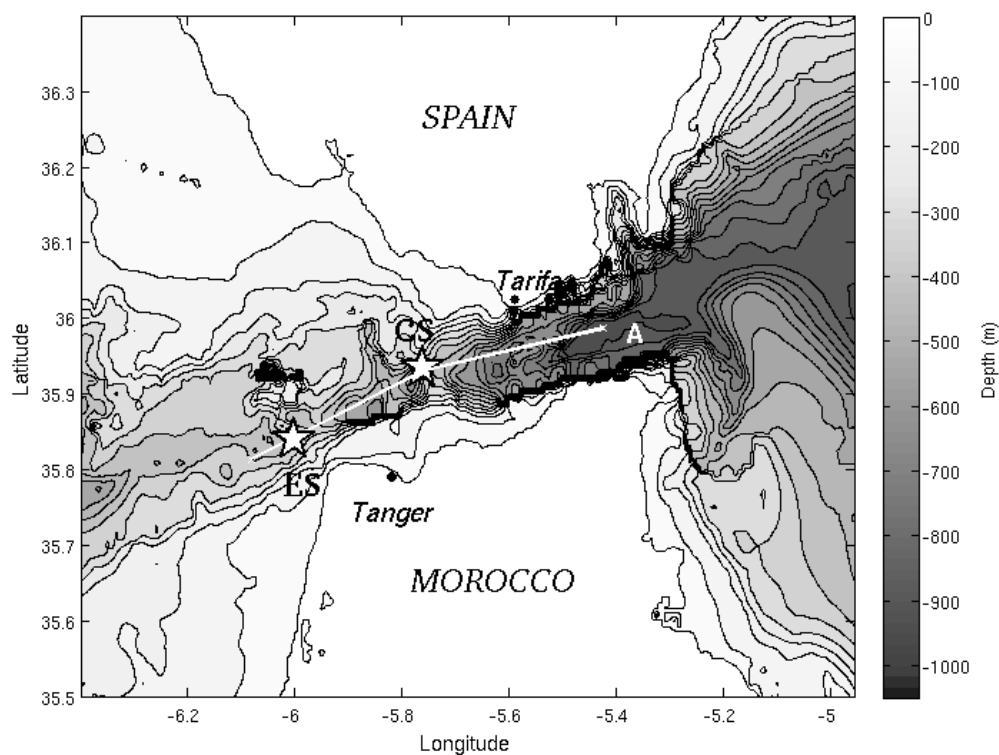
FIGURE 4 – Bathymetry of the strait of Gibraltar, location of the transect A used in SimGBR0 and location of Camarinal Sill (CS), Espartel Sill (ES)
