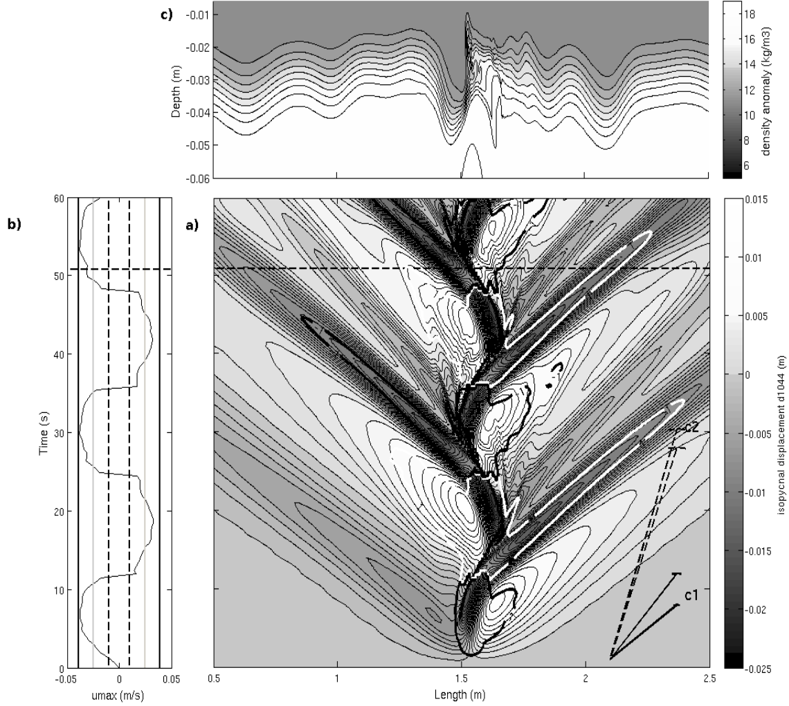
FIGURE 11 –a) Space-time diagram of the isopycnal displacement d_{1044} for \rho=1044 kg/m 3 (located at the top of the pycnocline) in Sim4 . Arrows indicate the speed of the two fastest normal modes calculated with modal decomposition method ( c_1= 0.039 m/s, c_2= 0.01 m/s). Black and white contour lines locate hydraulic control of the second vertical mode.
