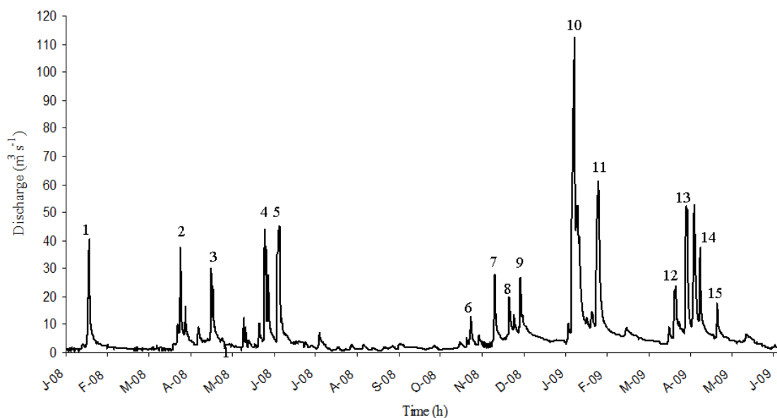
Figure 5-2: Hourly discharge in the 15 flood events observed during the study period (January 2008 to June 2009) at Larra sampling station.
