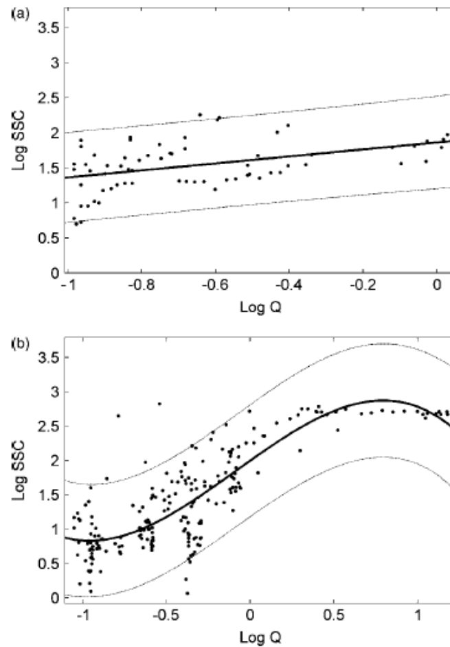
Figure 2-9: Catchment seasonal rating curves showing long discharge (Q) and log suspended sediment concentrations (SSC) with 95% confidence intervals for (a) summer-autumn and (b) winter-spring period (From Smith 2008)
