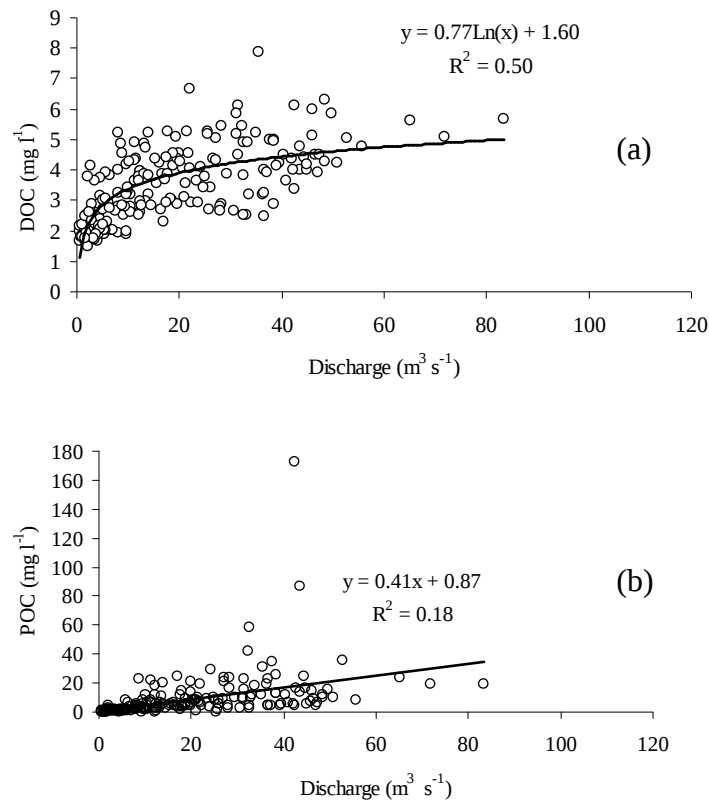
Figure 5-5. Relationship between discharge and DOC (a) and POC (b).
