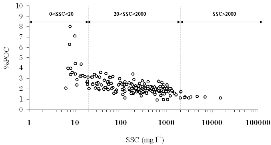
Figure 5-4. Relationship between POC contents (% of dry weight) and suspended sediment concentrations ( \text{mg l}^{-1} ) from the Save catchment at Larra sampling station
