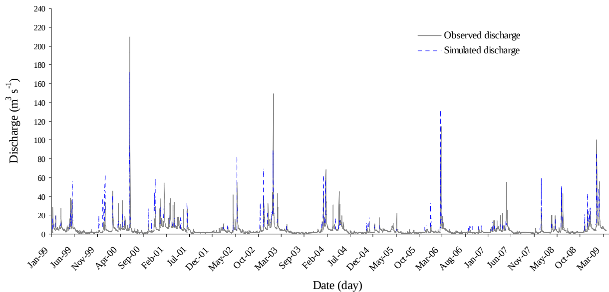
Figure 6-4. Observed and simulated daily discharge at Larra station (January 1999 to March 2009).
