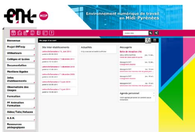
Illustration 2: interface Entmip
