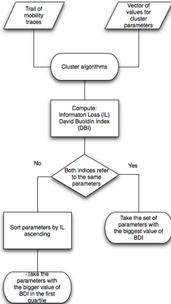
Figure 2.6: Flux diagram representing the method for choosing the optimal parameters of the clustering algorithm.
