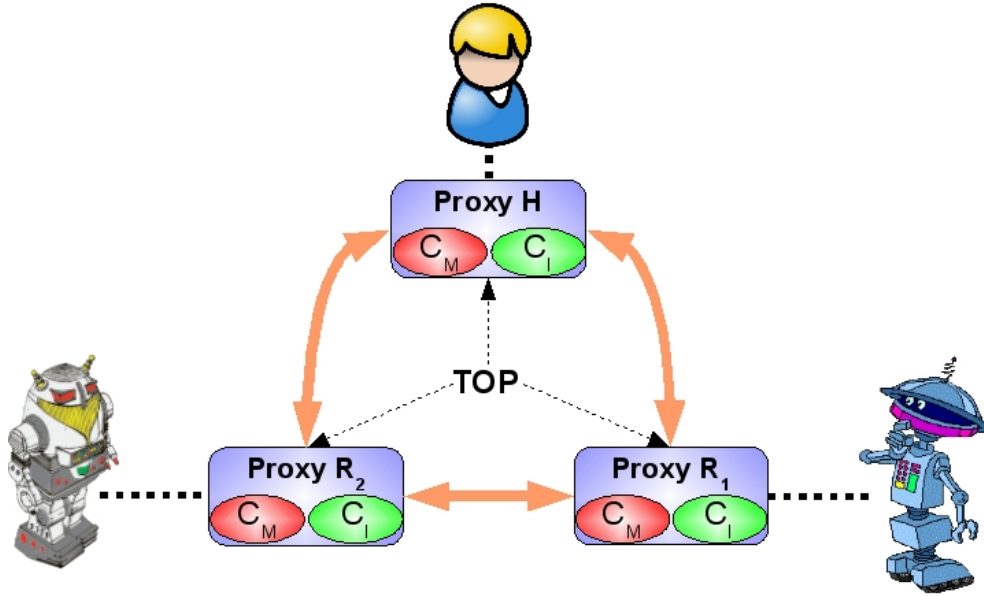
FIG. 1.5 – Structure d’une application STEAM.
