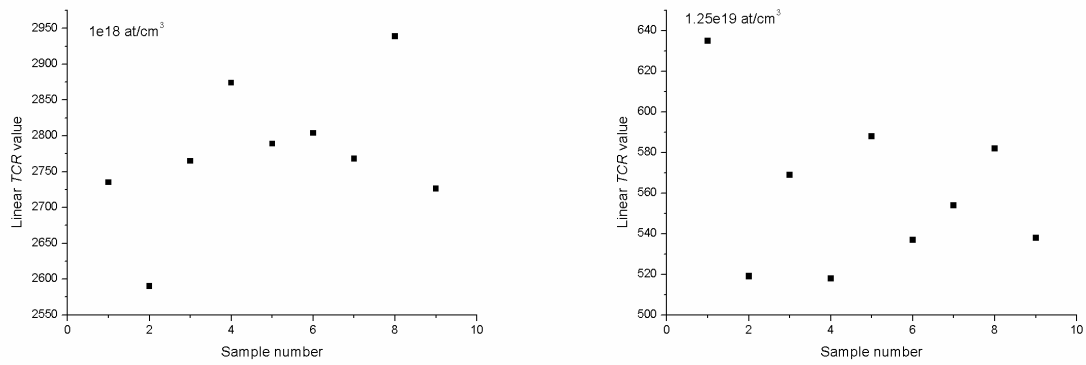
Fig. 4.29 Measured linear TCR values for two different doping profiles with the surface concentration of about 10^{18} at/cm 3 (left) and 1.25 \cdot 10^{19} at/cm 3 (right).
