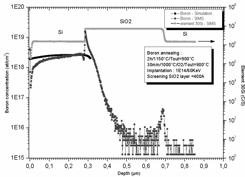
Fig. 4.34 Simulation of the dopants distribution for the implanted dose of 10^{14} at/cm 3 and corresponding SIMS analysis.
