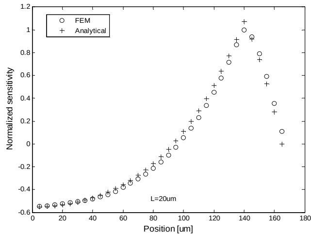
Fig. 2.43 c) Comparison of the normalized sensitivity value obtained by two different methodologies. Results are traced in the function of the gauge position on the membrane and the gauge length 20\mu\text{m} .
