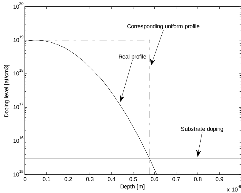
Fig. 2.28 The real Gaussian profile used for gauge parameters calculations and the corresponding uniform profile.
