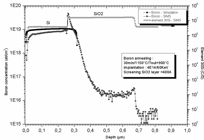
Fig. 4.38 Simulation and SIMS profile of the dopants distribution for the implanted dose of 4 \cdot 10^{14} at/cm 3 .
