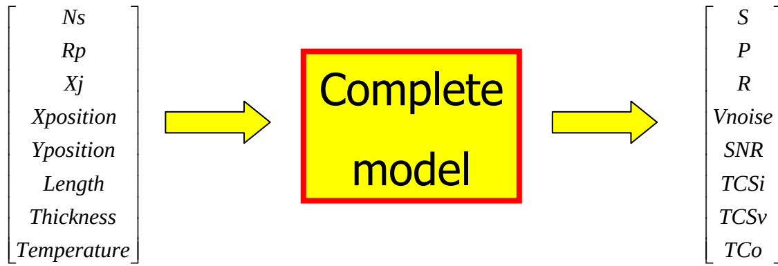
Fig. 3.5 The compact model of the piezoresistive pressure sensor.
