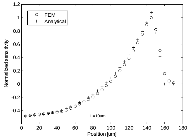
Fig. 2.43 b) Comparison of the normalized sensitivity value obtained by two different methodologies. Results are traced in the function of the gauge position on the membrane and the gauge length 10\mu\text{m} .
