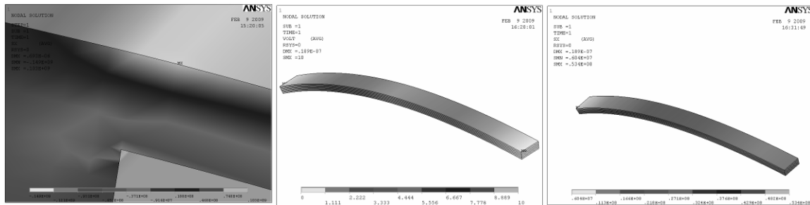
Fig. 2.39 Clamping zone of the membrane where the gauge is placed (left) the electrical potential distribution (centre) and the uniaxial stress value (right) in a gauge that was sub modeled.
