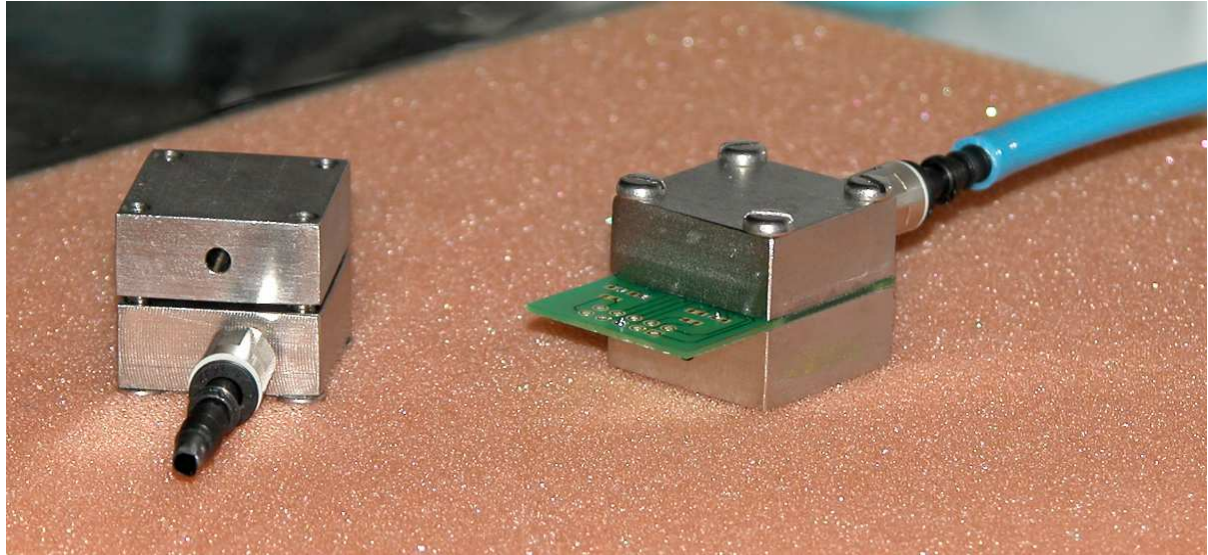
Fig. 4.12 The real view of the experimental setup.
