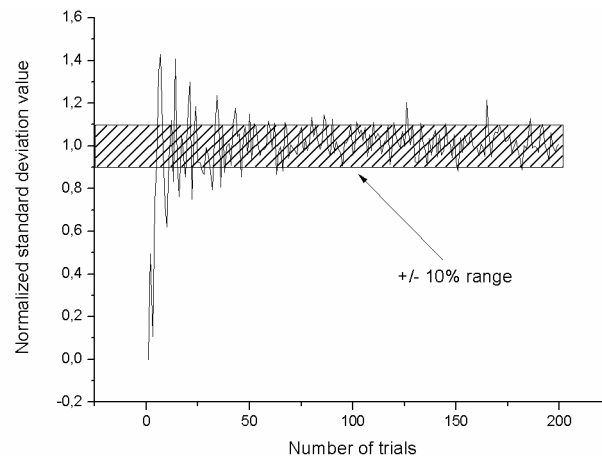
Fig. 3.11 The standard deviation value in function of the number of trials.
