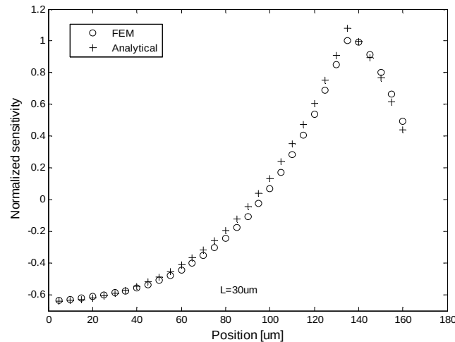
Fig. 2.43 d) Comparison of the normalized sensitivity value obtained by two different methodologies. Results are traced in the function of the gauge position on the membrane and the gauge length 30μm.
