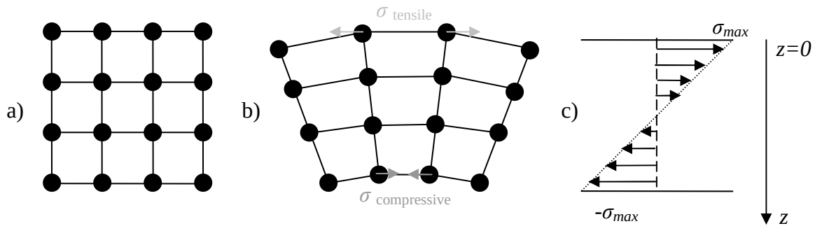
Fig. 2.11 The simplified model of the unloaded structure a), bended structure with compressive and tensile stresses b), model of stress distribution along the membrane thickness c).
