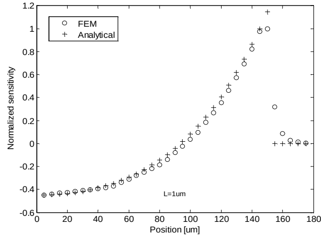
Fig. 2.43 a) Comparison of the normalized sensitivity value obtained by two different methodologies. Results are traced in the function of the gauge position on the membrane and the gauge length 1\mu\text{m} .
