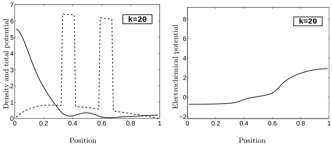
Figure I.3: Numerical solution of the QDD model, after 20 iterations. The same quantities as on Fig. I.1 are represented.
