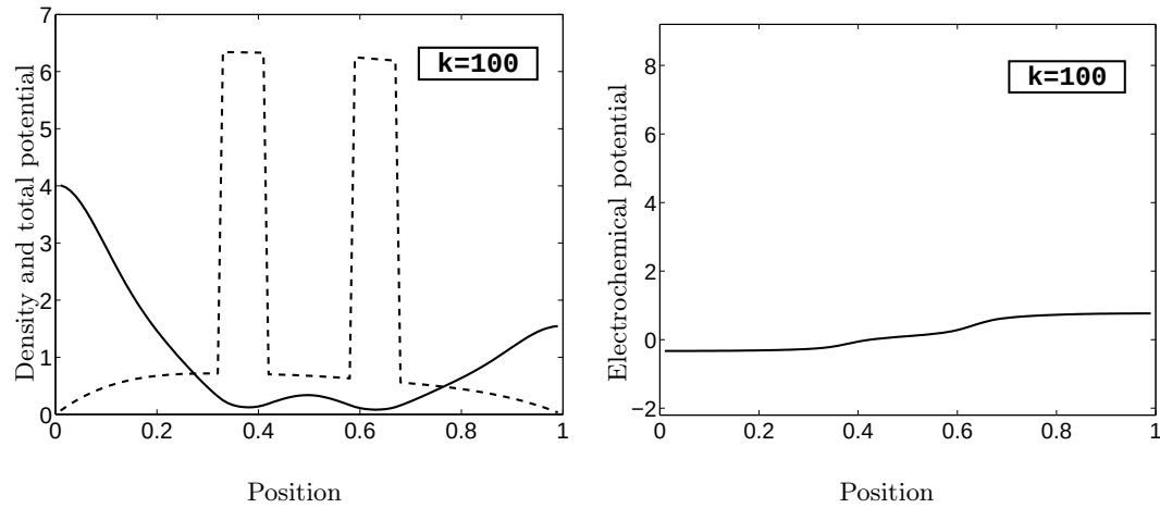
Figure I.4: Numerical solution of the QDD model, after 100 iterations. The same quantities as on Fig. I.1 are represented.
