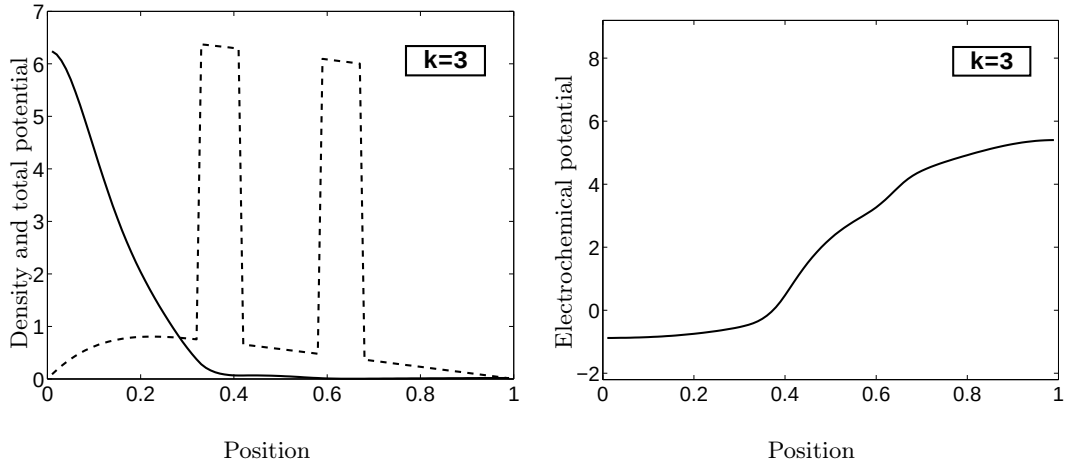
Figure I.2: Numerical solution of the QDD model, after 3 iterations. The same quantities as on Fig. I.1 are represented.
