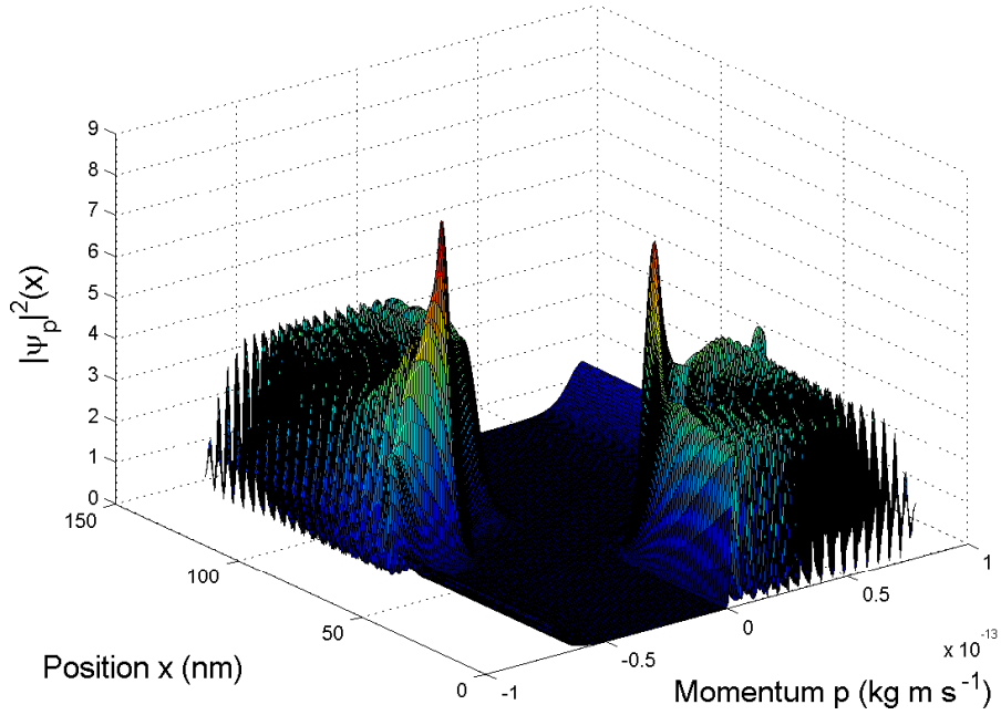
Figure III.9: Square norm of the generalized eigenfunctions \psi_p(x) for the first test case (single barrier) for an applied bias of 0.05V : we can see there is no resonance meaning the momentum p can be discretized with a big step size.
