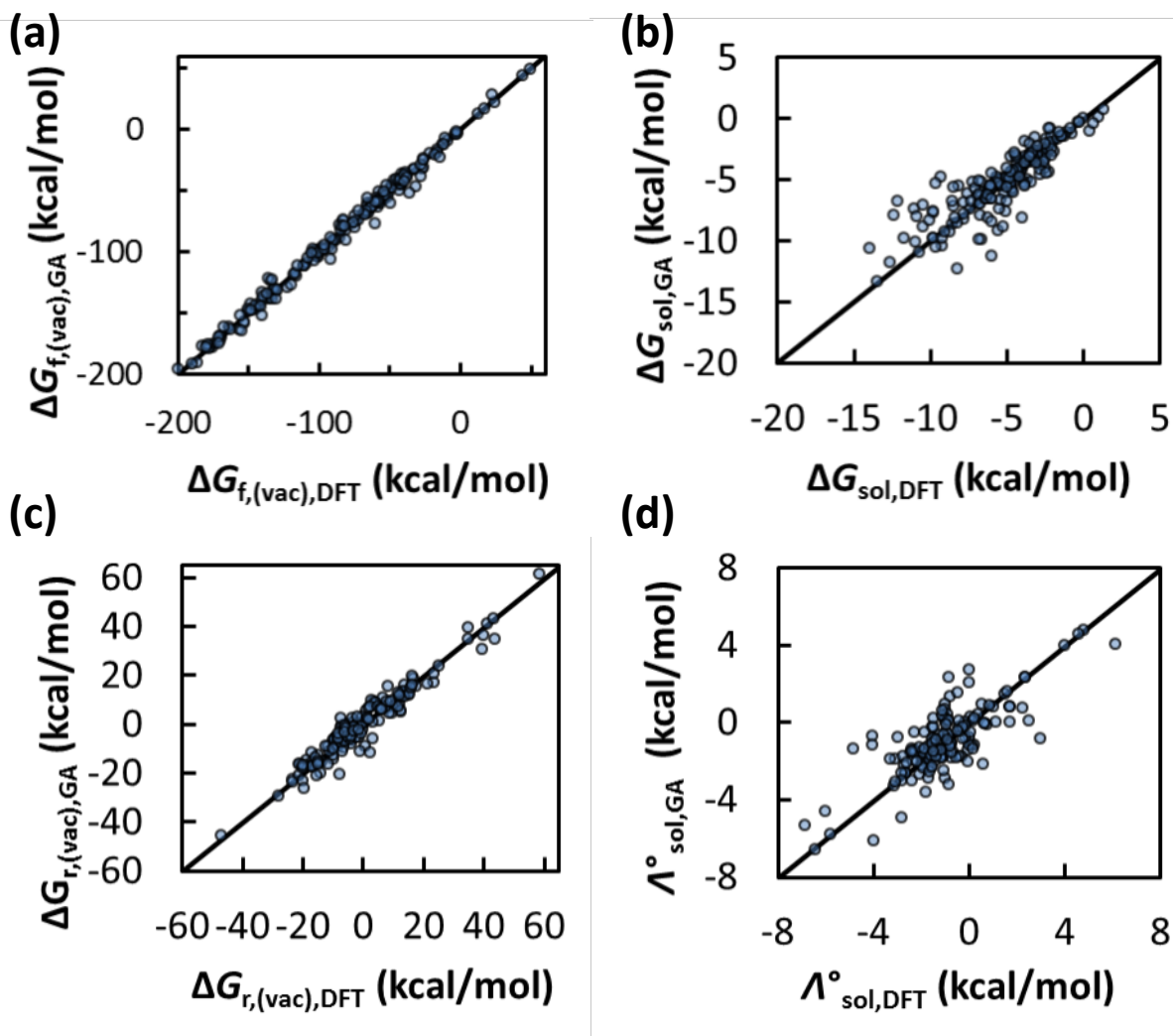
Figure 4. Parity plot between 10-fold cross-validation computed prediction and DFT data for (a) Gibbs free energy of formation, \Delta G_{f,\text{(gp)}} , (b) Gibbs free energy of solvation, \Delta G_{\text{sol}} , (c) Gibbs free energy of reaction, \Delta G_{r,\text{(vac)}} , and (d) the change of reaction energies upon solvation, \Delta_{\text{sol}} , as defined in Eq.(14) and (15). 151 reactions of the ethanol reaction network are considered (see SI for the detail).
