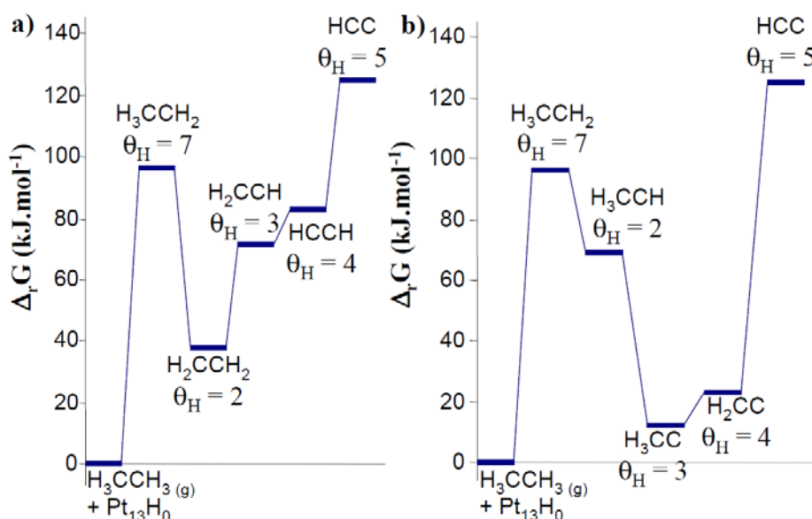
Figure 20 – \Delta_r G of the most stable configuration of C_xH_y species on the Pt_{13}H_n/\gamma-Al_2O_3 model (including H coverage optimization) relative to the a) symmetric b) asymmetric dehydrogenation pathways for the low J ratio ( J = 0.01 ) at 800 K.
