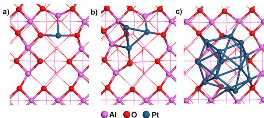
Figure 3 – Top views of the most stable adsorption geometries for \text{Pt}_n clusters on the (100) dehydrated surface of \gamma -alumina with a) n = 1 , b) n = 3 and c) n = 13
