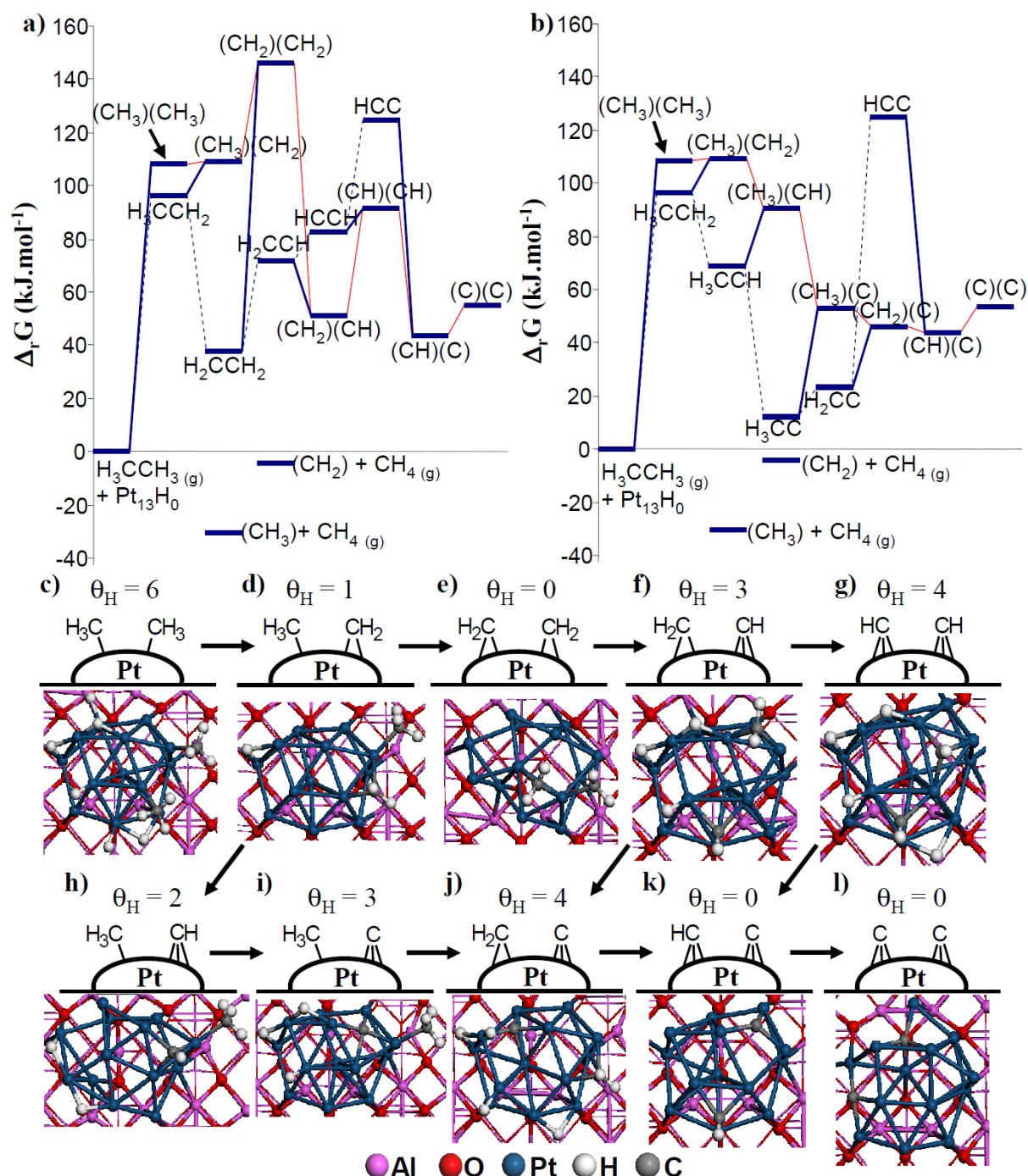
Figure 21 – a-b) Evolution of \Delta_r G value of the most stable configuration of C_xH_y intermediates issued from C-H plus C-C bond breaking on the Pt_{13}H_n/\gamma-Al_2O_3 model (including H coverage variation) for the low J ratio ( J = 0.01 ). Parenthesizes delimit the monocarbonaceous species adsorbed on the cluster after the C-C bond breaking. a) the symmetric dehydrogenation and b) the asymmetric dehydrogenation. Plain blue lines correspond to C-C bond breaking reactions whereas dash blue lines are the reaction paths of a) the symmetric and b) the asymmetric dehydrogenation reactions. Red lines represent the dehydrogenation reaction path after the C-C bond breaking. c) to l) : most stable structures where the C-C bond was broken.
