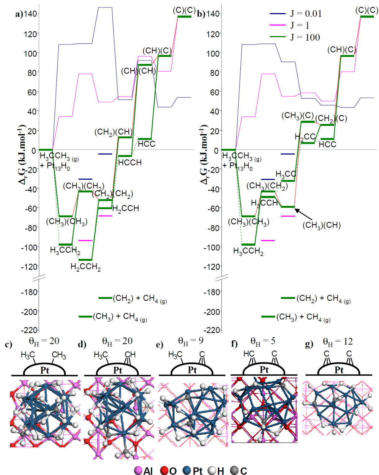
Figure 27 – \Delta_r G of the C-C bond breaking intermediates on the Pt_{13}H_n/\gamma\text{-Al}_2\text{O}_3 model for the J = 0.01 , J = 1 and J = 100 . (including H coverage variation) following a) the symmetric dehydrogenation and b) the asymmetric dehydrogenation pathways. Parenthesizes delimit the monocarbonaceous species adsorbed on the cluster after the C-C bond breaking. Plain green lines correspond to C-C bond breaking reactions whereas dash green lines are the reaction paths of a) the symmetric and b) the asymmetric dehydrogenation reactions. Red lines represent the dehydrogenation reaction path after the C-C bond breaking. c-f) selected optimized structures.
