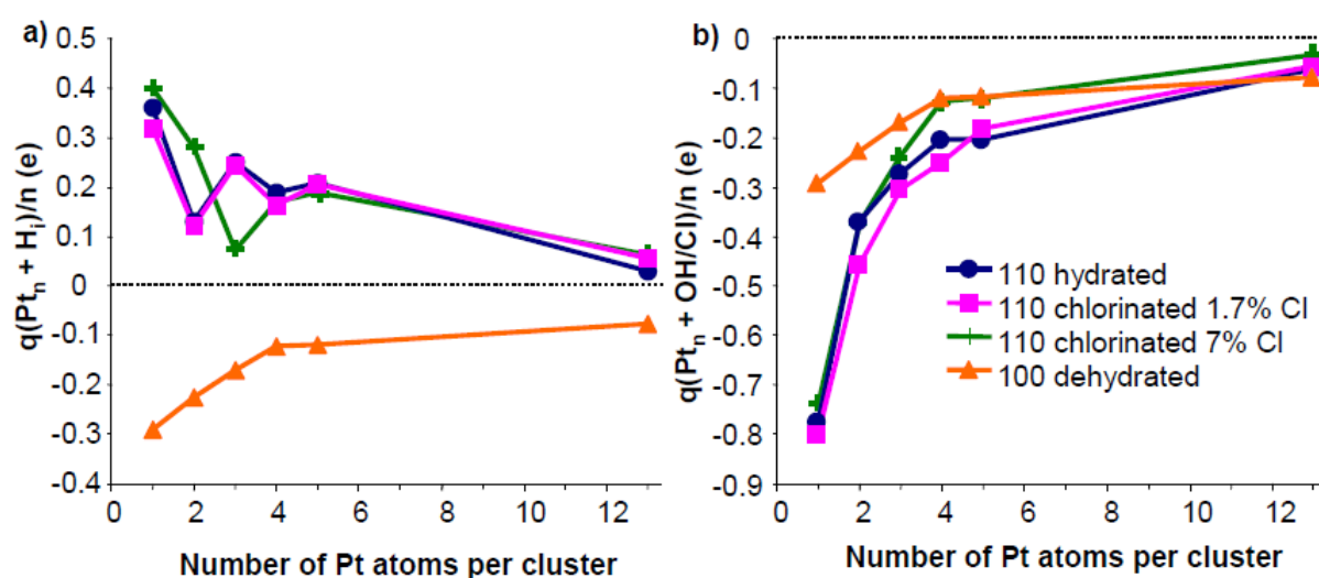
Figure 15 - Bader charge analysis of the supported ( \text{Pt}_n + migrated species) fragment normalized by the number of Pt atoms (mean charge per Pt atom) with migration of a) H atoms, b) OH or Cl species. OH migration are considered for the hydrated surface and Cl migration for the chlorinated ones. The (100) surface is recalled for comparison even if no migration obviously occurs.
