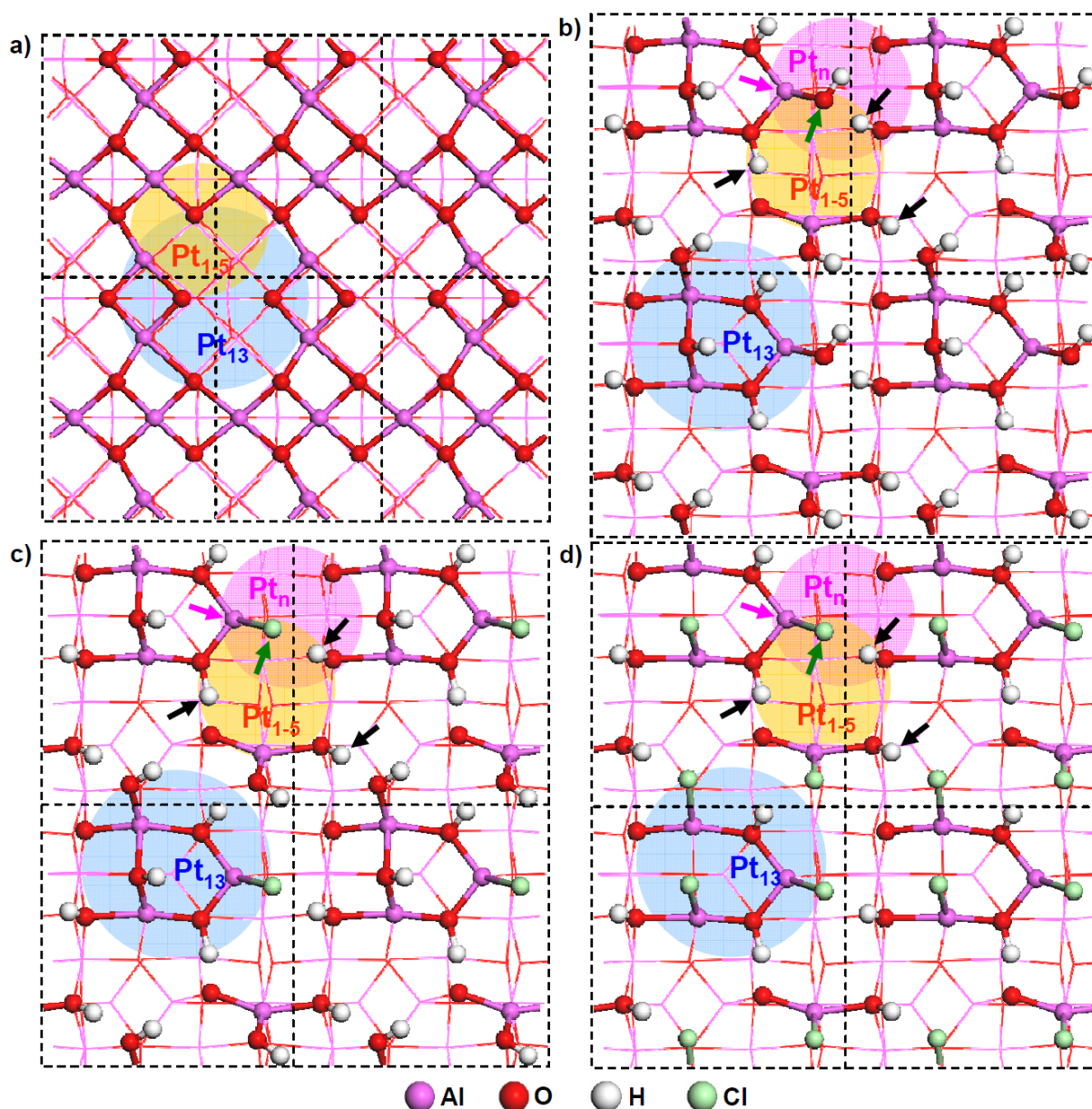
Figure 1 – Top views of the \gamma -Al 2 O 3 supercell models of a) dehydrated (100) surface, b) hydrated (110) surface, c) slightly chlorinated (110) surface (1.5 Cl.nm -2 ) and d) highly chlorinated surface (5.9 Cl.nm -2 ). Relevant adsorption sites of Pt n clusters: Pt 1-5 without migration in orange disks, Pt 13 without migration in blue disks, Pt n with migration in pink disks. Relevant surface species involved in migration are marked with arrows (black: H atoms from surface hydroxyl groups, green: hydroxyl or chlorine group). Pink arrows mark the Al III atom on the (110) surfaces. Dashed black lines delimit the irreducible unit cells while calculations are performed on (3x2) and (2x2) supercells respectively for the (100) and the (110) surfaces.
