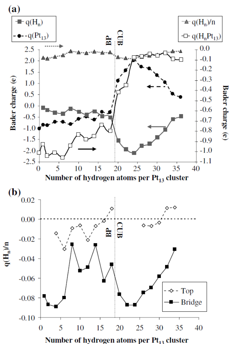
Figure 6. (a) Bader charge analysis of the \text{H}_n (total charge and mean charge per H atom), \text{Pt}_{13} and \text{Pt}_{13}\text{-H}_n subsystems. (b) Mean Bader charge per H atoms of the \text{H}_n subsystem for top and bridge sites. All data are drawn for the most stable cluster geometry for a given n value (the BP-CUB transition is represented by the dotted line).
