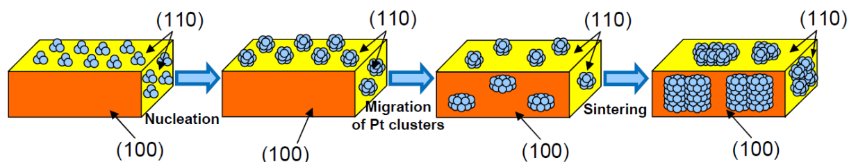
Figure 14 - Illustration of the nucleation process on tablet of \gamma\text{-Al}_2\text{O}_3 . At first, Pt clusters are stored on the (110) surface in the form of Pt_3 clusters. Sintering induced by thermal conditions increases the cluster size up to Pt_{13} . Its stability on chlorinated (110) surface is close to the on dehydrated (100). The migration of Pt_{13} clusters to the (100) surface can thus be considered to explain the high reactivity of the catalyst on both surfaces.
