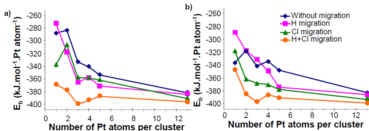
Figure 9 - Binding energies of \text{Pt}_n clusters as a function of cluster size including migration phenomena on a) a slightly chlorinated (110) \gamma\text{-Al}_2\text{O}_3 surface ( 1.5 \text{ Cl.nm}^{-2} ) and b) a highly chlorinated (110) \gamma\text{-Al}_2\text{O}_3 surface ( 5.9 \text{ Cl.nm}^{-2} ).
