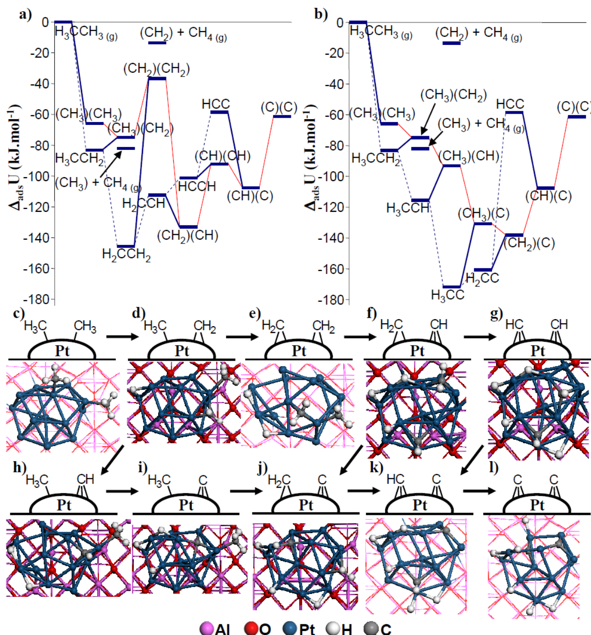
Figure 19 – a) b) Evolution of the adsorption energy for the intermediates issued from C-H plus C-C bond breaking on the Pt_{13}H_6/\gamma\text{-Al}_2O_3 model. Parenthesizes delimit the monocarbonaceous species adsorbed on the cluster after the C-C bond breaking following a) the symmetric dehydrogenation and b) the asymmetric dehydrogenation. Plain blue lines correspond to C-C bond breaking reactions whereas dashed blue lines are the reaction paths of a) the symmetric and b) the asymmetric dehydrogenation reactions. Red lines represent the dehydrogenation reaction paths after the C-C bond breaking. c) to l) : most stable structures where the C-C bond was broken.
