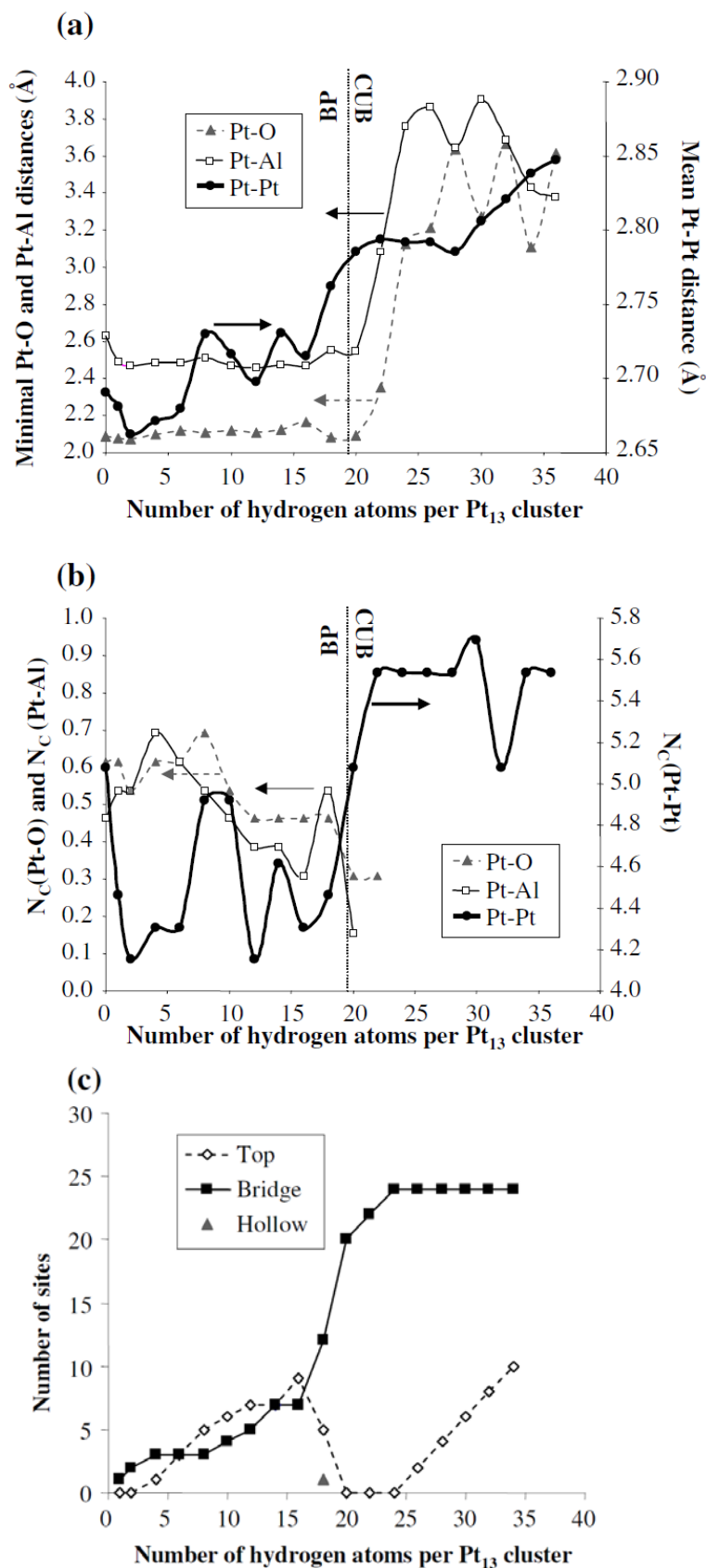
Figure 5. (a) Mean Pt-Pt distances (over Pt-Pt distances \leq 3 Å), and minimal Pt-O and Pt-Al distances for Pt_{13}-H_n on \gamma-Al_2O_3 (100). (b) Average Pt coordination numbers (for Pt-X distances \leq 3 Å). (c) Number of top, bridge and hollow occupied sites. All data are drawn for the most stable cluster geometry for a given n value (the BP-CUB transition is represented by the dotted line).
