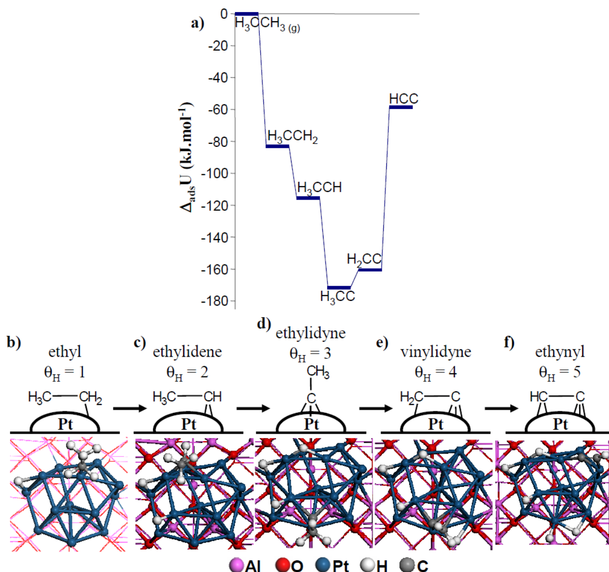
Figure 18 - Asymmetric dehydrogenation C_xH_y intermediates on Pt_{13}H_{6-y}/\gamma-Al_2O_3 model. a) \Delta_{ads}U for the most stable configurations depicted in figures b) to f).
