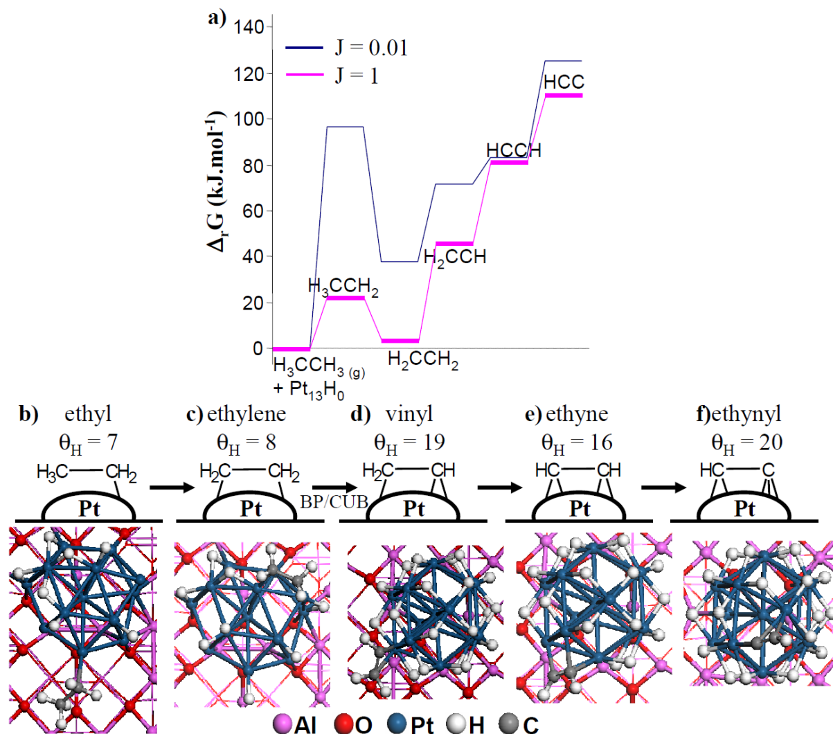
Figure 22 – a) \Delta_r G of the most stable configuration of C_xH_y species on the Pt_{13}H_n/\gamma\text{-Al}_2\text{O}_3 model (including H coverage optimization) relative to the symmetric dehydrogenation pathways for the medium J ratio ( J = 1 ). The results for the low J ratio ( J = 0.01 ) described in Figure 20a are recalled in blue. b) to f) Most stable structures found for J = 1 .
