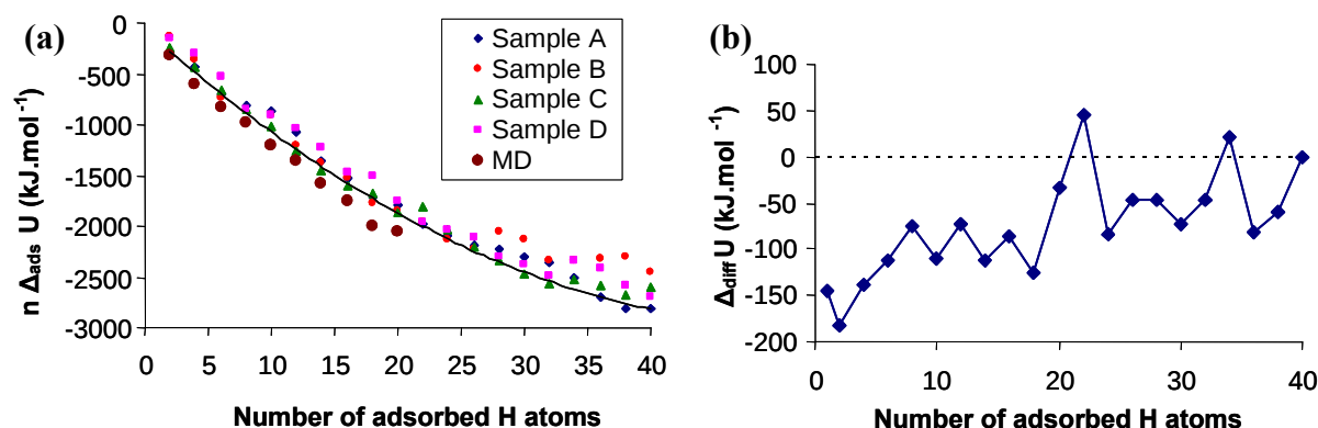
Figure S3.1: (a) Evolution of the adsorption energy of H 2 ( n\Delta_{\text{ads}}U ) as a function of the number of hydrogen atoms adsorbed on Pt 13 cluster for the BP morphology. Samples A, B, C and D were obtained by a static study and MD result from molecular dynamics approach. (b) Evolution of the differential adsorption energy as function of the number of H atoms adsorbed on Pt 13 cluster for the BP morphology (for the most stable configurations found at a given H coverage). The positive value observed for 22 H atoms adsorbed comes from the fact that the 22 H system was not refined by MD simulation.
