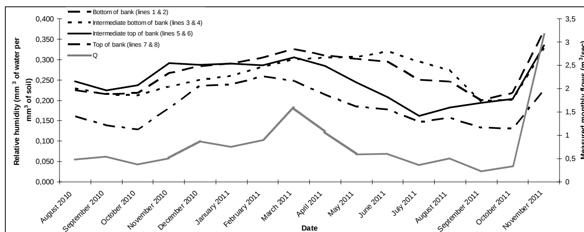
Fig. 1: Drought monitoring for the in situ experiment. In grey the monthly discharge at Pont de Bayeux, in black the in situ humidity sensors
