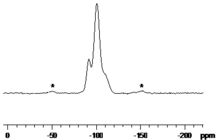
Figure III.S2. CP MAS ^{29}\text{Si} NMR of SBA-15. * denotes for spinning side bands.
