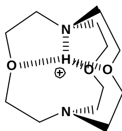
H + @Cryptand [1,1,1]
