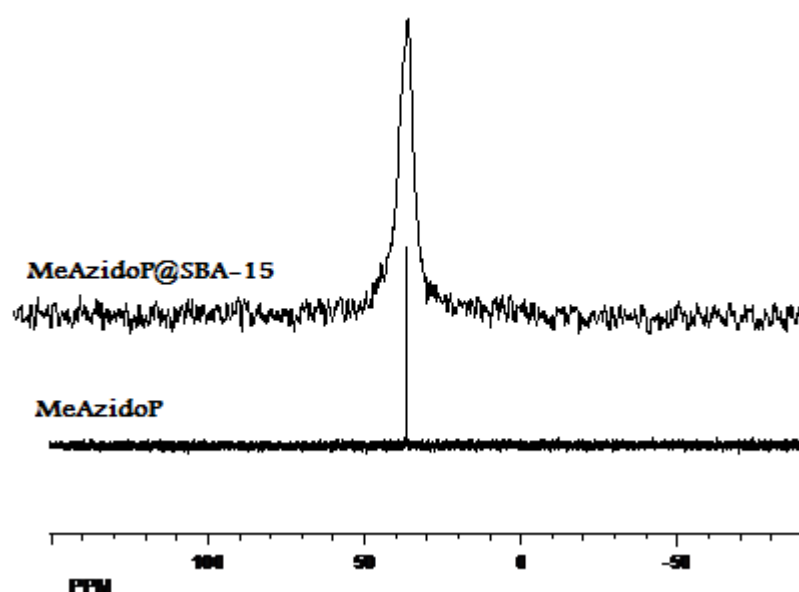
Figure III.S6. ^{31}\text{P} NMR of methyl azidophosphatane MeAzidoP and CP MAS ^{31}\text{P} of MeAzidoP@SBA-15.
