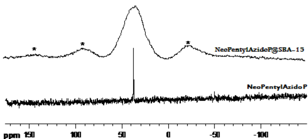
Figure III.S7. ^{31}\text{P} NMR of neopentyl azidophosphatane NeoPentylAzidoP and CP MAS ^{31}\text{P} of NeoPentylAzidoP@SBA-15. * denotes for spinning side bands.
