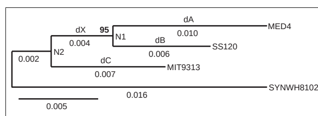
Figure 2 Phylogenetic tree of 16S rRNA genes from the four marine picocyanobacteria. Neighbor-joining tree with Kimura 2-parameter correction. The bootstrap value (1,000 replications) is shown in boldface. Lengths of the branches dA, dB, dC and dX (see text) are given below the branches. N1, node 1, branchpoint between MED4 and SS120; N2, node 2, branchpoint between MIT9313 and Node 1.
