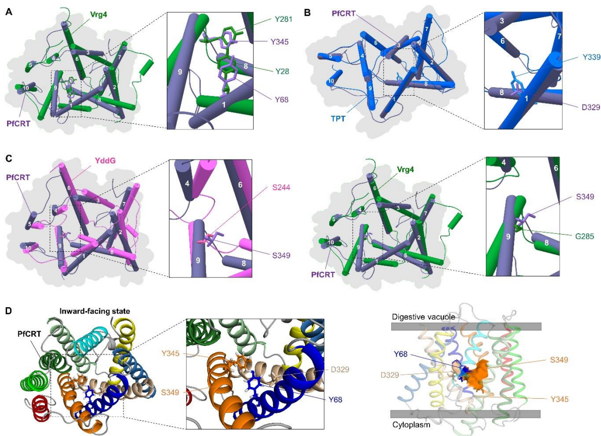
Figure 4. Comparative structure-based alignment of evolutionary conserved CRT positions located in the putative binding pocket of PfCRT. Structural alignment of PfCRT (grey purple) with (A and C) the Vrg4 (PDB ID: 5oge, green forest), (B) TPT (PDB ID: 5y79, blue) and (C) YddG (PDB ID: 5i20, pink) proteins using the align function in UCSF Chimera. The TMs helices are numbered. The PfCRT inward-facing state was aligned with Vrg4 and YddG, while the PfCRT occluded state was aligned with the TPT protein. (D) Location of the four putative PfCRT functional sites Y68, D329, Y345 and S349 in the PfCRT inward-facing state model. The structure is shown from the vacuolar face (left panel) with a zoom on the proposed functional positions, and from the side (right panel), as cartoon while candidate functional positions are shown in surface. These four amino acid positions cover a large part of the putative binding pocket.
