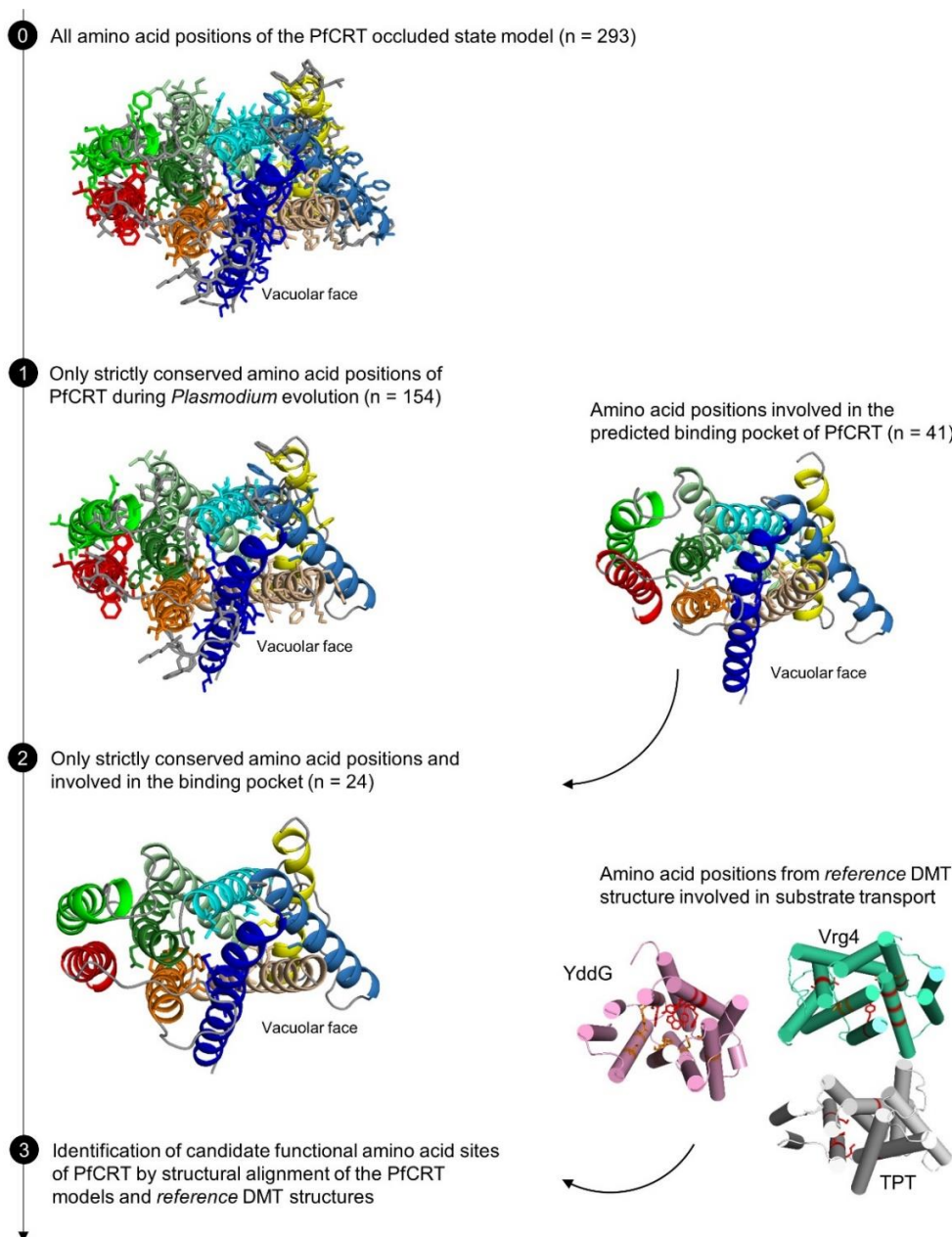
Supplementary Figure S10. Pipeline describing the filtering of PfCRT amino acid sites for the identification of PfCRT candidate functional sites. The PfCRT occluded state model is colored according to TMs. YddG, Vrg4 and TPT proteins are colored in pink, blue-green and grey, respectively. Functional amino acid sites of these proteins are shown in stick and colored in red. Starting with the PfCRT occluded state model covering 293 amino acid positions of the PfCRT sequence, only the strictly conserved amino acid sites at the Plasmodium scale were selected (n = 154). Next, the amino acid sites involved in the architecture of the predicted binding pocket (based on our model) were selected (n = 41). Among these sites, those that are strictly conserved during Plasmodium evolution were kept (n = 24). Finally, the PfCRT models (occluded and inward-facing states) were structurally aligned with the different reference DMT structures used in this study ( i.e. YddG, Vrg4 and TPT proteins). We then focused on the subset of PfCRT amino acid sites that structurally aligned with experimentally-tested and validated amino acid sites of the reference DMT proteins.
