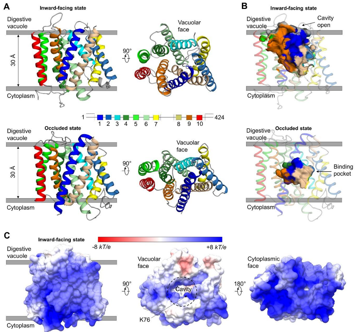
Figure 2. 3D-fold and structural features of the predicted inward-facing and occluded states of PfCRT. (A) Predicted tertiary structure of PfCRT in inward-facing ( top panels) and occluded ( bottom panels) states. Each TM is highlighted in a specific color. (B) Location of the cavity and the substrate-binding pocket (binding pocket) in the PfCRT models. In the inward-facing state, the cavity of PfCRT is open from the vacuolar face. In the occluded state, a substrate-binding pocket constitutes the core of the transporter. (C) Electrostatic surface potential of the inward-facing state of PfCRT. Values are in units of kT/e at 298 K, on a scale of -8 kT/e (red) to +8 kT/e (blue). White color indicates a neutral potential. The structure is shown from the side, vacuolar face and cytoplasmic face from the left to right respectively. The location of the key position K76 in CQR is indicated.
