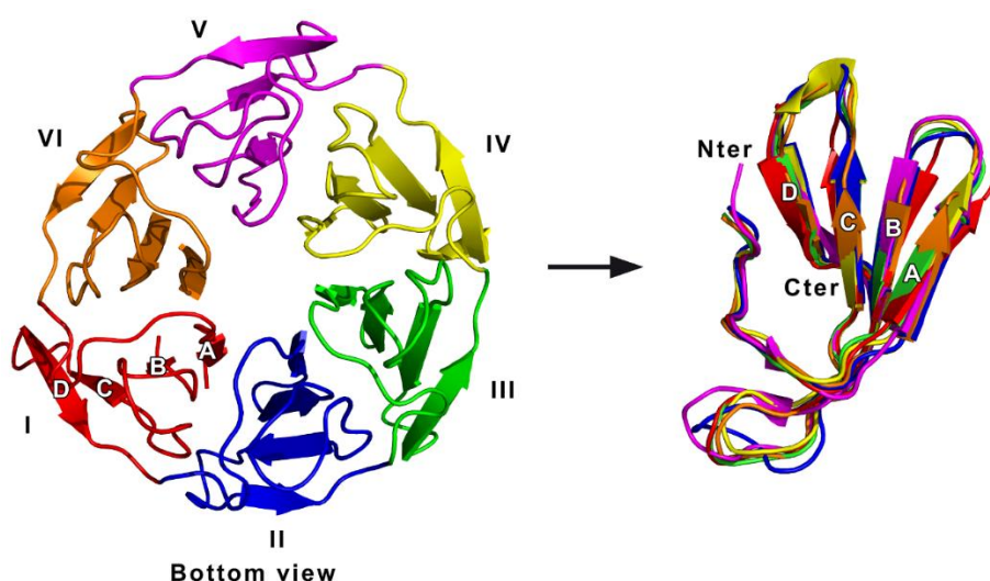
Figure S8. Structure-based alignment of the six blade repeats of Pfk13 KREP. We used the Pfk13 BTB-KREP structure solved by X-ray diffraction at a resolution of 1.81 Å (PDB code 4YY8, chain A). The Pfk13 KREP structure is shown as cartoon. The six blades are colored differently: red, blade I; blue, blade II; green, blade III; yellow, blade IV; magenta, blade V; orange, blade VI. The four strands within each blade are labelled A to D, from the innermost to the outermost. The KREP structure was divided into six PDB files, each one containing the atomic coordinates of one blade. Then, the six blade structures were aligned by minimizing the root-mean-square deviation (RMSD) of atomic positions using the align function in PyMOL (Schrödinger, LLC) ( right ). This structure-based alignment of the K13 KREP blades was then used to produce the amino acid sequence alignment of the six blades shown in Figure 4a. The blade length ranged from 46 (blade VI) to 49 (blade V) amino acids, the pairwise blade sequence conservation level ranged from 15.2% (blades III/VI) to 33.3% (blades IV/V), and the pairwise blade structure comparison indicated a RMSD ranging from 0.394 Å 2 (blades I/III) to 0.669 Å 2 (blades I/IV).
