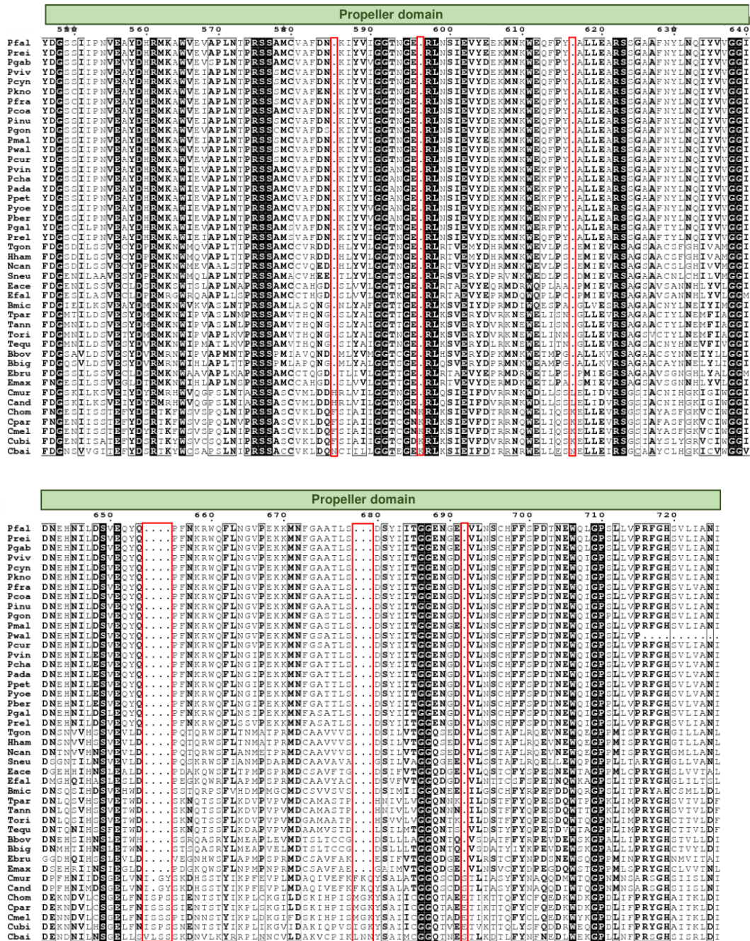
Figure S1. K13 multiple amino acid sequence alignment. The K13 multiple sequence alignment was performed using Mafft version 7. Strictly conserved positions are written in white letters and shaded in black, and highly conserved positions are boxed with black lines and written in white, bold letters (the level of conservation is based on BLOSUM62 scoring matrix). A four-letter code is used for the name of species (full species names are provided in Supplementary Table S1). The regions of the alignment with highly divergent positions, as well as positions containing gaps in at least 30% of all sequences, were manually removed (red boxes). The multiple alignment was displayed with the ESPrnt 3.0 server. The annotated domains of K13 (Coiled-coil containing, BTB and propeller (or KREP)) are shown above the K13 multiple sequence alignment.
