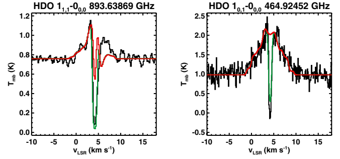
Fig. 3. In black: HDO 1_{1,1}-0_{0,0} and 1_{0,1}-0_{0,0} absorption lines observed at 894 GHz with HIFI and at 465 GHz with JCMT, respectively. In red: HDO modeling without adding the absorbing layer. In green: HDO modeling when adding an absorbing layer with a HDO column density of \sim 2.3 \times 10^{13} \text{ cm}^{-2} . The continuum for both the 894 GHz and 465 GHz lines refers to SSB data.
