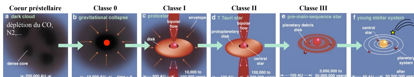
FIGURE 1.1 – Les diff rentes  tapes de la formation stellaire (Source : Spitzer Science Center).
