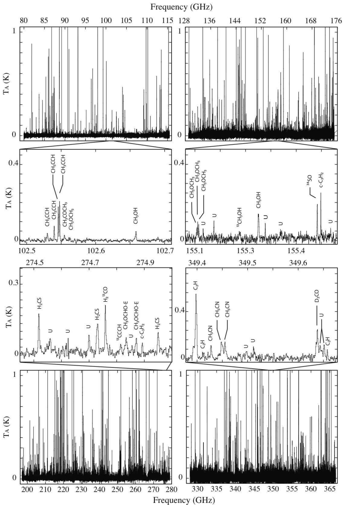
Fig. 2. The IRAS 16293 spectra in the four bands of the survey. Upper panels: IRAM-30 m 3 mm and 2 mm bands. Lower panels: IRAM-30 m 1 mm and JCMT-15 m 0.9 mm bands. The middle panels are zoomed views of sample frequency ranges in the four bands respectively. These panels include lines identification based on the publicly available spectral databases (see text for details).
