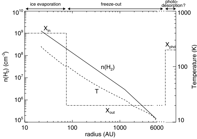
Fig. 2. \text{H}_2 density (solid line) and gas temperature (dashed line) structure of IRAS 16293 determined by Crimier et al. (2010) . The expected abundance profile of water is added (dashed-dotted line) on an arbitrary Y-scale. In the colder envelope ( T < 100 K), the water molecules are trapped on the grain mantles, whereas in the inner part of the envelope, they are released in gas phase by thermal heating, leading to an enhancement of the abundance. In the outer part of the molecular cloud ( A_V \sim 1\text{--}4 ), the water abundance can also increase by photodesorption mechanisms. A freeze-out timescale much longer than the protostellar lifetime can also lead to an enhanced abundance when the density is low ( \sim 10^4 \text{ cm}^{-3} ).
