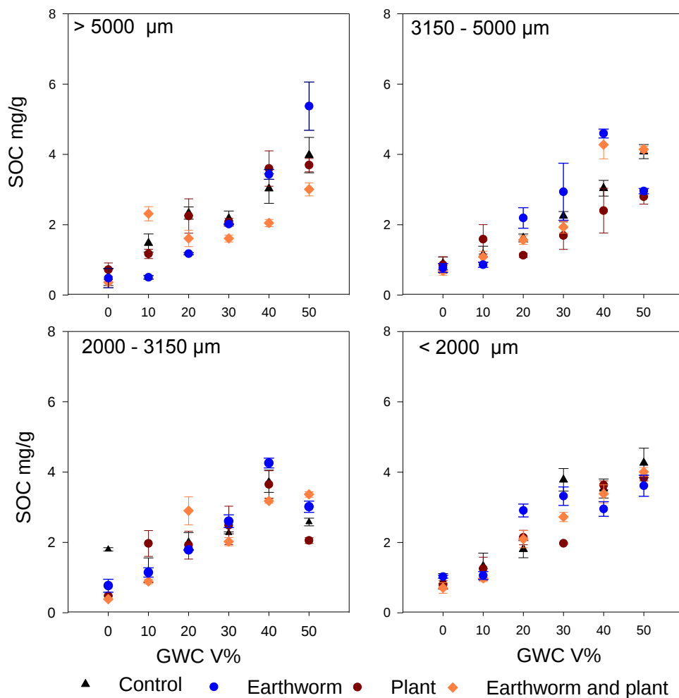
Fig. 2. Soil organic content in the aggregate > 5000 \mu\text{m} , aggregates between 5000-3150, aggregates between 3150-2000, aggregates <2000 in the different percentage of green waste compost 0%, 10%, 20%, 30%, 40%, 50%. Error bars represent the standard error about the mean.
