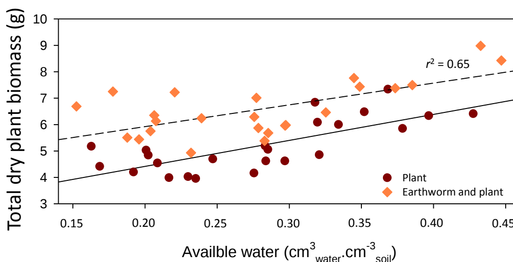
Fig. 7. Linear regression between total dry plant biomass and available water ( \text{cm}^3_{\text{water}} \cdot \text{cm}^{-3}_{\text{soil}} ) with earthworm (dotted line) or without earthworm (plain line). Plant biomass was higher with earthworms than without ( P < 0.001 ). Total plant biomass increased with available water, but the difference in slope of the two linear regressions was not significant. The best equations fitting the relation between total dried plant biomass (X, g) and plant available water ( \theta_{\text{Total}} , \text{cm}^3_{\text{water}} \cdot \text{cm}^{-3}_{\text{soil}} ) are: X = 8.97 \cdot \theta_{\text{Total}} + 4.07 and X = 8.97 \cdot \theta_{\text{Total}} + 2.69 with and without earthworms, respectively ( P < 0.001 , adjusted r^2 = 0.65 ).
