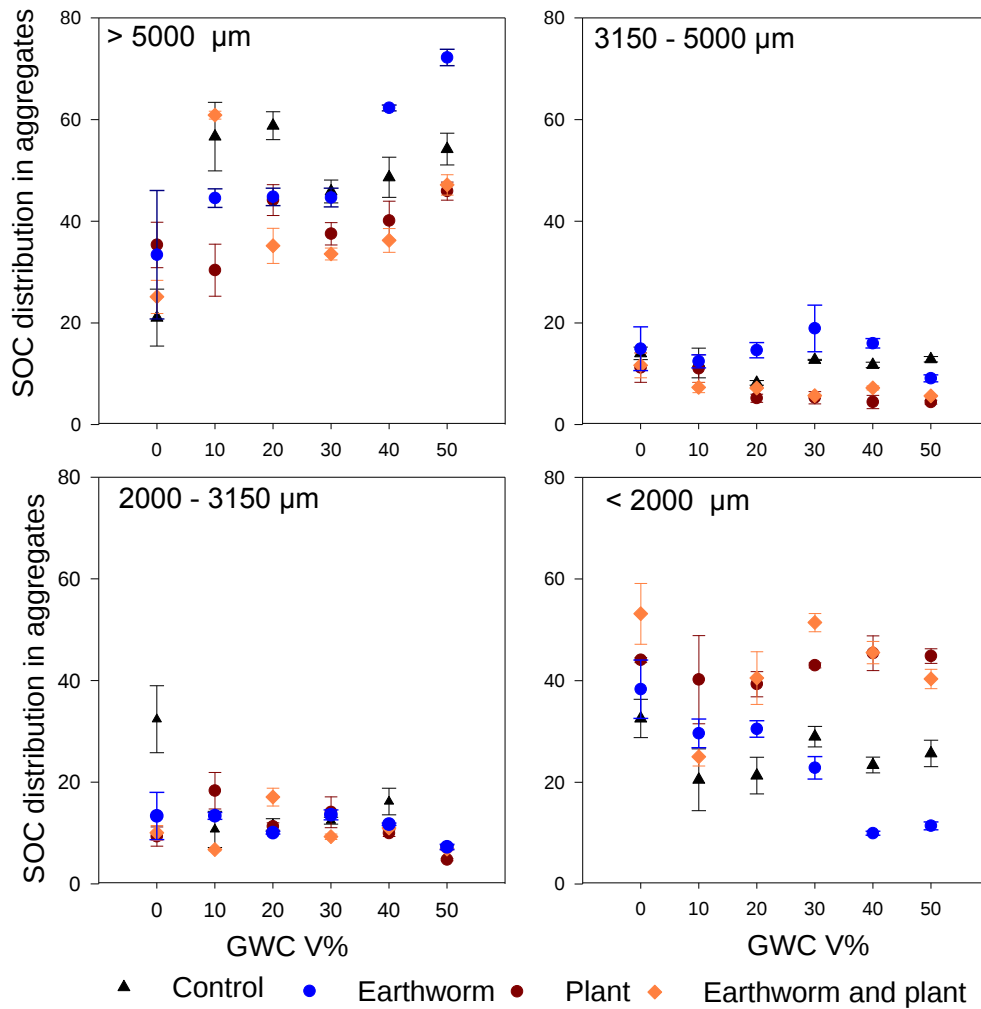
Fig. 3. Soil organic carbon distribution in the aggregates classes > 5000\mu\text{m} , aggregates between 5000\text{-}3150 , aggregates between 3150\text{-}2000 , aggregates <2000 in the different percentage of green waste compost 0%, 10%, 20%, 30%, 40%, 50%. Error bars represent the standard error about the mean.
