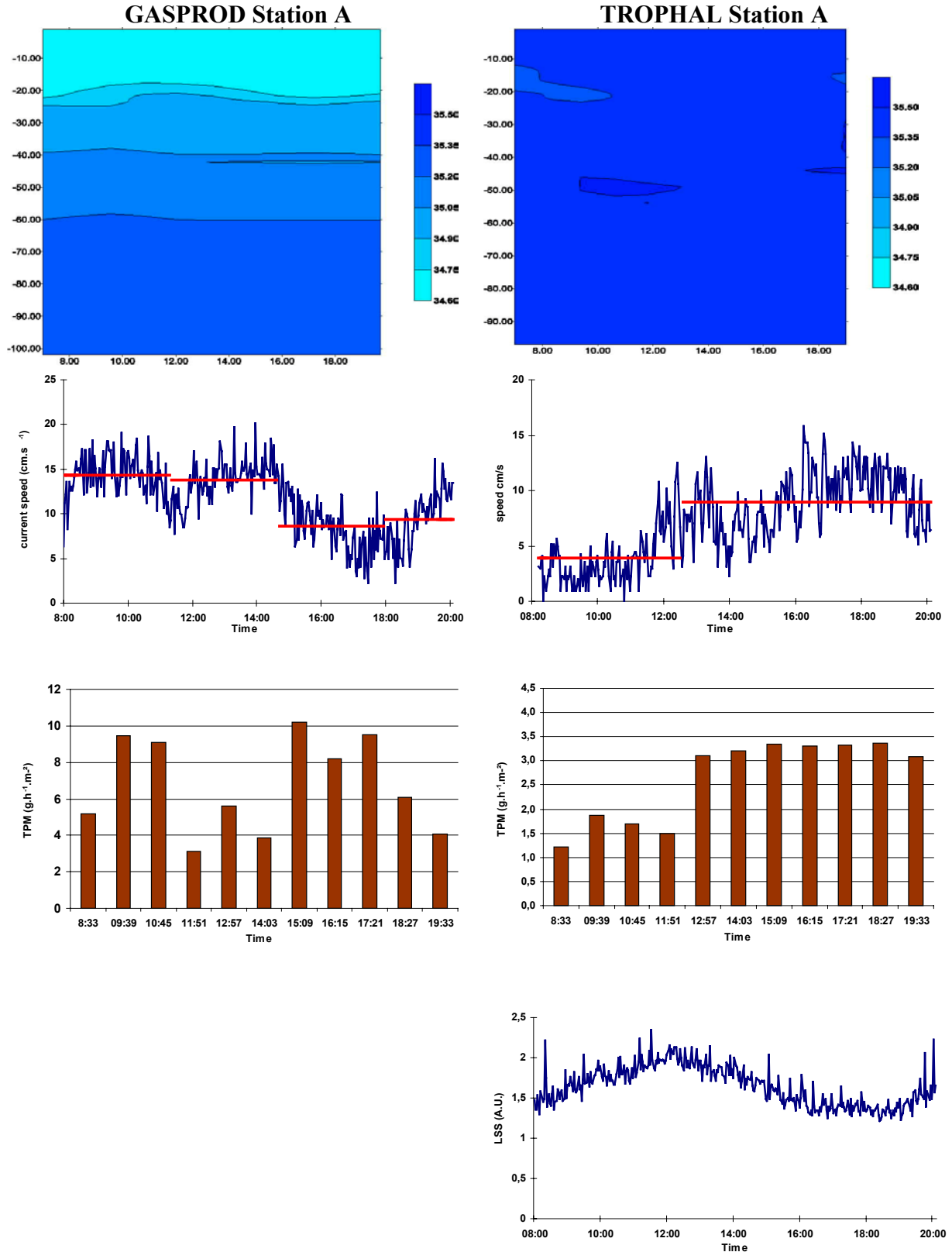
Figure 8. Station A. High-frequency temporal variability of particulate matter sedimentation (TPM, g.m -2 .h -1 ) in bottom trap in relation to current velocity (cm.s -1 ) and light scattering (a.u.) 1.6 m off the seabed. Water salinity measured by the SBE25 CTD probe is also represented.
