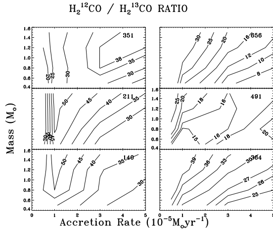
Fig. 4. The H 2 12 CO over H 2 13 CO line ratio of the same transitions of Fig. 3.
