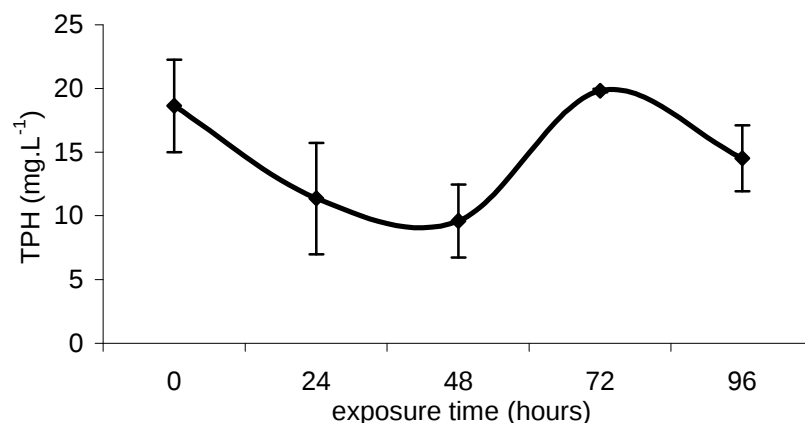
Fig 1. (Figure 35) : Total petroleum hydrocarbons (TPH) concentrations (mg.L -1 ) in seawater during the 96 hours exposure of sea bass to petroleum. Values are expressed as mean of both experimental replicates (mean ± SE).
