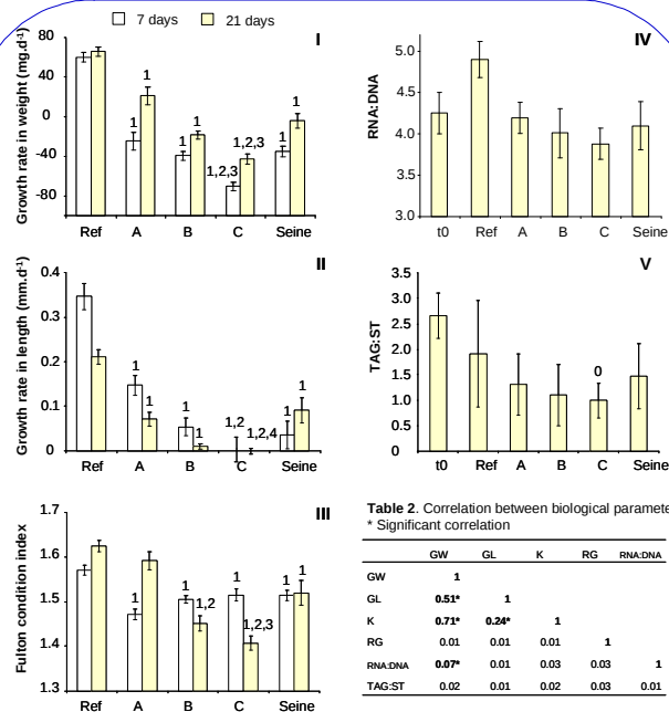
Fig 2. Comparison of the growth rate in weight (I), in length (II), the Fulton condition index (III), the RNA:DNA ratio and the lipid index (TAG:ST ratio) between fish exposed to the sediments. 0,1,2,3,4 : significant difference with t0, Ref, A, B, Seine
