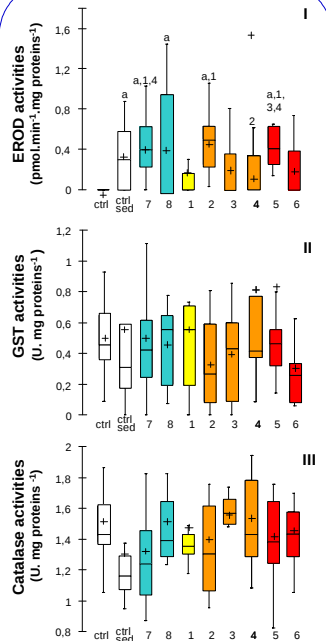
Fig. 2 : Comparison of hepatic EROD (I), GST (II) and Catalase activities (III). a, i (1...4) : significant difference with control (ctrl) and site i.
