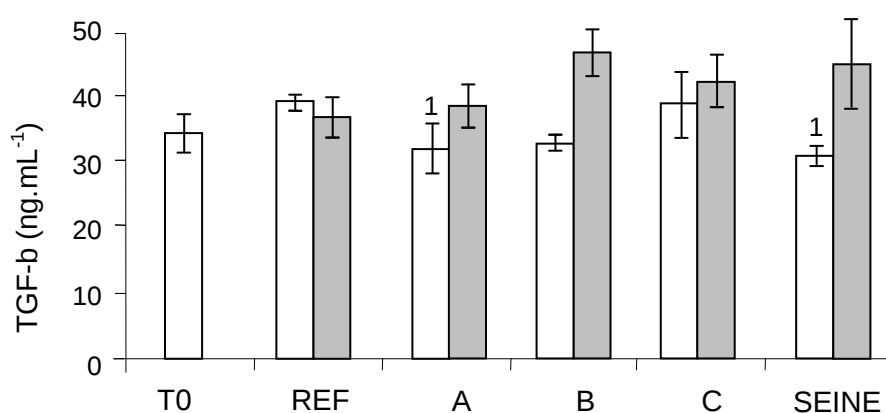
Fig. 4 (Figure 63): Differences in plasmatic levels of TGF-b1 (ng.mL -1 ) of turbot exposed to the five sediments (Ref, Seine, A, B and C) during 7 (□) and 21 (■) days. n= 3. ( 0 ), ( 1 ), ( 2 ), ( 3 ), ( 4 ), ( 5 ), ( 6 ) represent significant difference (p < 0.05) compared to “t 0 ”, Seine, A, B, C and starved fish, respectively.
