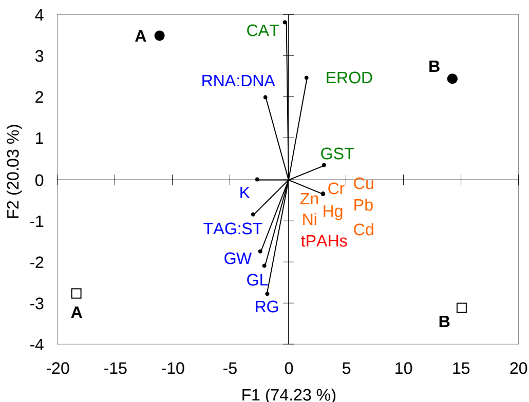
Fig. 4 (Figure 54): PCA based on biomarker responses (Ethoxyresorufin-O-deethylase -EROD-, Glutathione S-transferase -GST- and Catalase -CAT) of juvenile sea bass (□) and turbot (●) in relation with physiological biomarkers (specific growth rate in length -GL- and weight -GW-, recent growth -RG-, Fulton's condition index -K-, RNA:DNA and Triacylglycerol on sterol -TAG:ST- ratios) and chemical contamination (metals and total PAHs) measured in caging station A and B.
