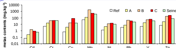
Fig 1. Metal concentrations (mg.kg -1 ) in sediment
