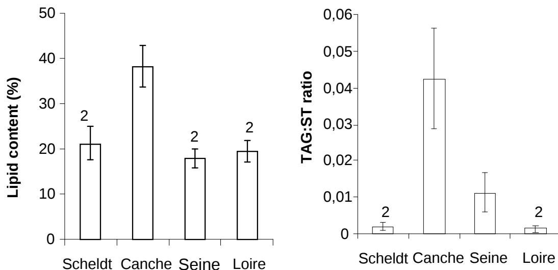
Fig. 4 (Figure 68) : Comparison of (a) lipid contents and (b) TAG:ST ratios of flounders sampled in the four estuaries. n=10. (1), (2), (3), (4) represent significant difference ( p < 0.05 ) compared to Scheldt, Canche, Seine and Loire respectively.
