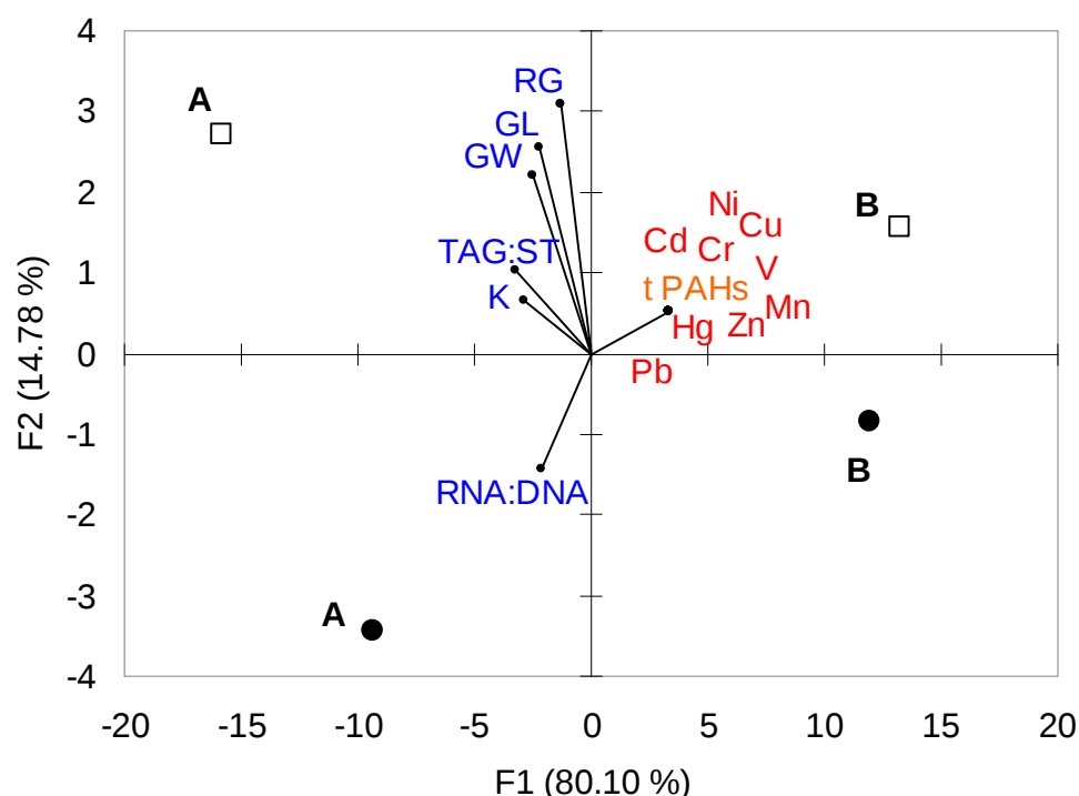
Fig. 4 (Figure 50) : PCA based on biological parameters (specific growth rate in length (GL) and weight (GW), recent growth (RG), Fulton's condition Index (K), RNA:DNA and TAG:ST ratios) of juvenile sea bass (□) and turbot (●) in relation with chemical contamination (metals and total PAHs) measured at caging stations A and B.
