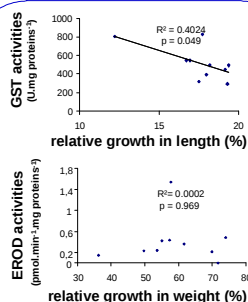
Fig. 4 : Correlation between biomarkers and relative growth.
