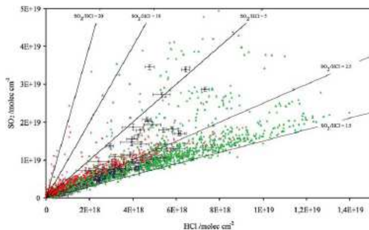
FIGURE 7 Column amounts of \text{SO}_2 and \text{HCl} for all spectra recorded on 9 January 2005 at Yasur: sets 1 (crater A, red circles), 2 (crater B, blue squares), and 3 (crater B, green triangles). Solid lines indicate given \text{SO}_2/\text{HCl} ratios. Passive gas has a typical \text{SO}_2/\text{HCl} molar ratio of between about 1.5 and 2.5 but there is a hint that the ratio is slightly higher for crater A than for B. Higher ratios indicate contributions from explosive gas. Given that the viewing geometry probably always contains some passive gas, the highest ratios ( > 20 ) indicate a lower limit to the \text{SO}_2/\text{HCl} proportion in explosive gas. Errors for set 2 shown as a guide
