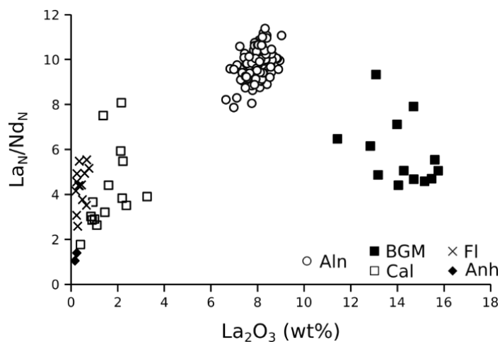
Figure 4.14. La_N/Nd_N (Sun and McDonough, 1989) versus La_2O_3 (wt%) plot for allanite and secondary minerals with significant LREE.
