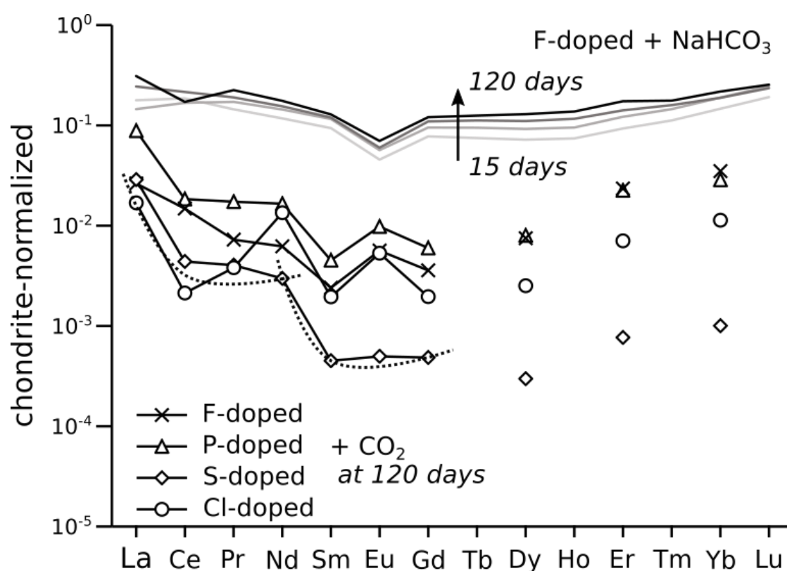
Figure 4.16. Chondrites-normalized REE pattern of fluids after 120 days for low-acid experiments F- (B1120), P- (B3P120), S- (B3S120), Cl-doped (B3Cl120) and in time series for alkaline F-doped experiment (B2). HREE with odd number are below detection or removed from the diagram because artificial anomalies are induced by close-to-detection limits (Table 4.3). The lanthanide tetrad effect is discernible within the LREE in low-acid experiments (dashed lines). After Sun and McDonough, 1989.
