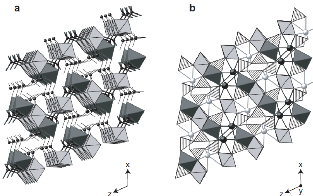
Figure 4.2. Structure cristalline de l'allanite d'après. Crystal structure of allanite, drawn with CrystalMaker® using data from Dollase (1971). The structure consists of chains of edge-sharing octahedra, which are parallel to [010]: M(1) and M(2) sites are the light gray octahedra; M(3) octahedra are shown as dark octahedra. These chains are linked by single SiO 4 tetrahedra and double-tetrahedral groups (Si 2 O 7 ). (a) Simplified diagram showing M and T sites only, viewed slightly off the b axis: Si(3) forms an isolated SiO 4 group (shown as sphere with stick bonds); Si(1) and Si(2) share an oxygen, forming an Si 2 O 7 group (shown as spheres with wire bonds). (b) View parallel to the b axis: the SiO 4 and the Si 2 O 7 groups are both shown as striated tetrahedra. The large cavities in the framework contain Ca 2+ (small light gray spheres) and REE 3+ (black spheres) in 9-fold and 11-fold coordination by oxygen, respectively.
