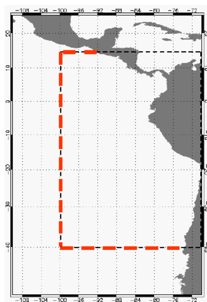
Fig. 2.9. Regional domain (dashed black lines) within the eastern South Pacific, with open boundaries (dashed red lines) at 100^\circ\text{W} , 15^\circ\text{N} and 40^\circ\text{S} . Grey colour is for land.
