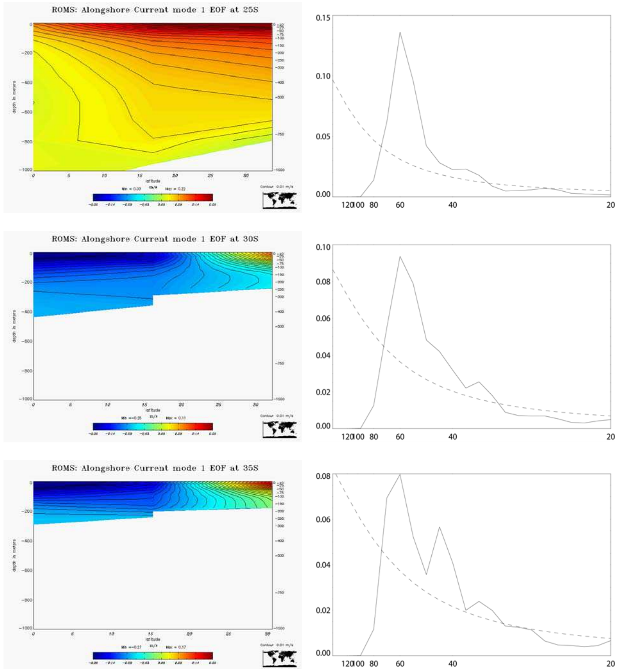
Fig. 3.22. First EOF mode of [50-70 days] band-pass filtered alongshore current anomalies performed from the surface to the bottom over cross-shore sections of lengths close to the first Rossby radius of deformation at (from top to bottom): 5°S, 10°S, 15°S, 20°S (previous page), 25°S, 30°S, 35°S (this page). For each latitude: 1 st EOF mode spatial pattern (left), and frequency spectrum of the 1 st EOF PC time series (right). Spatial patterns are plotted as a function of landward cross-shore distance (km) and depth (m). Units are m/s and contour interval is 0.01 m/s. Spectra are plotted as a function of frequency, and equivalent periods (days) are indicated. Full line is for PC, and dashed line is for red noise spectrum with the same lag-1 autocorrelation.
