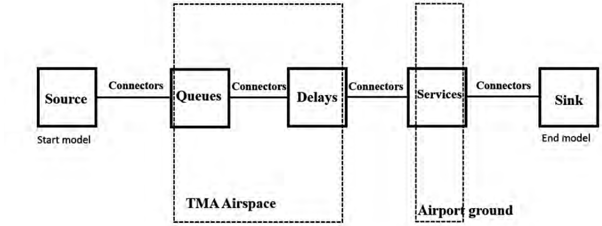
Figure B.1: Schema of the simulation model of the Opt-sim Method 2
