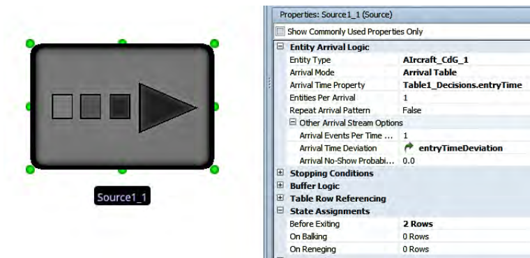
Figure A.7: Source object properties (SIMIO)
