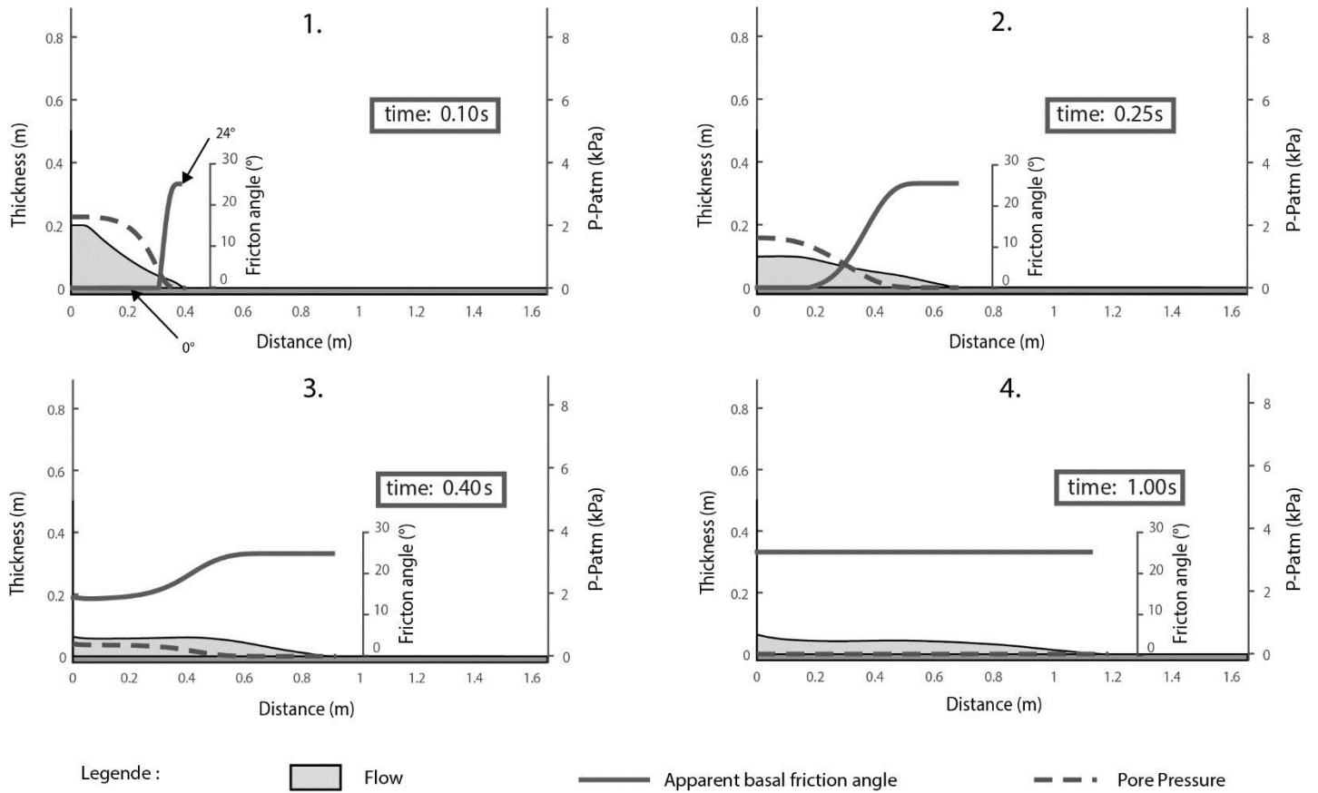
Figure S2. Evolution of the basal pressure during the emplacement of an initially fluidized flow (dashed line). The evolution of the basal friction angle is represented by the solid line. The initial granular bed (grey surface) is 20 cm high and wide. We show that the pressure decreases first at the front because it is thinner, and this phenomena propagates backwards with time. In contrast, the basal friction angle is near zero at the beginning of the calculation and increases as the pressure decreases.
