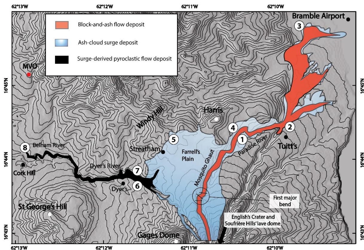
Figure 1: Map of deposits (block-and-ash flow, ash-cloud surge, and surge-derived pyroclastic flow deposits) from the 25 June 1997 dome collapse of Soufrière Hills Volcano at Montserrat, from Druitt et al., (2002). Note that this map refers only to the surface area of deposits at the end of the collapse.
