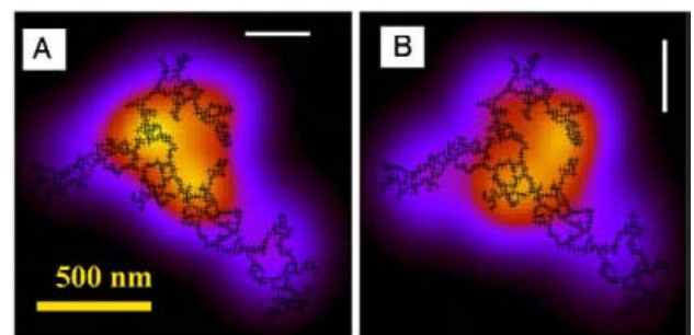
Fig. 6. (Color online) TPL maps computed with a PNN composed of 543 gold spheres of average radius a = 6 nm. The two images are overlaid with the PNN branches represented by black crosses. The white bars represent the polarization of the incident field, which is rotated 90^\circ when passing from map (A) to map (B). Image size, 1.2 \mu\text{m} \times 1.2 \mu\text{m} ; wavelength, 730 nm; beam waist, 275 nm.
