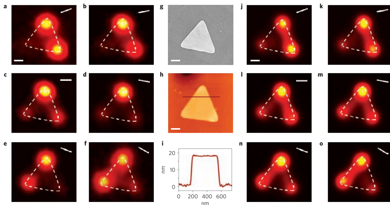
Figure 2 | Polarization control of TPL maps. a–g,j–o , Experimental ( a–f ) and theoretical ( j–o ) TPL images of the 790-nm triangular nanoprism, observed by SEM in g , h,i , AFM image ( h ) and height profile ( i ) of the same prism showing its uniform 20-nm thickness. The prism is excited at \lambda_0 = 800 nm with a linearly polarized light. The direction of the in-plane polarization is indicated by the white line in the upper right corners. The dashed white line is the outline of the considered nanoprism. Scale bars, 200 nm. The colour scale of ( a–f ) and ( j–o ) is similar to that of Fig. 1d. Simulation details for j–o are given in the main text and in Methods. Experimental TPL maps were processed as described in the Supplementary Information.
