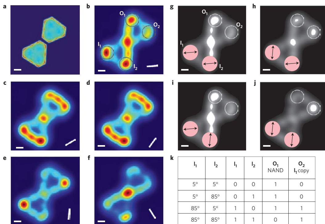
Figure 6 | Plasmonic modal logic gates in coupled nanoprisms. a , Simulated SP-LDOS map of the truncated triangular prism dimer shown in Fig. 5b. b–f , Simulated maps of the TPL signal for the coupled prisms for a series of incident linear polarization directions: 5° ( b ), 25° ( c ), 55° ( d ), 85° ( e ) and 120° ( f ). \lambda_0 = 800 nm, beam waist = 270 nm. The colour scale is similar to Fig. 5d–g. g–j , Time-lapsed illumination of I_1 and I_2 with a polarization orientation of 5° or 85° is correlated to the time-integrated TPL signal in O_1 and O_2 . Map g corresponds to inputs polarized at 5° on I_1 and I_2 , and results from the sum of b weighted by its maximal values in I_1 and I_2 . Map i corresponds to inputs polarized at 5° on I_1 and at 85° on I_2 , and results from the sum of b weighted by its maximal value in I_1 and e weighted by its maximal value in I_2 . Maps j and h are obtained by the same method. Map j corresponds to inputs polarized at 85° on I_1 and I_2 , and map h corresponds to inputs polarized at 85° on I_1 and 5° on I_2 . All four maps have been thresholded to the same value. k , Table summarizing the four illumination and detection configurations. Polarization of 5° (85°) in I_1 or I_2 is ascribed a 0 (1) binary code. Intensity in O_1 and O_2 is ascribed a 0 (1) digital value if it is below (above) the common threshold. O_1 accomplishes a NAND gate while O_2 duplicates the I_1 input. The direction of the in-plane polarization is indicated by the white line in the lower right corners. Scale bars, 200 nm.
