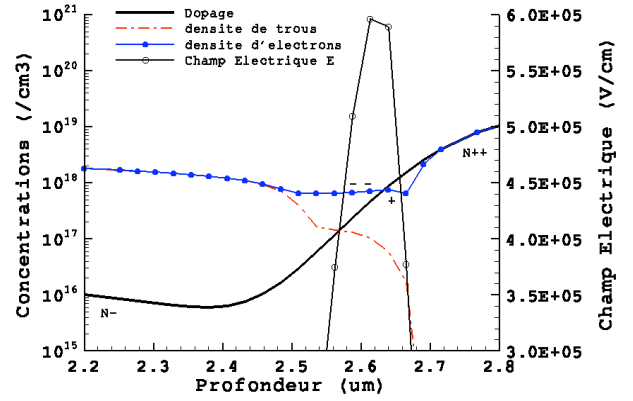
(c') Zoom I_{TLP}=1.2\text{A}
