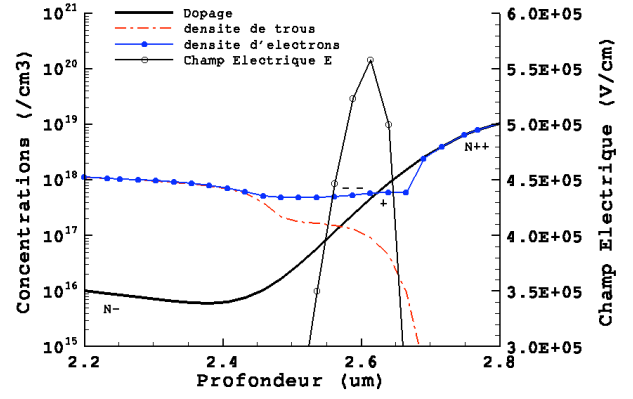
(a') Zoom I_{TLP}=800\text{mA}
