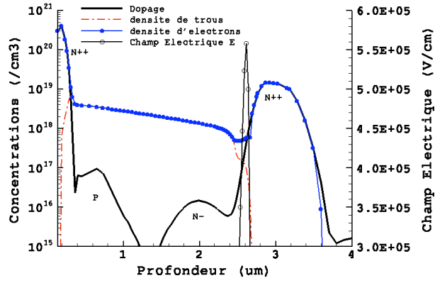
(a) I_{TLP}=800\text{mA}
