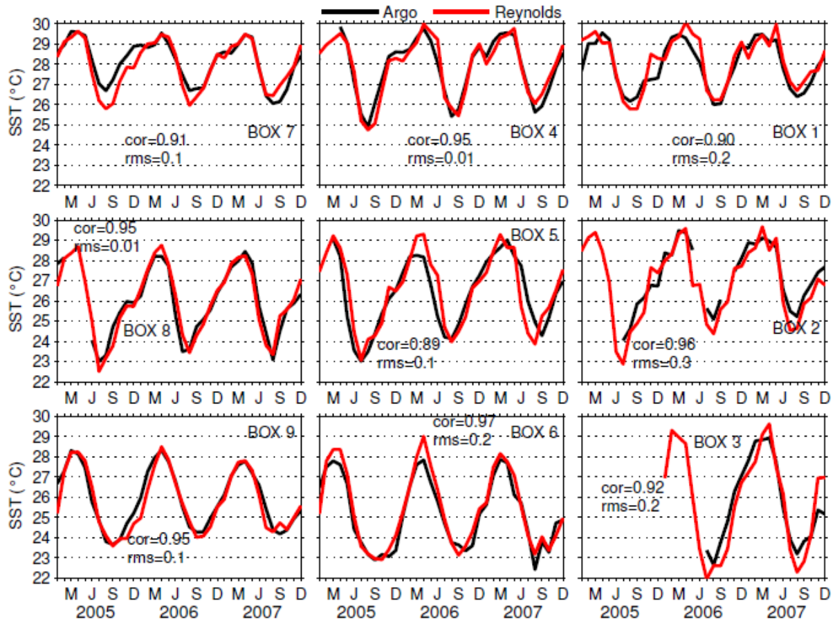
Figure 4: Interannual variability of the monthly sea surface temperature (°C) in 2005-2007 in the different boxes from ARGO data (black) and from Reynolds et al. [2007] (red). Correlations and root-mean square differences are also indicated.
