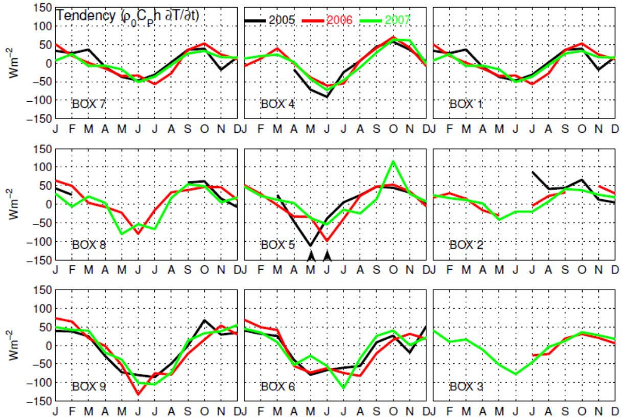
Figure 13: Heat storage rate evolution (in \text{W m}^{-2} ) in the different boxes in 2005 (black), in 2006 (red) and in 2007 (green).
