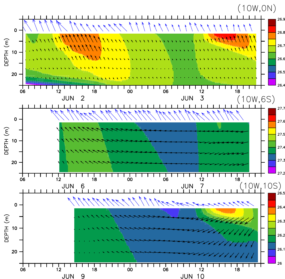
Fig. 10 Time–depth sections of temperature in the first 25 m and winds (blue vectors) at 10° W, 0° N (top), 10° W, 6° S (middle), and 10° W, 10° S (bottom) during the simulation. Currents relative to 25 m are superimposed (black vectors). Vector scales are 0.2 \text{ ms}^{-1} for the currents and 9 \text{ ms}^{-1} for the winds
