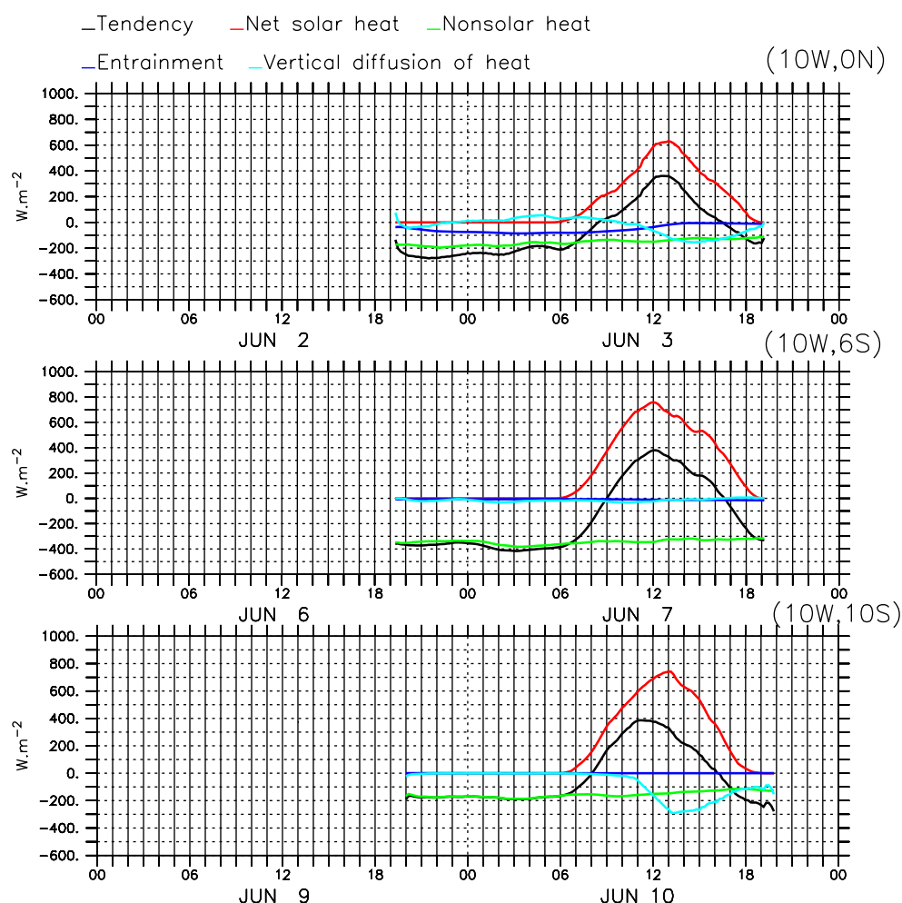
Fig. 12 Heat budget ( \text{W m}^{-2} ) over 24 h as a function of time at 0^\circ \text{ N} (top), 6^\circ \text{ S} (middle), and 10^\circ \text{ S} (bottom). Tendency is in black; solar heat flux in red; turbulent surface heat flux in green; vertical entrainment in blue; and vertical turbulent diffusion in cyan
