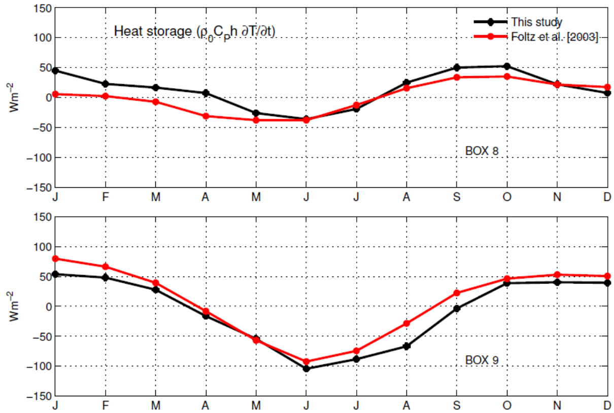
Figure 8: Comparison of the seasonal cycle of heat storage in boxes 8 (top) and 9 (bottom) (black curves) with Foltz et al. [2003] at two PIRATA mooring buoys along 10^\circ\text{W} respectively at the equator (top) and 6^\circ\text{S} (bottom) (red curves).
