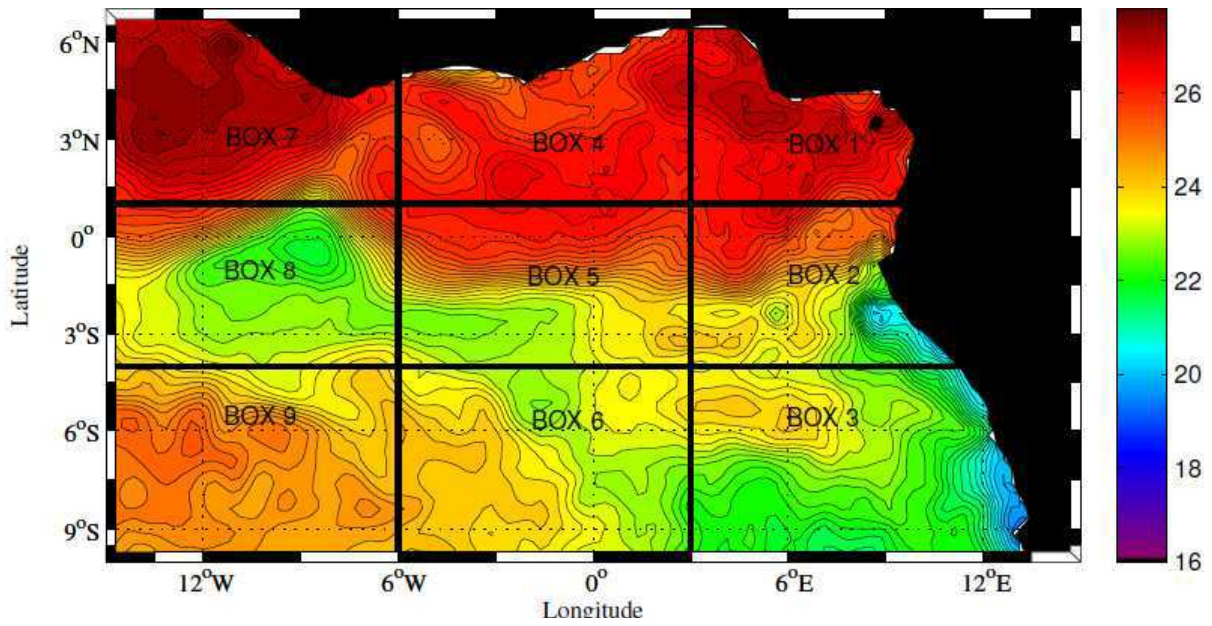
Figure 2: Spatial delimitation of the 9 boxes in the eastern equatorial Atlantic. SSTs from Reynolds et al. [2007] at 2005 July 15 are plotted.
