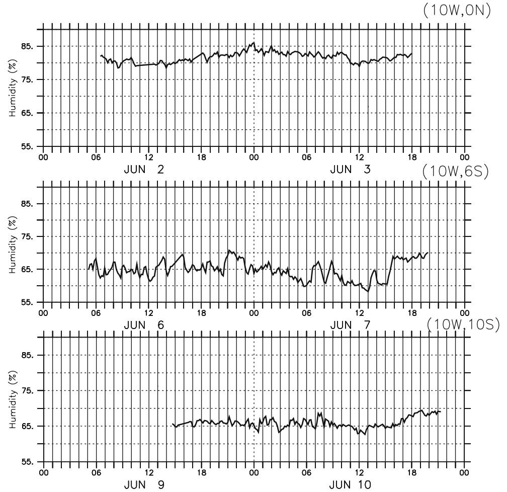
Fig. 4 Time series of the relative humidity (%) at 0° N (top), 6° S (middle), and 10° S (bottom)
