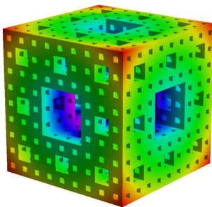
FIGURE 28 – Eponge de Sierpinski
