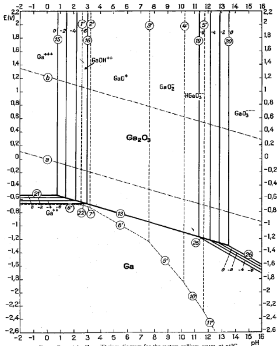
FIG. 1. Potential-pH equilibrium diagram for the system gallium-water, at 25°C.
