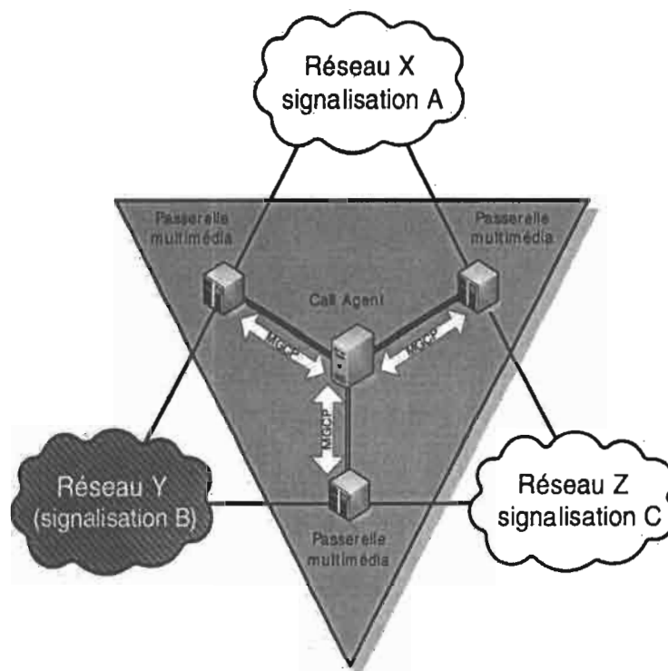
Figure II.2 : architecture MGCP [9]
