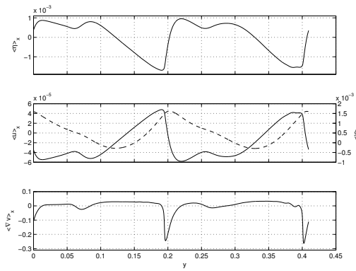
FIGURE 4.10 – Height (upper panel), cross-shock ( v ) and along-shock ( u ) velocities (middle panel, resp. in continuous and dashed lines) and divergence (lower panel) spatially averaged along a moving line of strong convergence.
