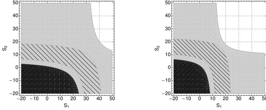
FIGURE 3.20 – Signs of (k_j/a)^2 in the (S_1, S_2) space for \delta = 0.2 (left) and \delta = 0.85 (right). Black zone : both k_1 and k_2 are imaginary. Grey zone : only k_1 (or k_2 ) is imaginary. Dashed zone shows that the value of J_1(k_1) (that is at the circle of radius a ) is between its first maximum and zero, which indicates where the solutions for S_1 and S_2 lie.
