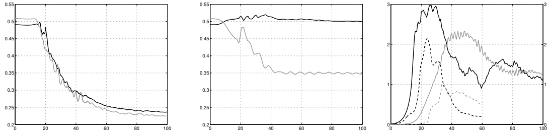
FIGURE 2.20 – Normalized integral of the positive (black) and negative (grey) potential vorticity anomalies (summed over the two layers) as a function of time for the l=2 centrifugal ( left panel ) and l=2 barotropic ( middle panel ) instabilities. Curves from the simulations of the initial destabilization and the subsequent evolution calculated in a refreshed numerical domain, in order to eliminate spurious reflexions of high-amplitude waves by the boundaries, are superimposed for the centrifugal instability. Right panel : Comparison of the magnitude of the baroclinic divergence inside (black, right axis) and outside (grey, left axis) a circle of radius \approx 1.9 R_d for the l=2 centrifugal (continuous) and barotropic (dashed) instabilities.
