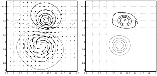
FIGURE 3.4 – Isobars with superimposed velocity field (left) and PV anomaly (right) of the NAGM of Fig. 3.2 at t = 80 . Isobars at the interval 0.04, PV from \pm 0.1 at the interval 0.5. Thin dotted line on the left panel indicates the zero of the pressure anomaly.
