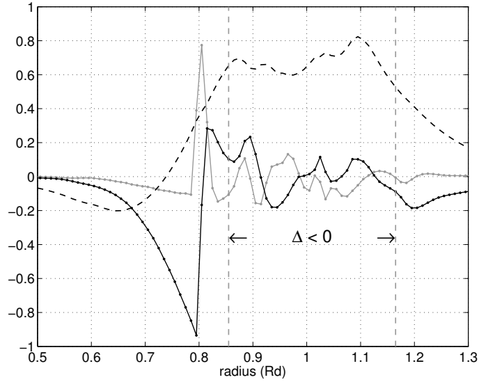
FIGURE 2.12 – Saturation of the axisymmetric centrifugal instability : radial distribution of the radial and azimuthal components of the baroclinic velocity, and of its divergence, at a given polar angle at t = 4.5 f^{-1} .
