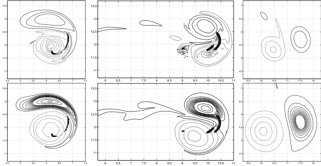
FIGURE 3.33 – PVA contours for the AGM with initial Ro = 0.4 and d = 0.8 . From left to right : t = 8, 40 (initial adjustment with shock formation) and 200 (ending stage). First row : layer 1 ; second row : layer 2. Contours at interval 1 from \pm 0.2 to 9.2 for both layers, and 5 from \pm 15 (applicable to cyclone only). Contour for dissipation higher than 7.5 \cdot 10^{-3} is superimposed, to visualize the shock, in thick black line.
