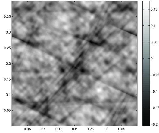
FIGURE 4.9 – Divergence field at t = 10 for a random IGW initialization.
