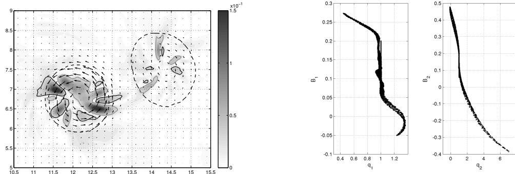
FIGURE 3.53 – Baroclinic divergence with superimposed velocity field at t = 152 (left, with same conventions as in Fig. 3.37), and scatter plots (two right panels) at t = 180 (same conventions as in Fig. 3.27), for a typical two-layer NAGM. True maximum value for the divergence is 0.3.
