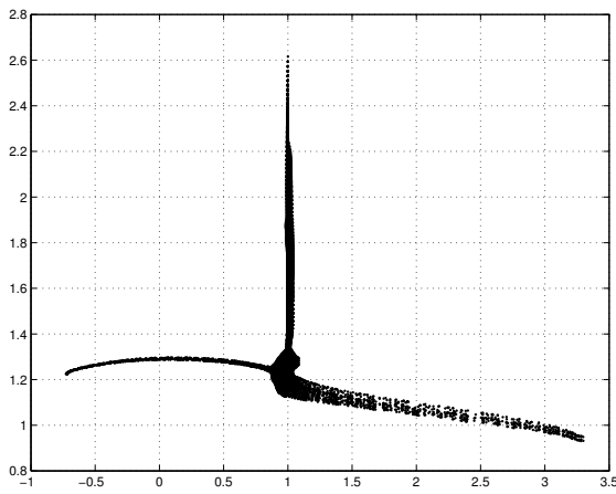
FIGURE 3.10 – Bernoulli function vs PV for the tripole at t = 76 .
