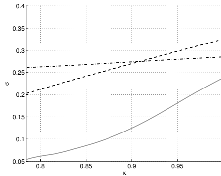
FIGURE 2.8 – Evolution of the growth rate of the unstable modes of a vortex with Ro = 1.4 , Bu = 7 , \delta = 1 and d = 0.9 as a function of \kappa . Same legend as in Fig. 2.7.
