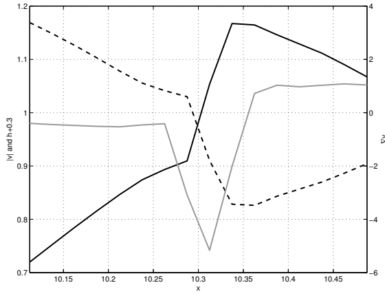
FIGURE 3.15 – |\mathbf{v}|/\sqrt{gH_0} (Froude number) - black, thickness h + 0.3 (dashed), and divergence \nabla \cdot \mathbf{v} (gray) profiles along the modon's axis at t = 46 .
