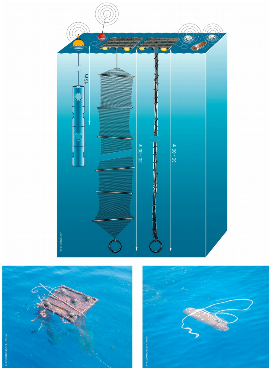
Figure 3.1: Description of the structure and design (in the water column) of a typical drifter (upper left) and of fish aggregating devices (FADs) used in purse seine fisheries including artificial rafts with a sea anchor made of ‘curtain’ nets (upper middle left, lower left photo) or ‘sausage’ nets (upper middle right) and natural logs (upper right, lower right photo).
