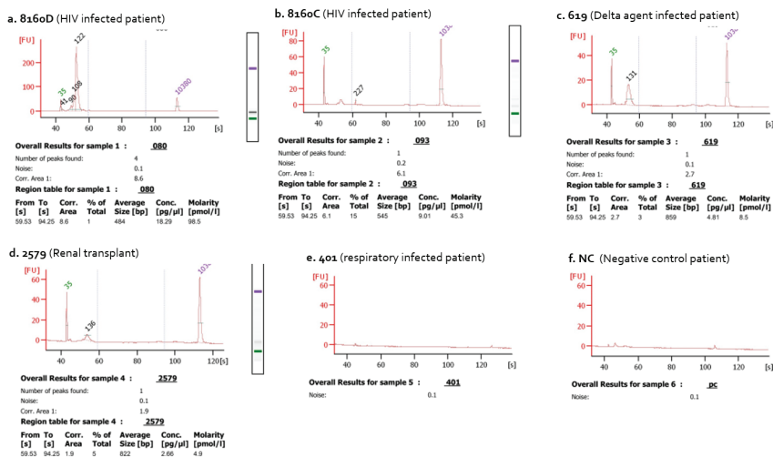
Figure 20: Bioanalyzer electropherogram DNA library profiles (Agilent 2100 Bioanalyzer system) of the 6 selected clinical samples after library preparation and size selection
