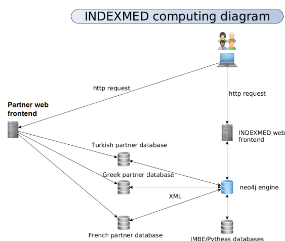
Figure 2. Global hardware architecture: it provides graph results from local or remote databases. Each partner will store data locally and the system will be able to get results using standard protocols. Graph results can be obtained by end users using a specific web frontend. 3 countries are testing the architecture under European programs and inventories of marine biodiversity (CIGESMED, DEVOTES, ZNIEFF). In addition, queries on remote databases are being tested (e.g. GBIF (species occurrences), Tela Botanica (French Flora), European Pollen databases. Other thematic databases will be integrated in the development of this project.
