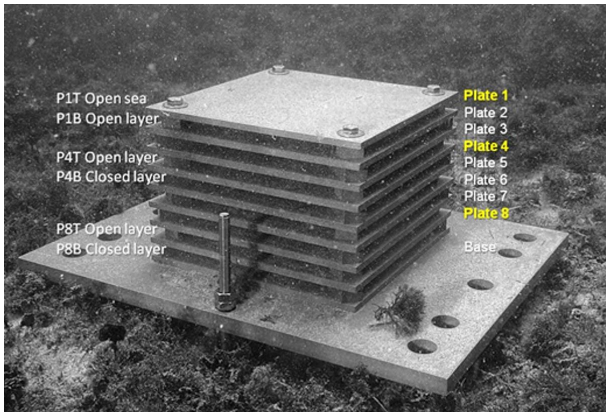
Figure 2: A newly deployed ARMS (Ile de l'Erevine, NW Mediterranean). The alternative use of long and short PVC cross spacers give a tower of four open and four closed layers. © photo CNRS / F. Zuberer.
