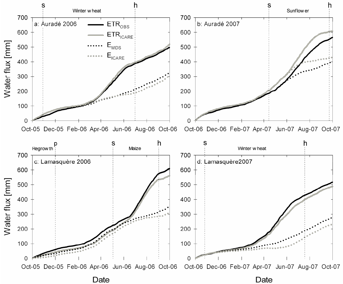
Figure 3: Comparison of cumulated evapotranspiration (ETR) measured by EC ( ETR_{OBS} ) and simulated with the ICARE-SVAT model ( ETR_{ICARE} ), and soil evaporation (E) calculated with the marginal distribution sampling method ( E_{MDS} ) and with the ICARE-SVAT model ( E_{ICARE} ) for both sites and both years. Annotations indicate date of sowing (s), harvest (h) and ploughing (p) and the name of the growing crop (or regrowth event).
