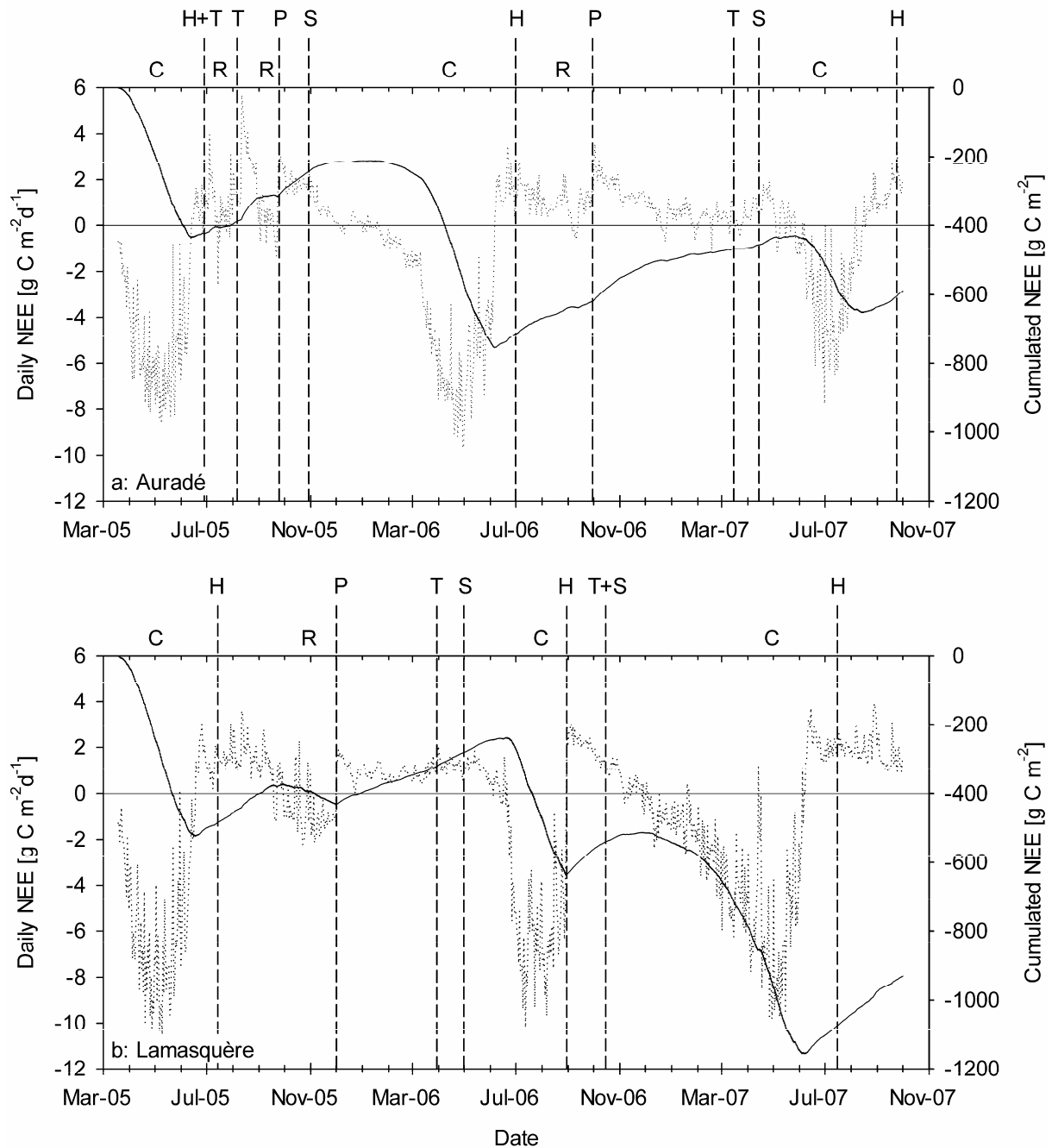
Figure 5: Daily net ecosystem exchange (NEE) evolution (left axis) and cumulated values of NEE (right axis) from 18-Mar-2005 to 01-Oct-2007 at the Auradé (a) and Lamasquière (b) plots. Crop development (denoted as C) and re-growth (denoted as R) periods were reported at the top of each subplot. Annotations corresponding to vertical dotted lines give information about punctual management operations affecting NEE: S is crop sowing, H is harvest and T and P are superficial tillage and deep ploughing, respectively.
