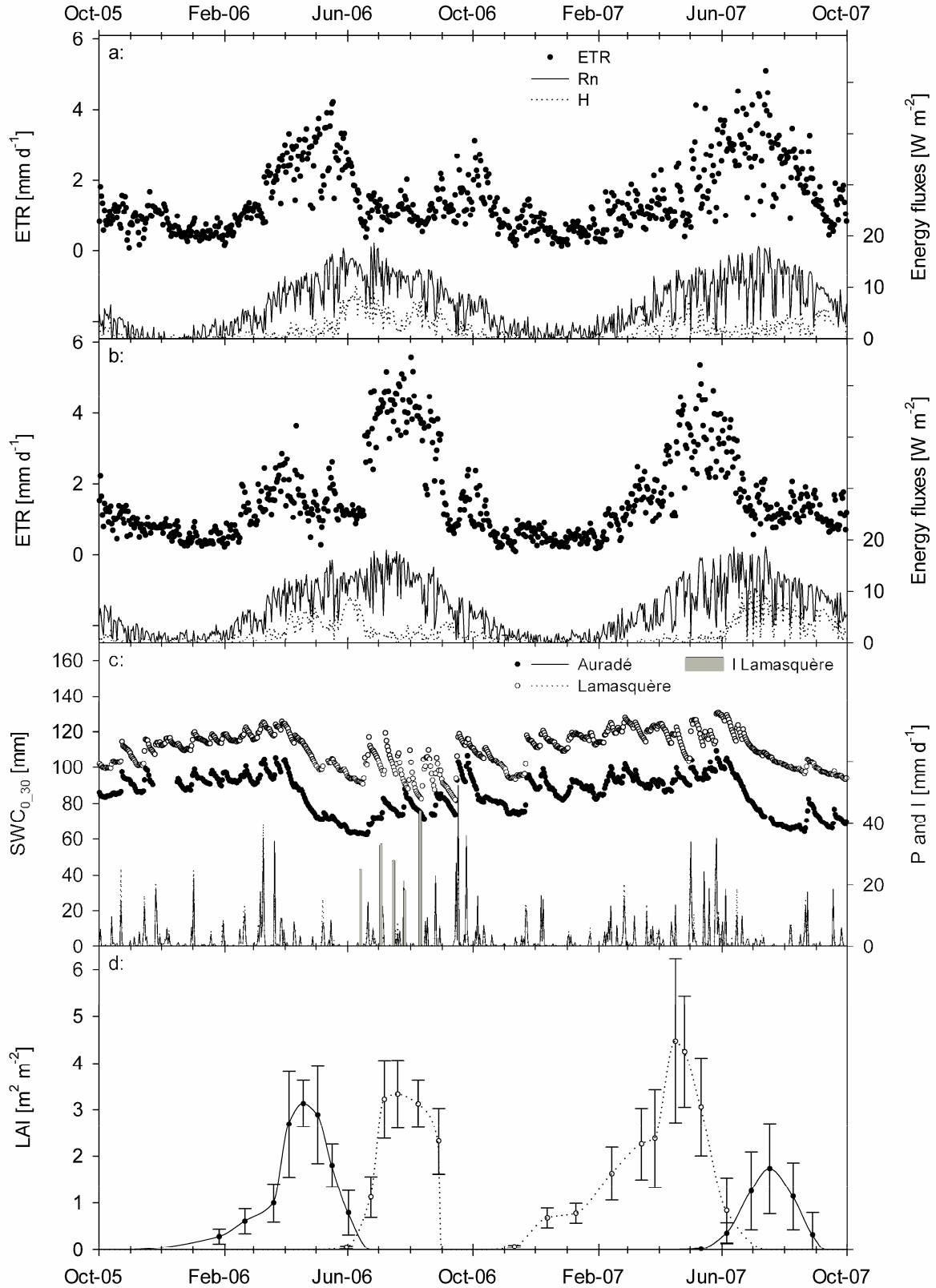
Figure 2: Seasonal dynamics of daily evapotranspiration (ETR), net radiation ( R_n ) and sensible heat flux ( H ) at Auradé (a) and Lamasquère (b), daily soil water content between 0 and 0.3 m depth ( SWC_{0-30} , open and full circles), daily precipitation and Lamasquère irrigation ( P , solid and dotted lines and I , grey bars, respectively) (c) and measured leaf area index (LAI, open and full circles) and interpolated LAI (solid and dotted lines) (d), from October 2005 to October 2007. In d, error bars correspond to \pm one standard deviation of the mean.
