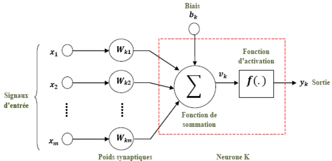
Figure 3.18. Neurone formel
