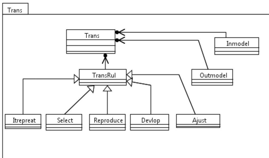
Figure 6.24. Description du Package Trans
