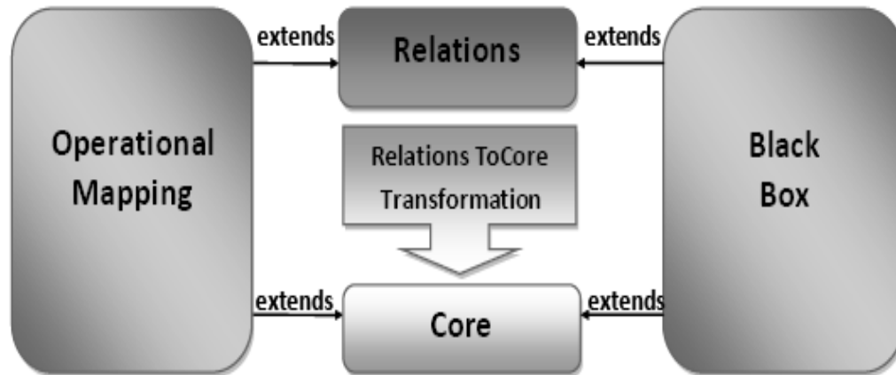
Figure 4.10. Architecture de QVT
