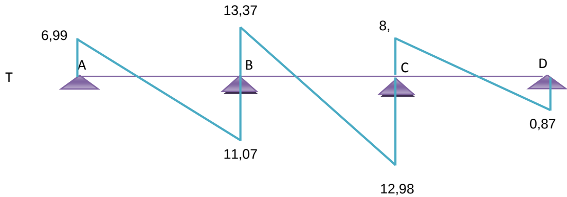
Figure III.4 Diagramme des efforts tranchants
