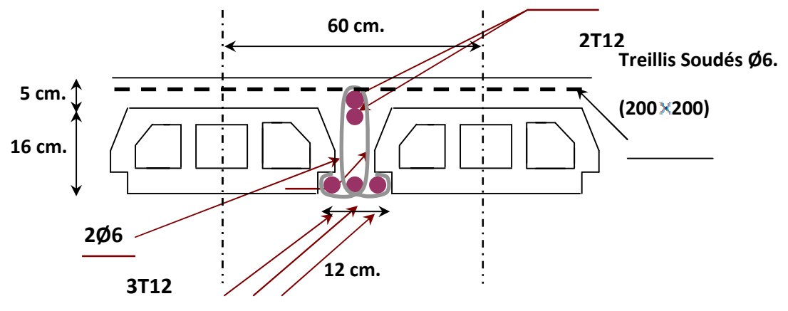
Figure III.14 ferrailage de poutrelle
