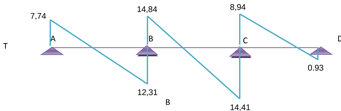
Figure III.6 Diagramme des efforts tranchants
