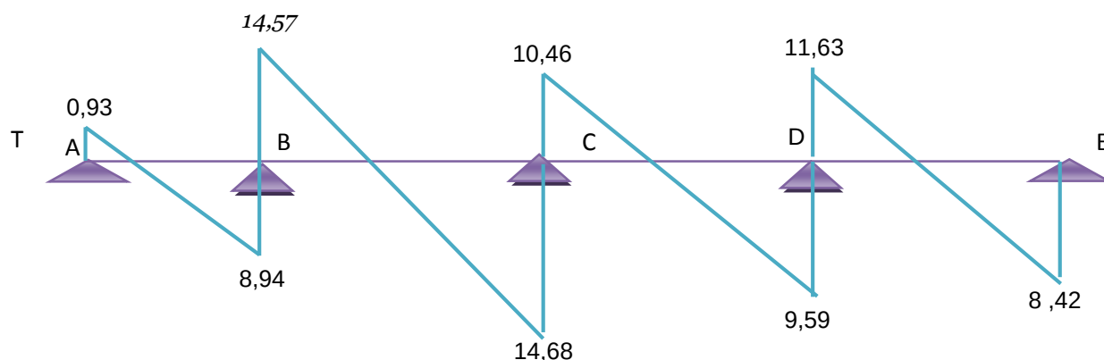
Figure III.11 Diagramme des efforts tranchants
