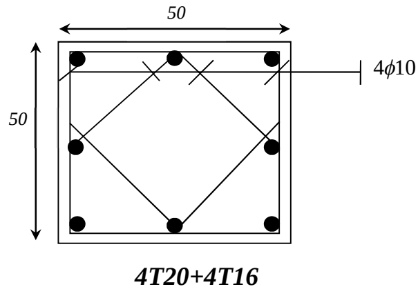
Figure.VI.2 Ferrailage des poteaux
