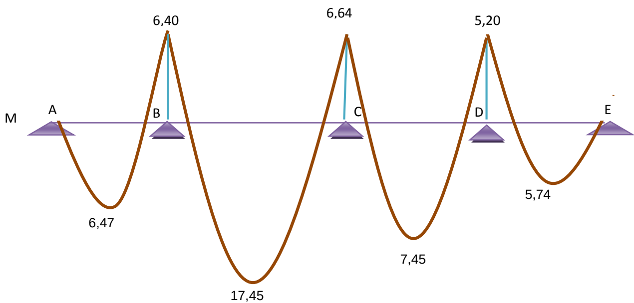
Figure III.10 Diagramme des moments fléchissants, M [KN.m]
