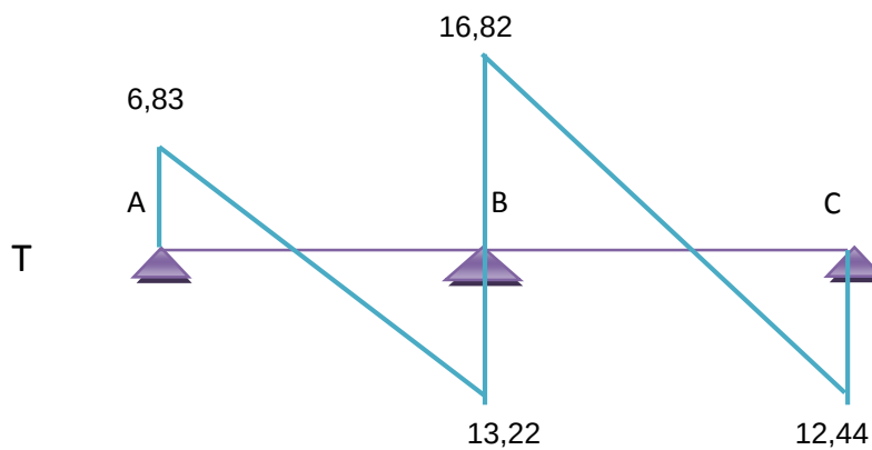
Figure III.9 Diagramme des efforts tranchants
