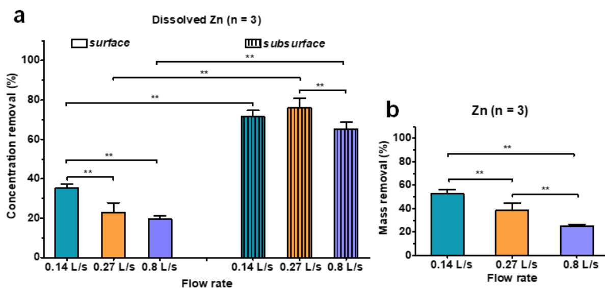
Figure 0.12 (Figure S11). Effect of flow-rate on the removal efficiency of Zn for the standard swale. a Concentration removal. b Mass removal. Significant differences are shown with ** ( p < 0.05 ), bars indicate standard deviation
