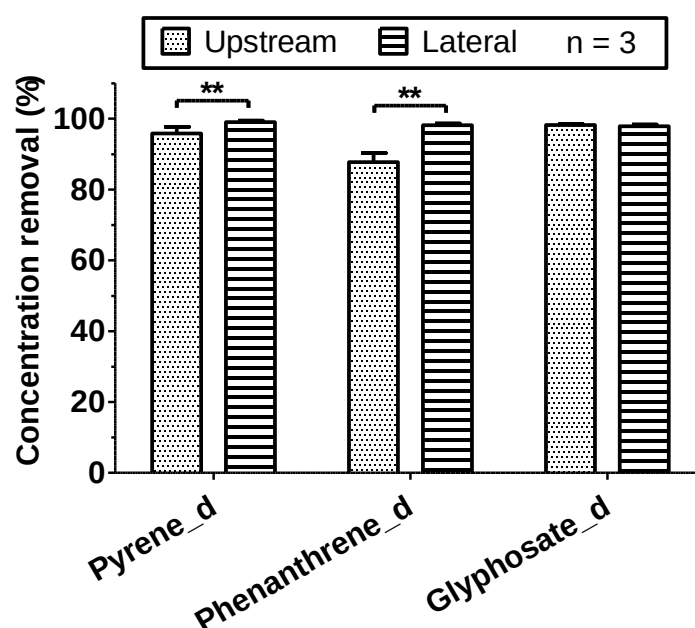
Figure 0.11 (Figure S10). Concentration reductions for dissolved pyrene, dissolved phenanthrene and dissolved glyphosate (filtering swale, inflow flow-rate = 0.27 L/s). Significant differences are shown with ** ( p < 0.05 ), bars indicate standard deviation
