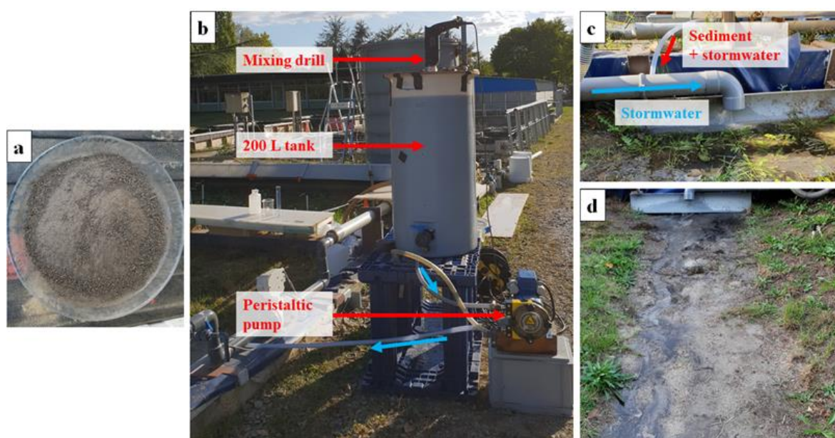
Figure 0.7 (Figure S6). TSS spiking system. a Photograph of the 561 g dried sediment added in the 200 L polyethylene tank. b Photograph (overview) of the TSS spiking system during a test: TSS solution was continuously stirred by a mixing drill and a peristaltic pump (69 L/h) was used to feed the swale. c TSS solution was diluted in stormwater incoming from the 7 m 3 tank. d Photograph of the upstream flows spiked with TSS, pyrene, phenanthrene and glyphosate (filtering swale)
