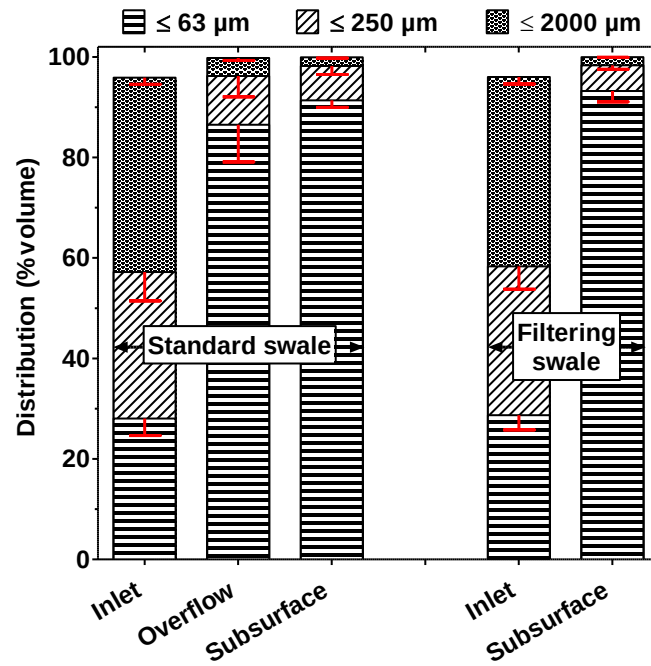
Figure 0.18 (Figure S17). Evolution of the distributions of 3 particle size classes ( \leq 63 \mu\text{m} , \leq 250 \mu\text{m} and \leq 2000 \mu\text{m} ) in both swale inflows and outflows (red error bars show the standard deviations, n = 3 test events for the filtering swale, n = 2 test events for the standard swale, analyses on each water sample were performed 3 times)
