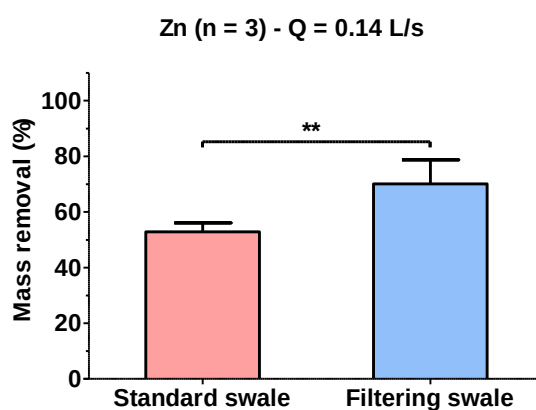
Figure 0.14 (Figure S13). Mass removal of Zn for the standard swale and the filtering swale (0.14 L/s events).
