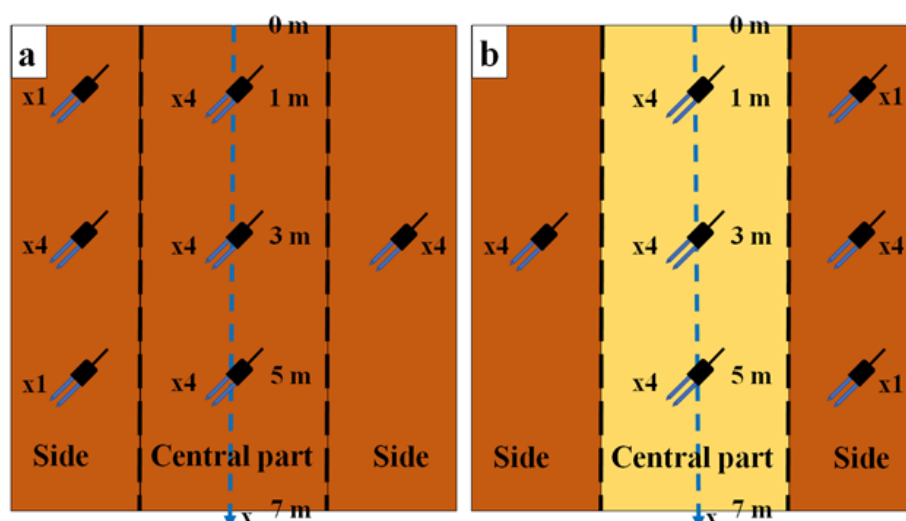
Figure 0.8 (Figure S7). Location of the soil moisture sensors in the pilot swales (plan view). a standard swale. b filtering swale
