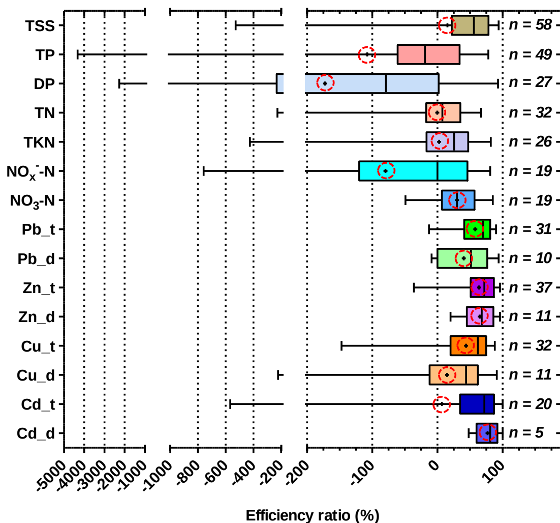
Figure 2.3 (Figure 3). Range of ER values for pollutants from the database. Boxplots were used to display data spread (see Figure 2b for the legend of a boxplot)
