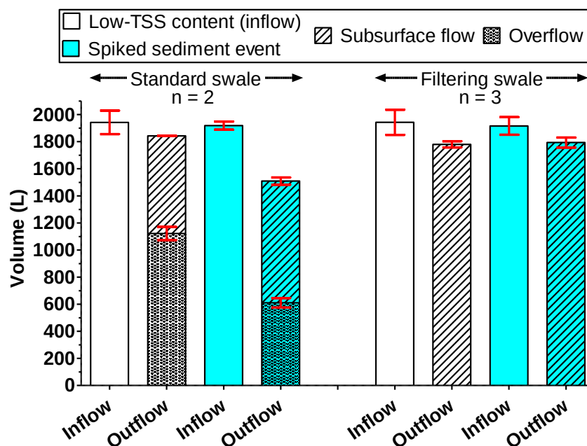
Figure 0.19 (Figure S18). Water balances found under RRMS conditions. Red error bars indicate the standard deviations
