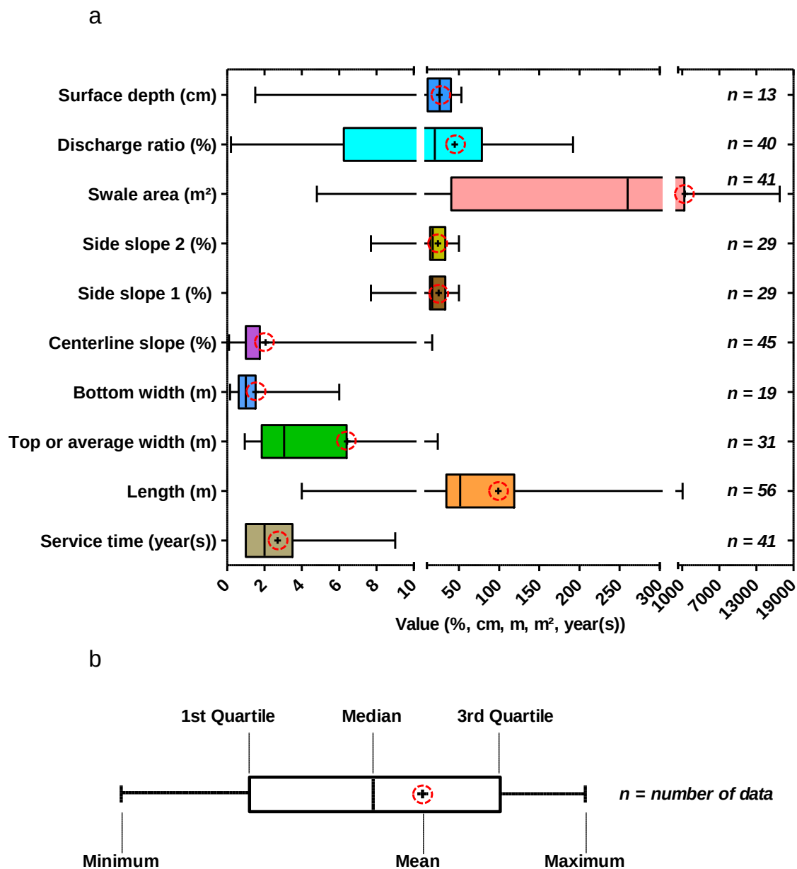
Figure 2.2 (Figure 2). Design characteristics of swales registered in the database. a Boxplots for the design factors characterizing swale database. b Legend for boxplots
