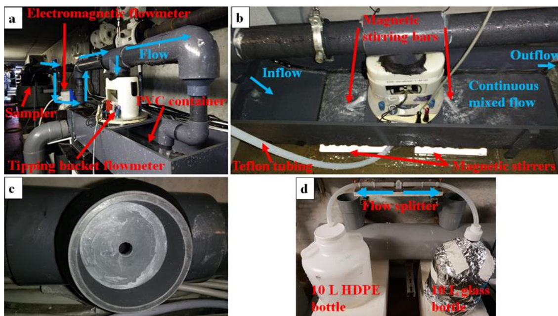
Figure 0.6 (Figure S5). Specific facility designed to measure effluent flow-rates and to collect composite water samples. a Photograph of the facility. b Photograph of the PVC container continuously supplied with swale outflows. c Photograph of the aperture (diameter = 8 mm) in the PVC pipe connected to the tipping bucket flowmeter; this restricts the maximum flow-rates discharged into the bucket. d Photograph of the water sampling system; flows are equally split downstream the automatic sampler between a 10 L HDPE bottle and a 10 L glass bottle
