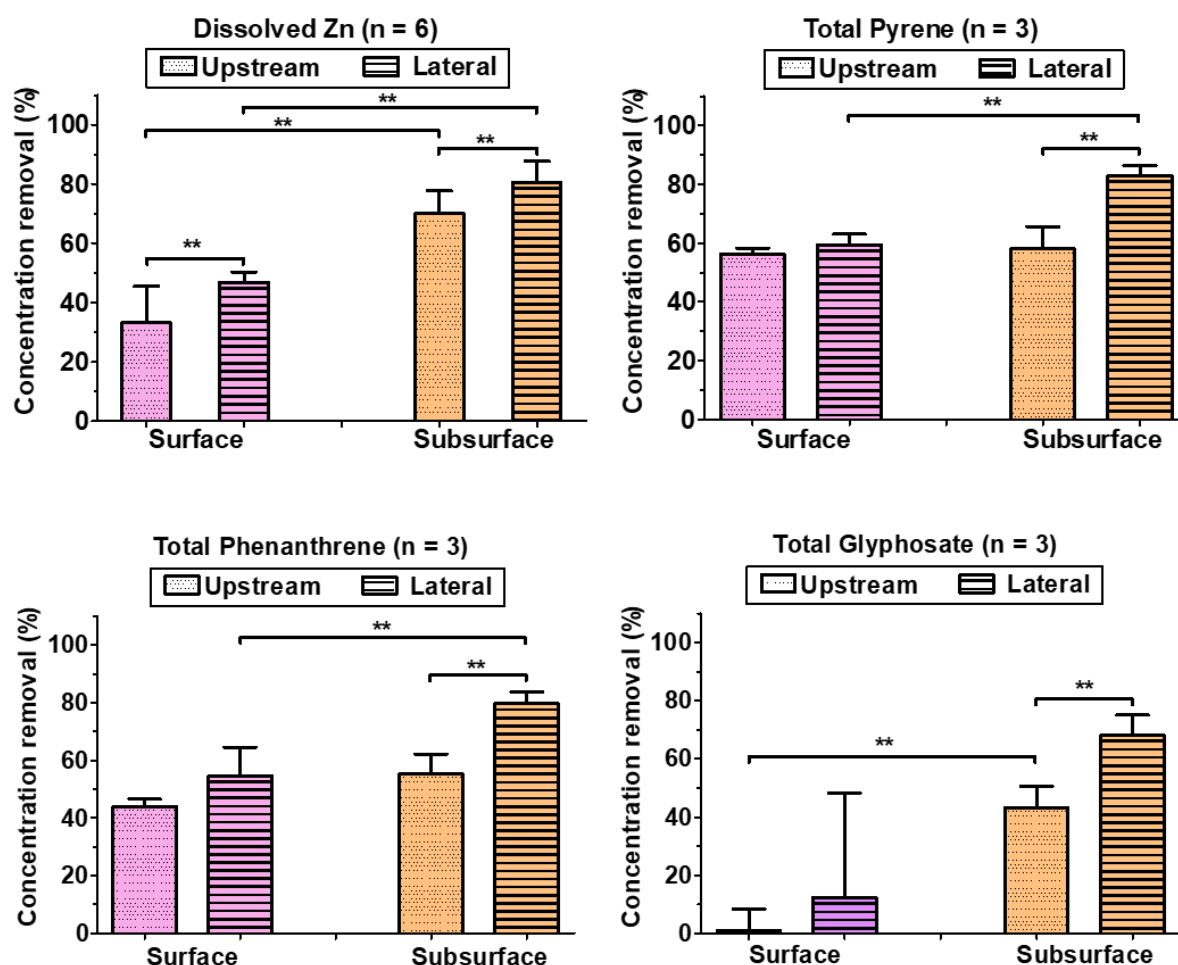
Figure 5.2 (Fig. 2). Removal efficiencies (in concentration) of dissolved Zn, total pyrene, total phenanthrene and total glyphosate by the standard swale (0.27 L/s inflows). Removal efficiencies were separately calculated for overflows (surface outlet) and for subsurface outflows (subsurface outlet). Uncertainty bands represent +standard deviation. Significant statistical differences are shown with ** ( p < 0.05 )
