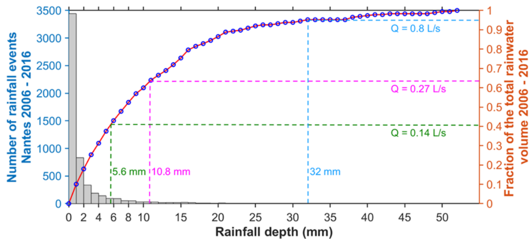
Figure 0.2 (Figure S1). Runoff depths of pilot test events, histogram of the rainfall depths recorded in Nantes during the period 2006 - 2016, and contribution to the total rainwater volume (red curve)
