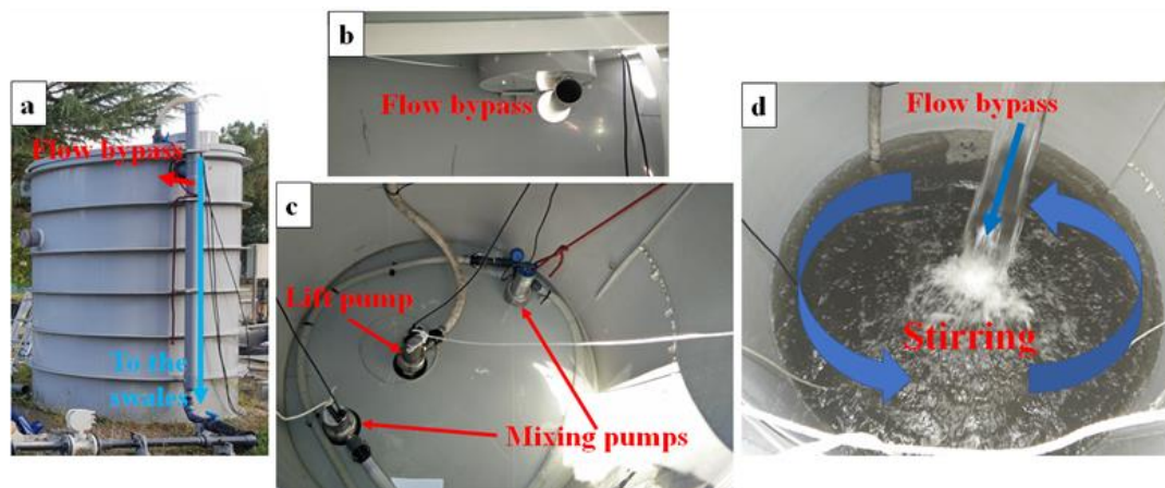
Figure 0.3 (Figure S2). Stormwater tank of 7 m 3 equipped with pumps and a flow bypass to ensure thorough mixing. a Photograph of the PVC tank. b Photograph of the bypass pipe (inside the tank). c Photograph of the pumps. d Photograph of the stormwater stirred by both the pumps and the backflow from the bypass pipe
