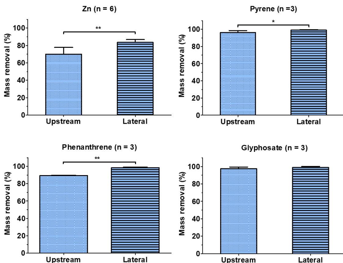
Figure 5.5 (Fig. 5). Removal efficiencies (in mass) of Zn, pyrene, phenanthrene and glyphosate by the filtering swale (0.27 L/s inflows). Uncertainty bands represent +standard deviation. Significant statistical differences are shown with * ( p < 0.1 ) and ** ( p < 0.05 )
