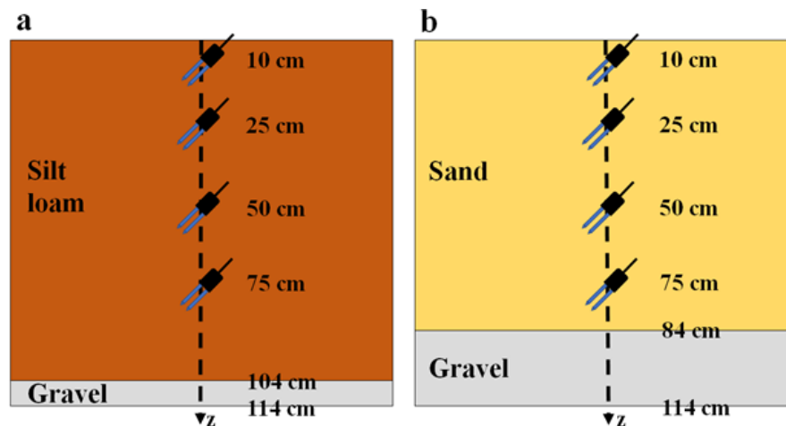
Figure 0.9 (Figure S8). Location of the soil moisture sensors in the central parts of the pilot swales (side view). a standard swale. b filtering swale
