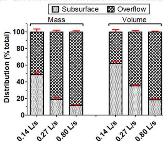
Figure 0.16 (Figure S15). Effect of flow-rate on the distributions of the discharged Zn mass and the discharged volume between overflows and subsurface outflows (standard swale); results are found for 0.14 L/s ( n = 3 ), 0.27 L/s ( n = 3 ) and 0.8 L/s ( n = 3 ) upstream inflows. Red error bars show the standard deviations
