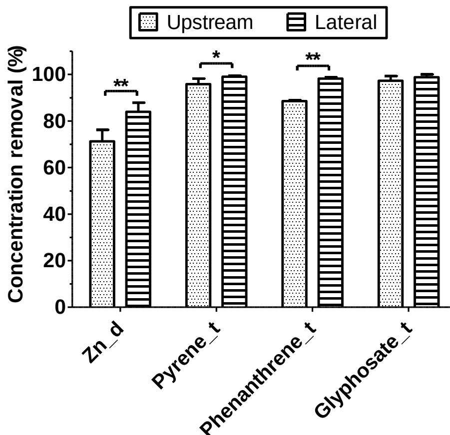
Figure 5.4 (Fig. 4). Removal efficiencies (in concentration) of dissolved Zn (Zn_d), total pyrene (Pyrene_t), total phenanthrene (Phenanthrene_t) and total glyphosate (Glyphosate_t) by the filtering swale (0.27 L/s inflows). Uncertainty bands represent +standard deviation. Significant statistical differences are shown with * ( p < 0.1 ) and ** ( p < 0.05 )
