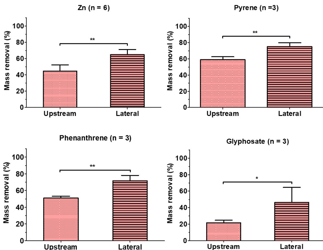
Figure 5.3 (Fig. 3). Removal efficiencies (in mass) of Zn, pyrene, phenanthrene and glyphosate by the standard swale (0.27 L/s inflows). Uncertainty bands represent +standard deviation. Significant statistical differences are shown with * ( p < 0.1 ) and ** ( p < 0.05 )
