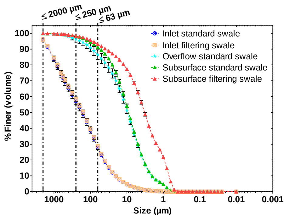
Figure 0.17 (Figure S16). Particle size distributions of swale inflows and outflows (bar represents standard deviation, n = 3 test events for the filtering swale, n = 2 test events for the standard swale, analyses on each water sample were performed 3 times)
