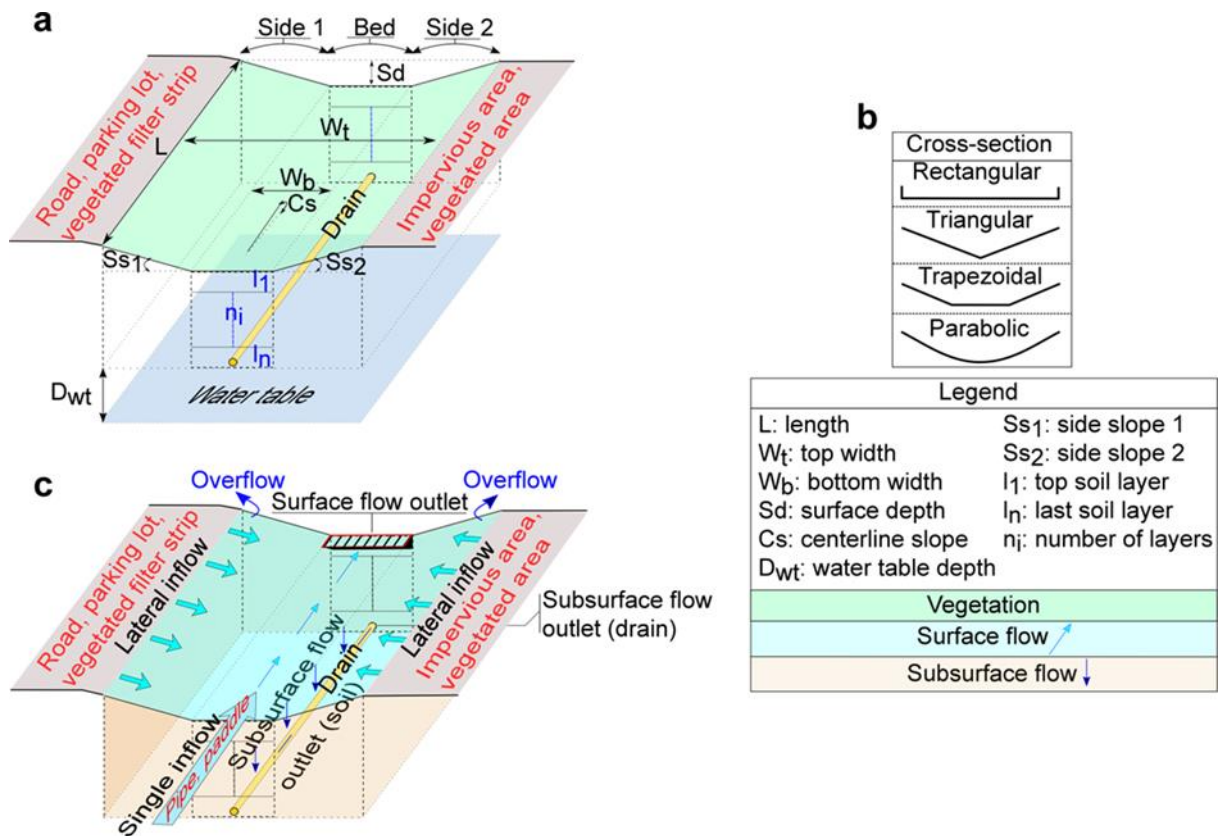
Figure 0.1 (Figure S1). Descriptive schemes introducing a. swale design characteristics, b. range of cross-section shapes and c. swale distribution of flows
