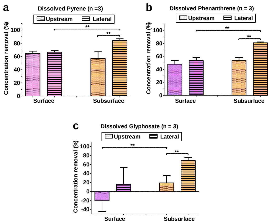
Figure 0.10 (Figure S9). Concentration reductions for dissolved pyrene, dissolved phenanthrene and dissolved glyphosate (standard swale, inflow flow-rate = 0.27 L/s). Significant differences are shown with ** ( p < 0.05 ), bars indicate standard deviations
