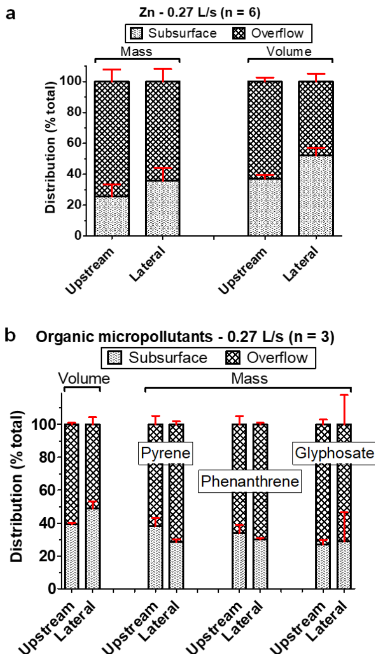
Figure 0.15 (Figure S14). Distributions of the discharged mass and the discharged volume between overflows and subsurface outflows (standard swale); results are found for 0.27 L/s upstream inflows (n = 3 or n = 6) and 0.27 L/s lateral inflows (n = 3 or n = 6). a Zinc. b Pyrene, Phenanthrene and Glyphosate. Red error bars show the standard deviations
