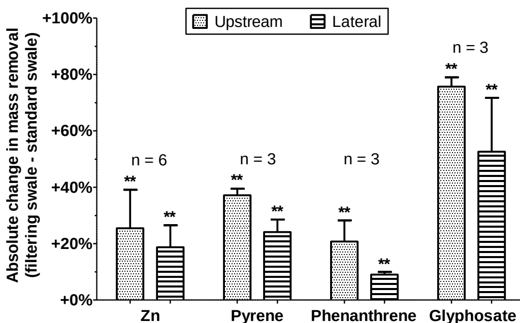
Figure 5.6 (Fig. 6). Pollutant removal efficiency gains for the filtering swale compared to the standard swale. Uncertainty bands represent +standard deviation. Significant statistical differences are shown with * ( p < 0.1 ) and ** ( p < 0.05 )
