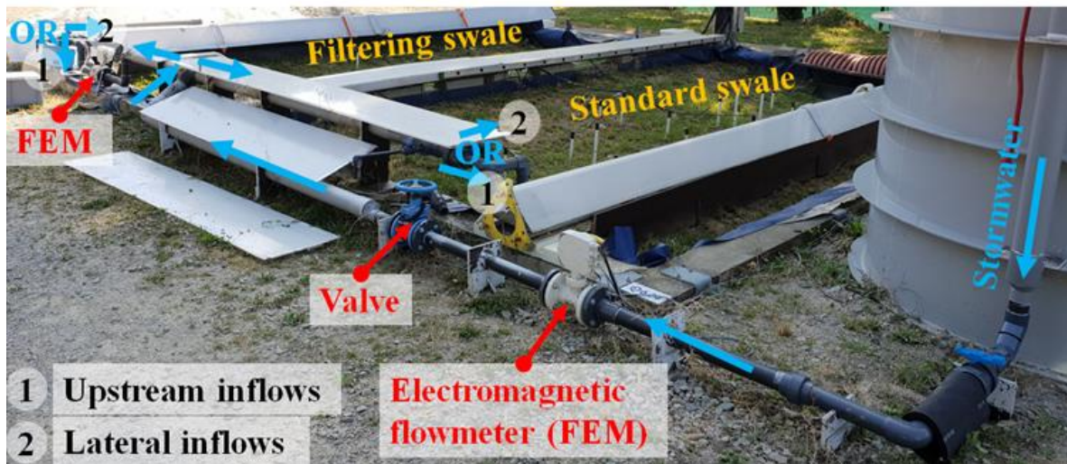
Figure 0.4 (Figure S3). Photograph of the piping system designed to supply the pilot with artificial runoff events
