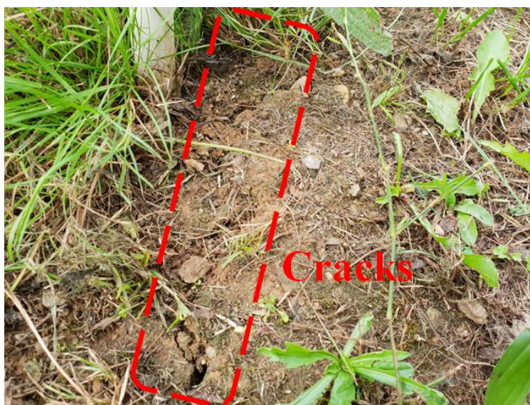
Figure 0.20 (Figure S19). Photograph of cracks in the standard swale
