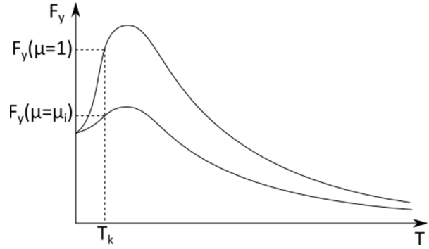
Figure A.3: Reduction factor
