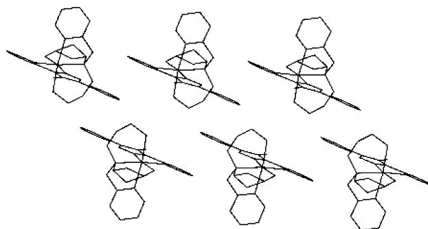
Figure 3. View of [\text{Fe}(\text{DAPP})(\text{abpt})](\text{ClO}_4)_2 showing the \pi stacking interactions at 293 K.
