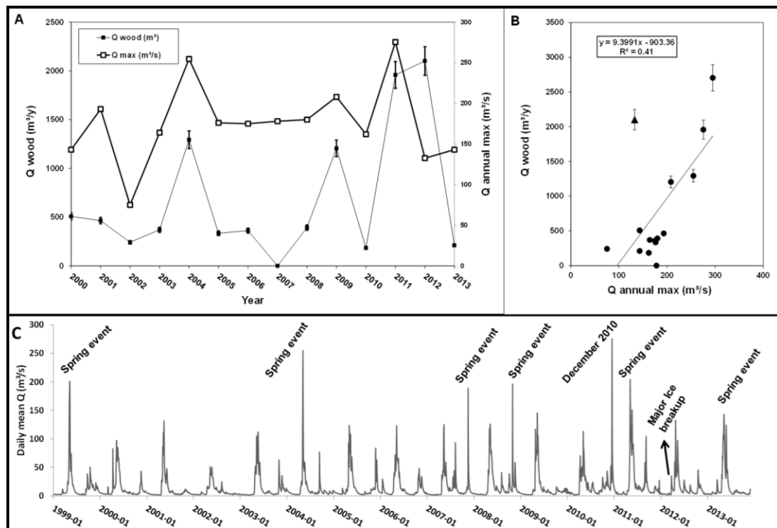
Figure 21. (A) Relationship between river discharge ( Q_{max} ( m^3/s )) and LW discharge ( Q_{wood} ( m^3 )) in the Saint-Jean River over time; (B) the scatter plot of the flow. (Triangle symbol indicates an important ice breakup event in 2012); and (C) flood series between 1999 and 2013.
