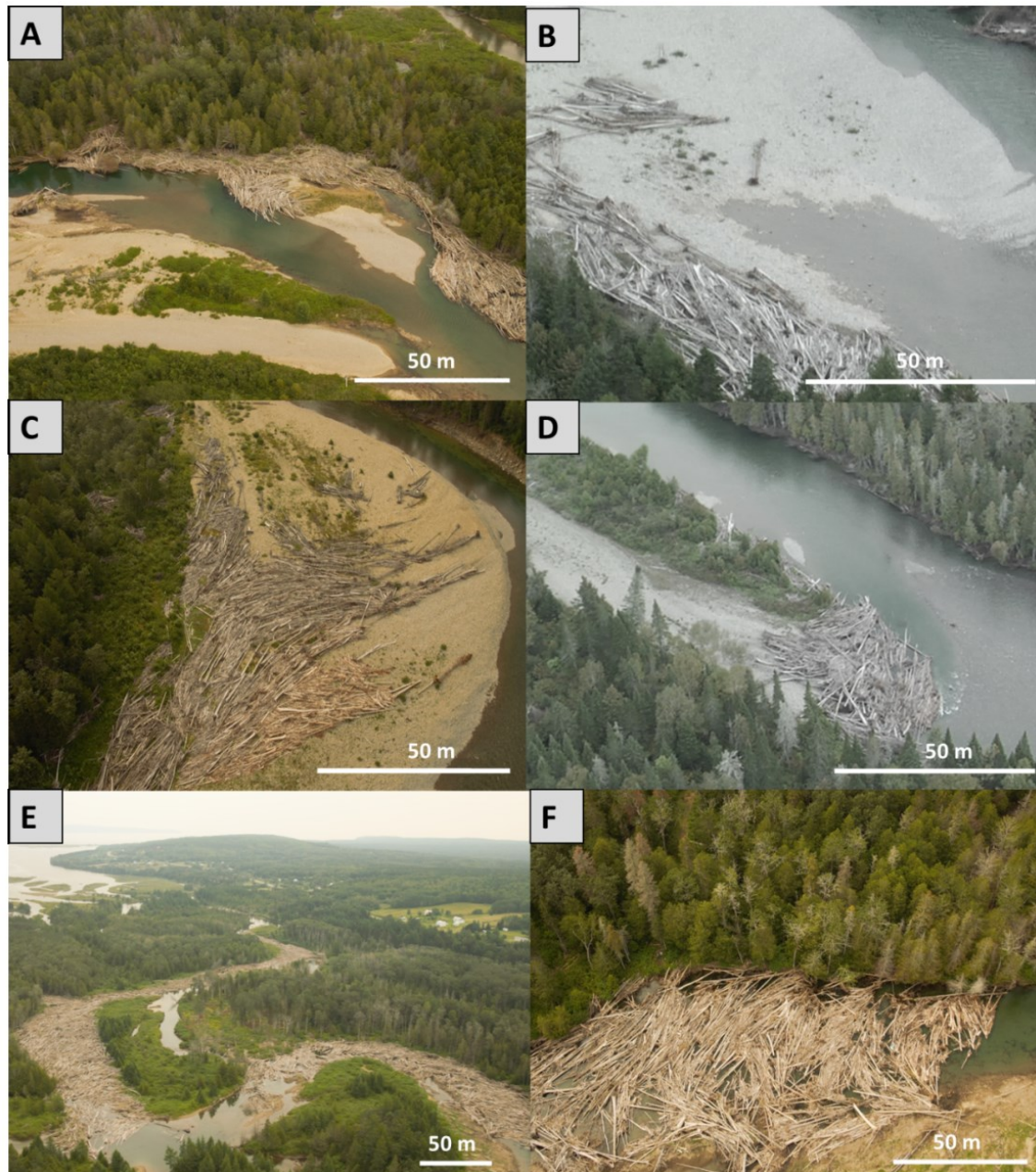
Figure 25. Large wood jam accumulations in the SJR corridor. (A) Meander jams, (B) secondary channel jams, (C) bank deposit jams, (D) bar apex jams, (E) oblique view of south channel raft, and (F) aerial view of large jam rafts in the upstream part of the SJR delta.
