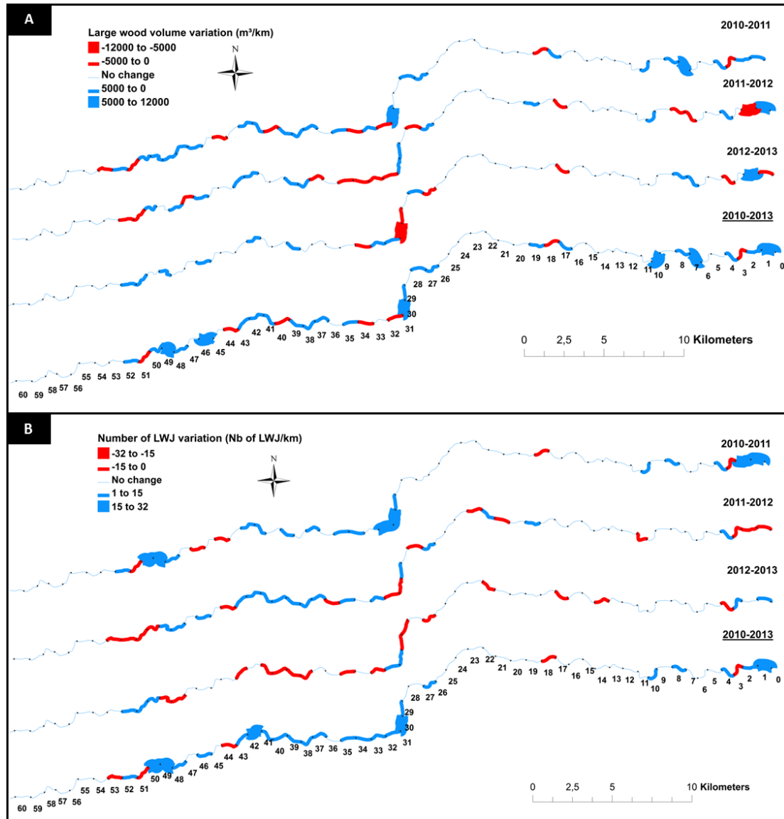
Figure 32. Spatiotemporal variability between each year of the survey (2010–2013) of (A) LWJ volume ( \text{m}^3 ) per kilometre and (B) number of LWJ per kilometre.
