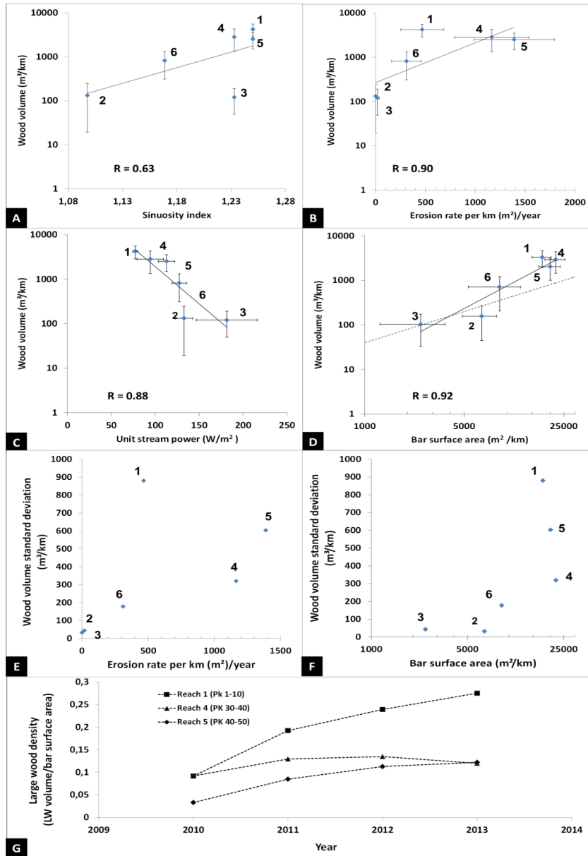
Figure 35. Geomorphological relationship between sinuosity (A), erosion rate (B and E), unit stream power (C), and bar surface area (D and F) on LWJ dynamics for the six 10 km reaches (indicated by numbers) of the SJR fluvial corridor: 1 = 0-10 km, 2 = 10-20 km, 3 = 20-30 km, 4 = 30-40 km, 5 = 40-50 km, 6 = 50-60 km. (G) LW density over the four years for reaches with the highest LW volumes and bar surface areas. Error bars represent the 95% confidence interval for each river reach, the dashed line in (D) represents a homogeneous LW density by bar surface area with a ratio of 1 \text{ m}^3 per 25 \text{ m}^2 and E and F represents the LW volume standard deviation between the four-year surveys.
