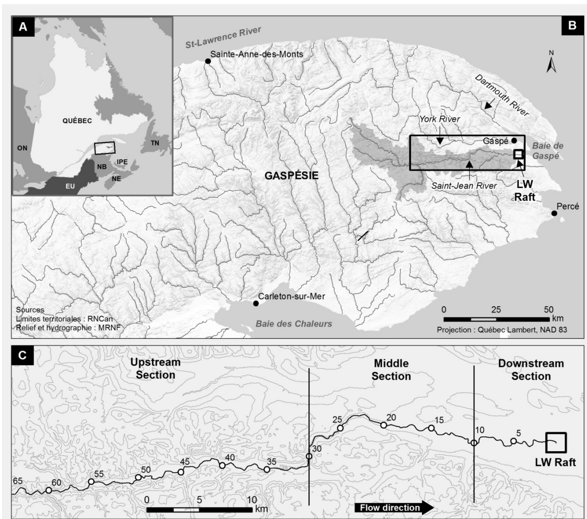
Figure 24. (A) Map showing the location of the Saint-Jean River in Québec, Canada. (B) Location of the Saint-Jean River on the Gaspé Peninsula. (C) Detailed map showing the studied river corridor with distances from the river mouth (in km).
