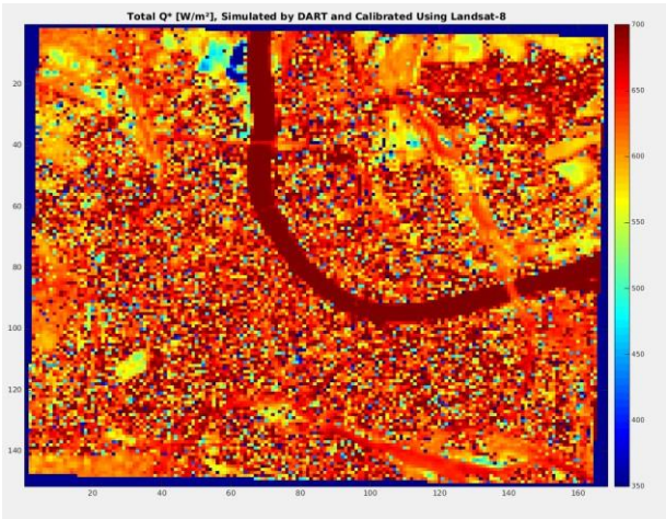
Fig. 4 Total radiative budget (W/m2) over the city of Basel as modeled by DART.
