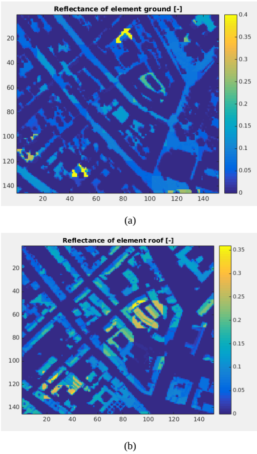
Fig. 3 High resolution (metric) reflectance image derived from a LandSAT-8 image (864.6nm, 30m)
