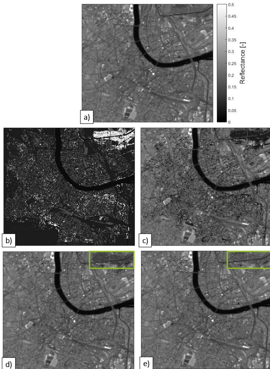
Figure 4.32 : Calibration it rative de DART. (a) Image Sentinel-2 du 24.06.2016 (B8a-865nm)   20m de r solution. (b) Image de r flectance simul e DART sans calibration   20m de r solution. (c) Image DART apr s 1 it ration (d) 2 it rations (e) 3 it rations.
